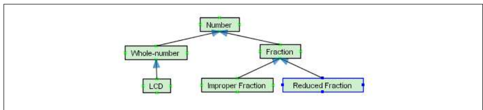
Figure 5.11: Ontology for the Domain of Adding Two Fractions
