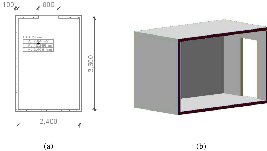
Figure 4. ISO 9705 test room (a) plan elevation, (b) cut-through isometric view.
