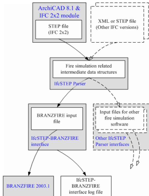
Figure 3. IfcSTEP Parser data exchange process (dotted items not currently implemented).
