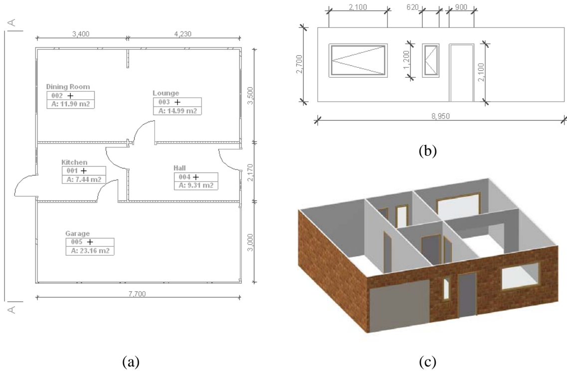
Figure 6. Ground floor of the two-storey residential building (a) plan elevation, (b) end elevation, section A-A, (c) isometric view.
