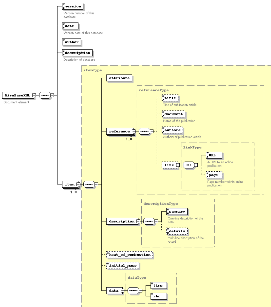
Figure 2. An overview of the FireBaseXML schema. Optional elements are shown by boxes drawn with dotted lines.
