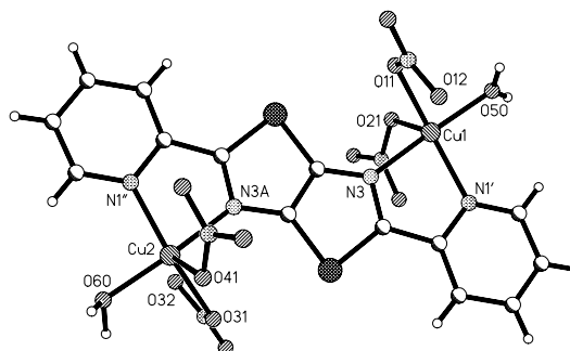
Fig. 3 The X-ray crystal structure of 6 . Selected bond distances (Å) and angles ( o ): Cu1-N3 2.047(4), Cu1-N1' 2.098(4), Cu1-O11 2.101(3), Cu1-O21 2.295(4), Cu1-O50 1.989(4), N3-Cu1-O50 172.92(19), N3-Cu1-N1' 81.13(16), N1'-Cu1-O50 96.39(17), O11-Cu1-O50 89.50(16), N3-Cu1-O11 89.90(15), N1'-Cu1-O11 153.61(15), O50-Cu1-O21 95.75(18), N3-Cu1-O21 91.32(15), N1'-Cu1-O21 114.03(15), O11-Cu1-O21 90.80(14), Cu2-N3A 2.047(4), Cu2-N1'' 2.087(4), Cu2-O31 2.120(3), Cu2-O41 2.286(4), Cu2-O60 1.995(4), N3A-Cu2-O60 172.39(19), N3A-Cu2-N1'' 80.80(16), N1''-Cu2-O60 95.52(18), O31-Cu2-O60 90.62(16), N3A-Cu2-O31 90.04(15), N1''-Cu2-O31 154.82(14), O60-Cu2-O41 97.79(19), N3A-Cu2-O41 89.80(16), N1''-Cu2-O41 114.29(17), O31-Cu2-O41 88.90(15).
