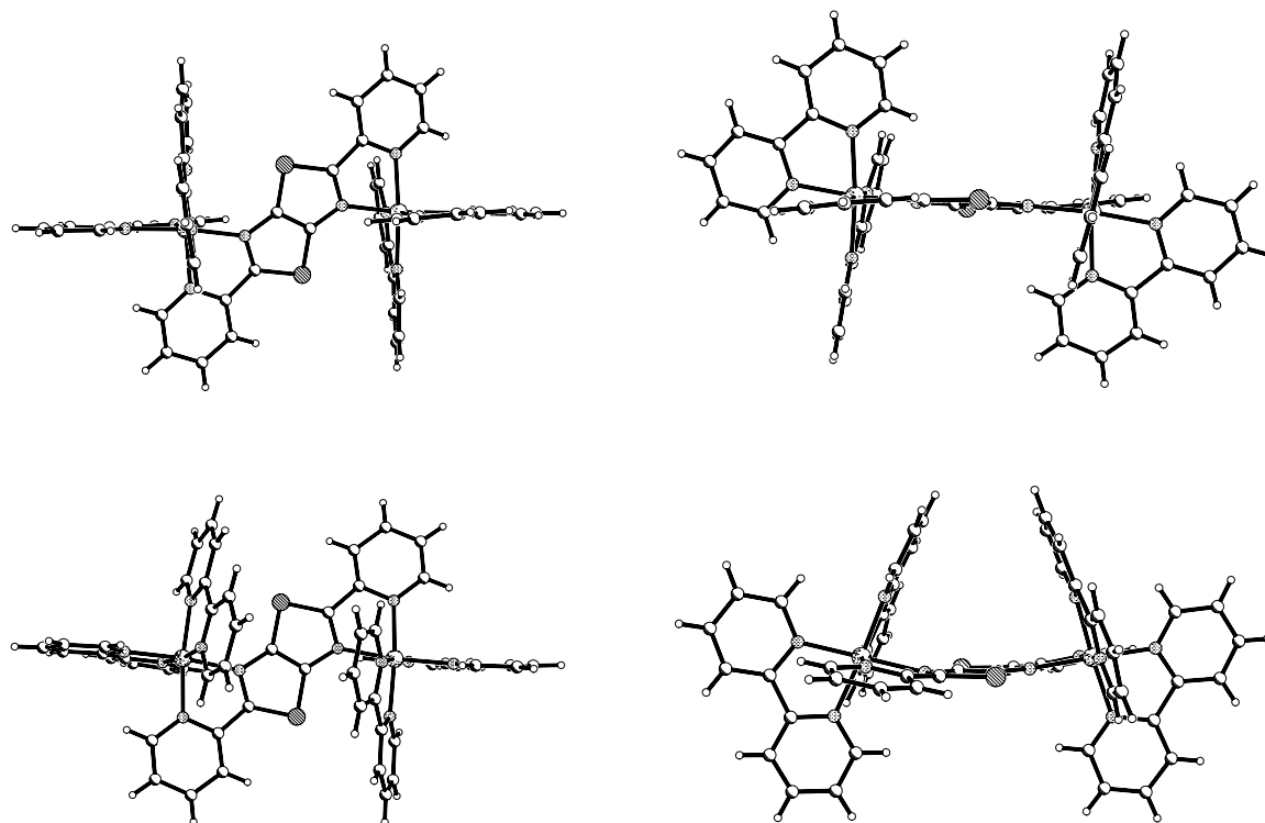
Fig. 5 Two perspective views of the X-ray structures of 7meso (top) and 7rac (bottom), emphasizing the very different shapes of these two diastereoisomeric cations. Hexafluorophosphate counterions and acetonitrile solvate molecules are omitted for clarity. The Ru-N bond lengths lie in the relatively narrow range of 2.031(7)-2.086(7) Å, with the longest bond in each case being to the pyridine nitrogen of the bridging ligand. The cis -disposed bond angles lie in the range 77.6(3)-100.8(3)°, with the smallest angles being within the chelate rings. The trans -disposed bond angles are in the range 170.7(1)-175.2(1)°.
