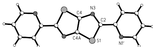
Fig. 2 The X-ray crystal structure of 5 . Selected bond distances (Å) and angles ( o ): S1-C2 1.757(2), S1-C4A 1.730(2), C2-N3 1.316(2), C2-C2' 1.472(2), N3-C4 1.367(2), C4-C4A 1.384(3), C4A-S1-C2 87.90(8), S1-C2-N3 116.95(14), C2-N3-C4 107.92(15), N3-C4-C4A 117.9(2), S1-C4A-C4 109.33(18).
