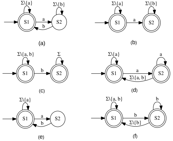
Fig. 7: Translations of LTL expressions to FSAs: (a) a is always followed by b , (b) a is never followed by b , (c) a is always preceded by b , (d) a is never immediately followed by b , (e) a is always immediately followed by b , (f) a is always immediately preceded by b .
