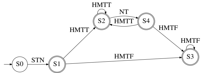
Fig. 4: StringTokenizer’s Ground Truth Model. “STN”: StringTokenizer(). “HMTT”: hasMoreTokens() = true. “HMTF”: hasMoreTokens() = false. “NT”: nextToken().
