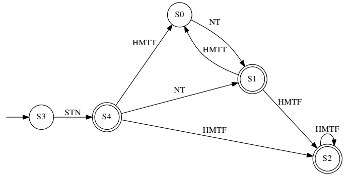
Fig. 3: StringTokenizer’s SpecForge Model. “STN”: StringTokenizer(). “HMTT”: hasMoreTokens() = true. “HMTF”: hasMoreTokens() = false. “NT”: nextToken().
