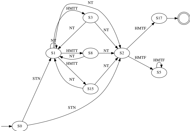
Fig. 2: StringTokenizer’s CONTRACTOR++ Model. “STN”: StringTokenizer(). “HMTT”: hasMoreTokens() = true. “HMTF”: hasMoreTokens() = false. “NT”: nextToken().
