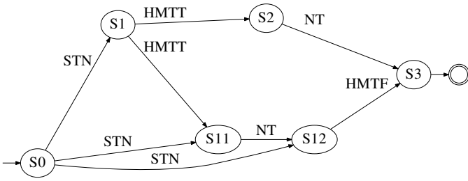
Fig. 1: StringTokenizer’s Traditional 2-tail Model. “STN”: StringTokenizer(). “HMTT”: hasMoreTokens() = true. “HMTF”: hasMoreTokens() = false. “NT”: nextToken().
