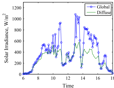
(b) “Cloudy” scenario solar irradiance
