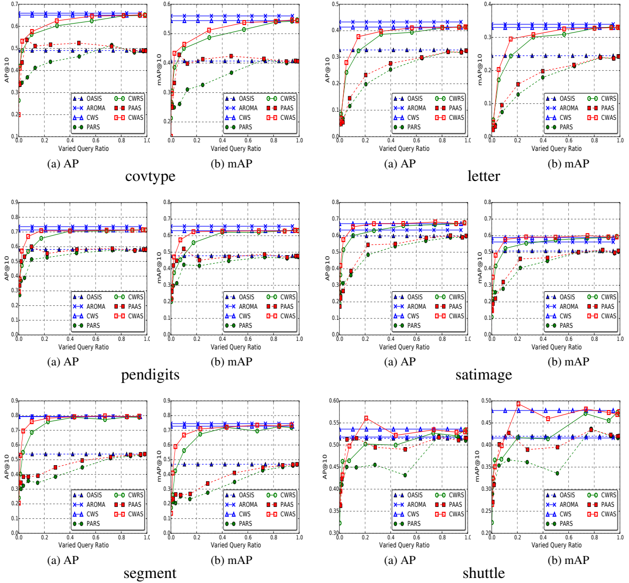
Figure 1: Performance with varied query ratios on the test datasets, where AP@10 denotes Average Precision at 10, and mAP@10 denotes mean Average Precision at 10.
