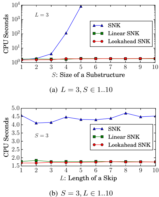
Figure 6: Efficiency: SNK vs. approximations
