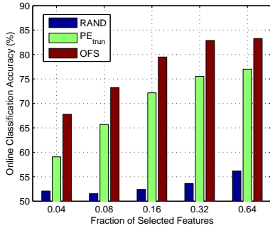
(a) splice
