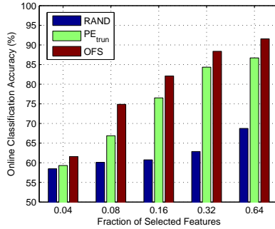
(b) spambase
