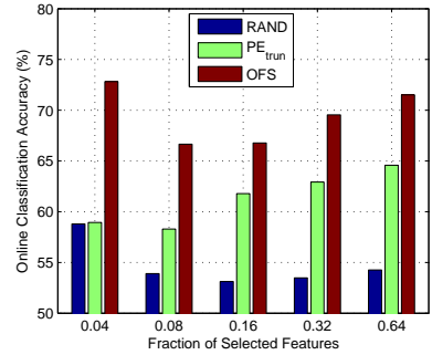
(c) svmguide3
