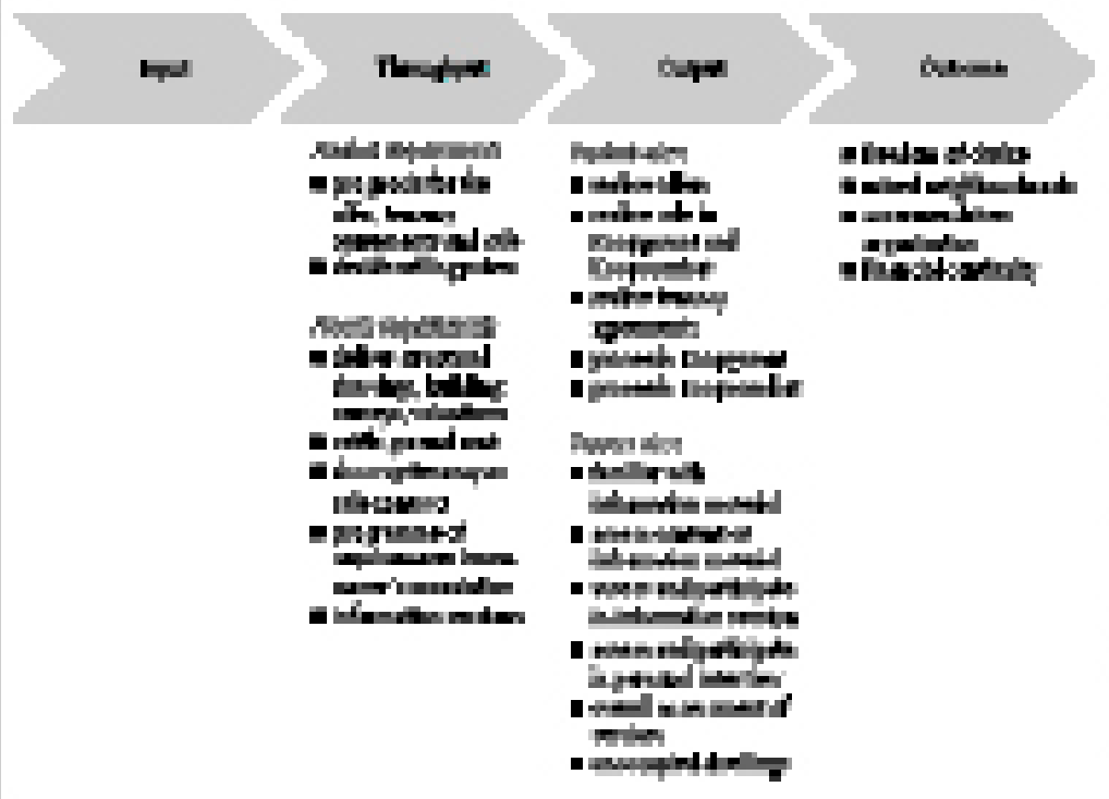
Figure 7.3 Input-output-outcome model
