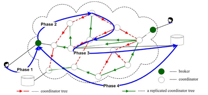
Fig. 7. We explain the query brokering process in four phases.
