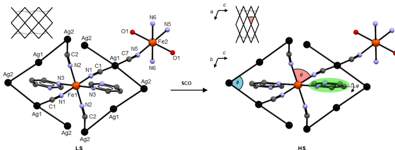
Figure 2. Fragment of FeAg viewed along the a -axis in the LS (left) and HS state (right) with zig-zag Ag1-Ag2-Ag1 angle, \phi (blue), pyrimidine ligand twist angle, \varphi , and the N2-Fe1-N1 wine-rack hinge angle, \theta (red) labelled. H-atoms are removed for clarity. Top left inset shows the wine-rack topology viewed along the b -axis in each spin-state, with the silver chains (grey) and hinge angle (red) highlighted. Contraction of the framework is exaggerated for clarity.
