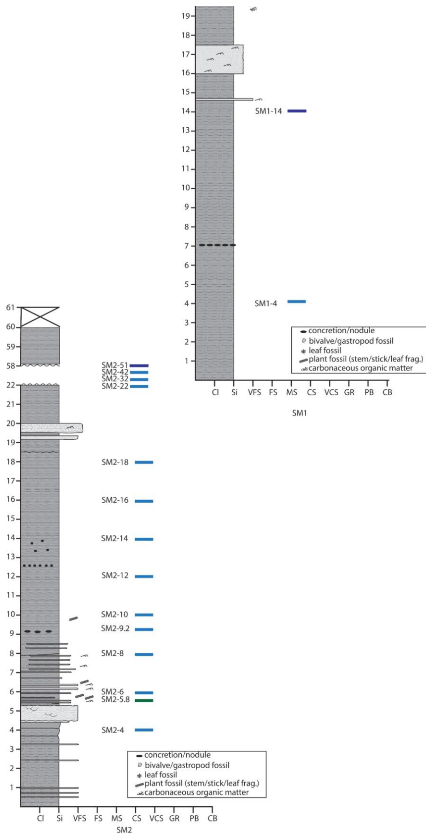
Figure 11 bottom – The changes in \delta^{13}\text{C} values is shown in comparison to the stratigraphy for the first 25m of measured section SM2. Cl = clay, Si = silt, VF = very fine sand. This area showed the most nuanced variation with certain stratigraphic position.
