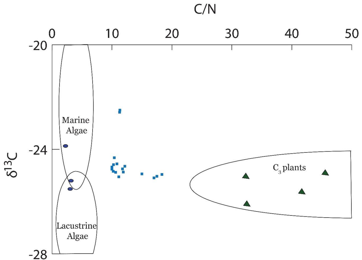
Figure 13 – The relationship between \delta^{13}\text{C} values and C/N ratios indicates areas produced by marine algae, lacustrine algae, and \text{C}_3 land plants (after Meyers, 1997). Most of the sample is a combination of algae and plant material, as shown by the blue squares, suggesting a mix source of both marine and terrestrial material. The green triangles encompassed by the half oval represent \text{C}_3 land plants. And the dark blue ovals represent algae, the upper oval is marine algae, while the other oval indicates lacustrine algae.
