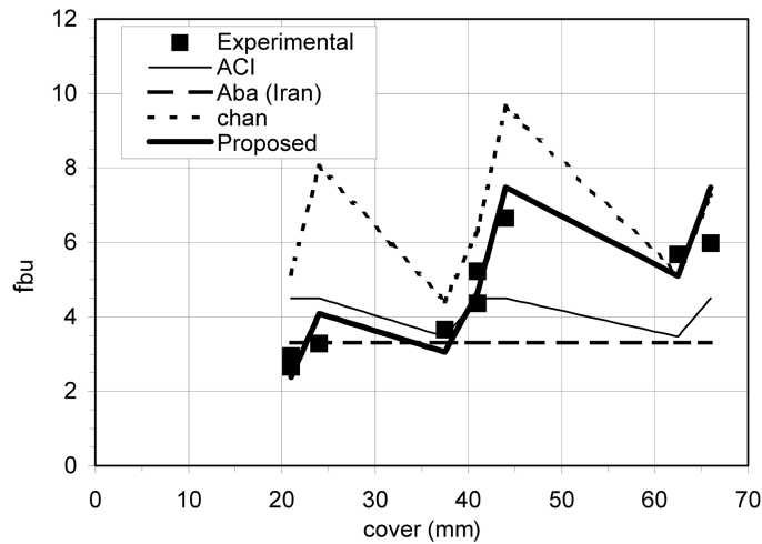
(b) Concrete cover versus ultimate bond strength
