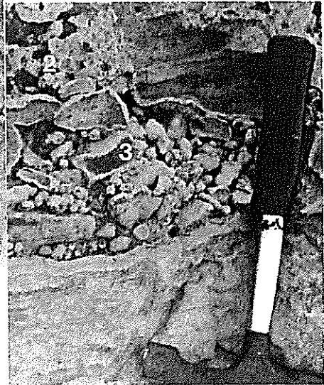
Fig. 7b. Left. Laminar caliche (1) and vadosic pisolites (2) in the beach facies, near Section C. Right. Paleosol breccias (3) and vadosic pisolites (2) in the beach facies, near Section C.
