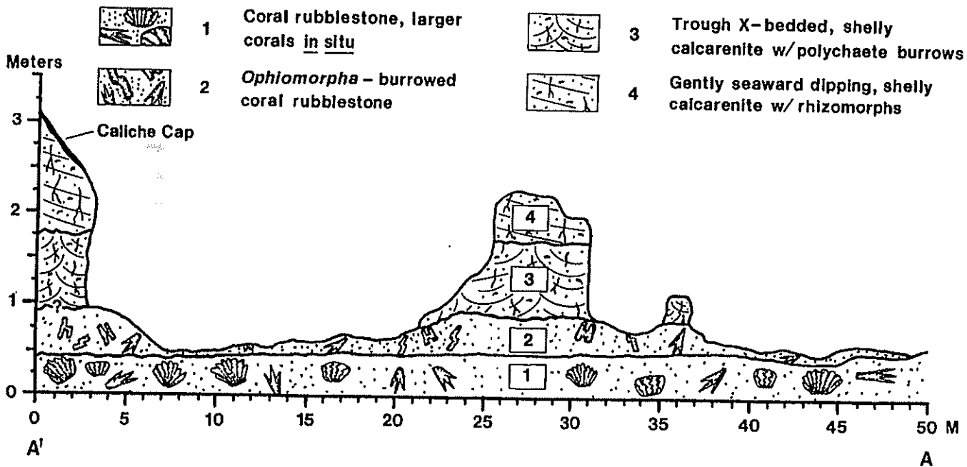
Fig. 14. Profile A-A' from the Devil's Point coral reef. A wave-cut bench occurs at the top of Facies 1 on this profile and Profile B-B' (Fig. 15).
