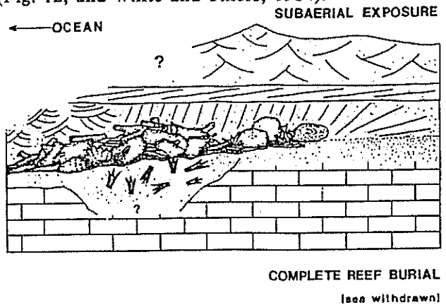
Fig. 12. Complete burial of the Cockburn Town coral reef, shortly after 119 kybp.
