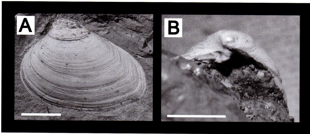
Figure 10. Photographs of shells of Pachydon macriformis Meek and Hayden from the Van Daele shell bed, Section B-56 (Belt et al., 2004, fig. 9), Little Missouri River district. A , Exterior view of right valve. B , Cardinal tooth in a right valve. Scale bars 5 mm.
