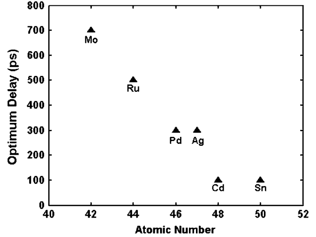
Fig. 3. Optimum delay between the 120-ps, \sim 350 -mJ prepulse, and the 8-ps, \sim 1 -J short pulse, for 4d^1S_0 \rightarrow 4p^1P_1 lasers on the different Ni-like ions; Z = 42 (Mo), Z = 44 (Ru), Z = 46 (Pd), Z = 47 (Ag), Z = 48 (Cd), and Z = 50 (Sn).
