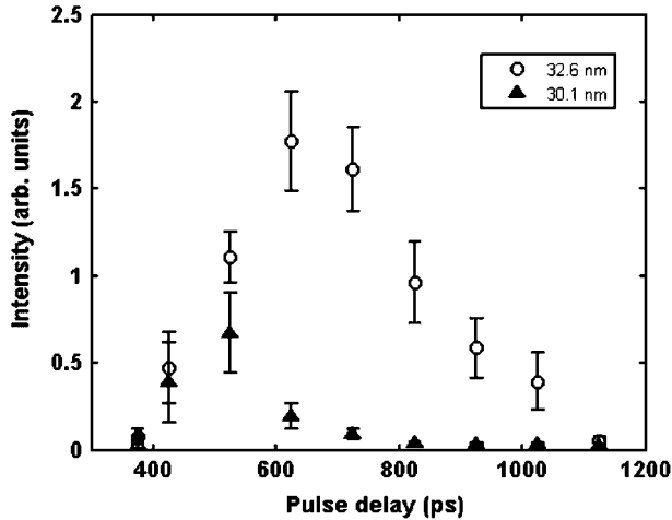
Fig. 11. Variation of the intensity of the 32.6- and 30.1-nm lines of Ne-like Ti as a function of time delay between the 120-ps prepulse and the 8 ps. The grazing incidence angle was 20^\circ .
