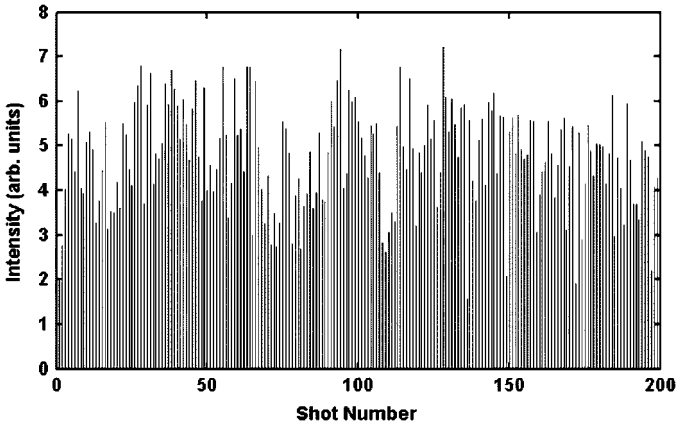
Fig. 8. Shot to shot variation of the intensity of the 14.7-nm laser line of Ni-like Pd for a series of 200 laser shots obtained at 5-Hz repetition rate with \sim 1 J of short pulse excitation. The stability is characterized by a standard deviation that is 24% of the mean.
