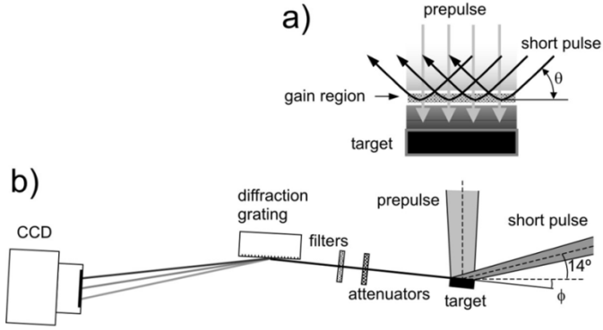
Fig. 1. (a) Schematic representation of the grazing incidence pump geometry. The short pulse impinges onto the target at a grazing incidence angle \theta . (b) The experimental setup. The angle \phi between the normal to the target surface and the axis of the prepulse beam is varied by tilting the target to obtain the different short pulse grazing incidence pump angles \theta used in this work (e.g., \phi = 6 added to the 14^\circ angle of the short pulse beam axis gives a 20^\circ grazing incidence angle).
