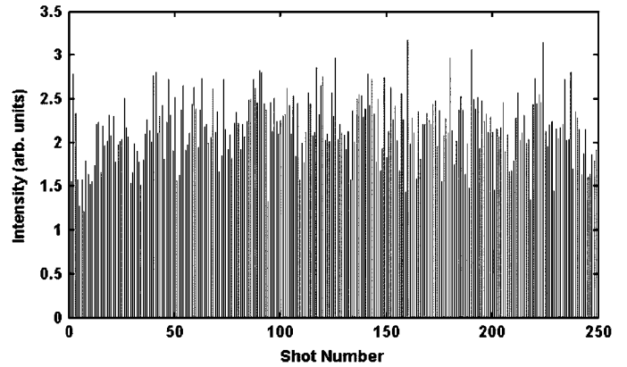
Fig. 13. Shot to shot variation of the intensity of the 32.6-nm laser line of Ni-like Ti at 5-Hz repetition rate. The standard deviation of the series is 17% of the mean.
