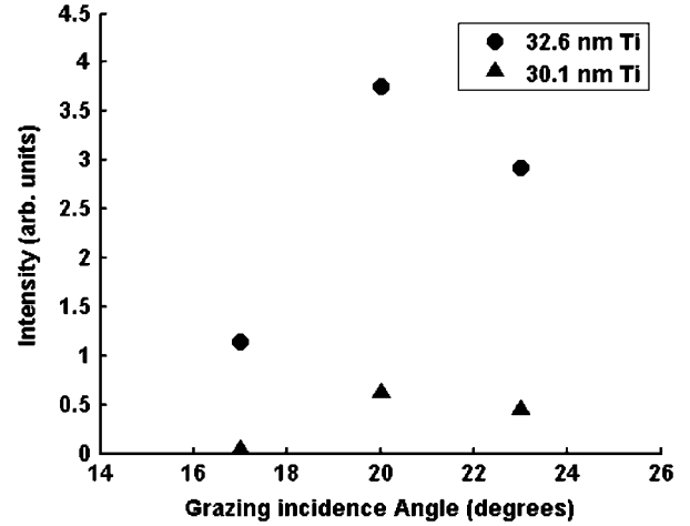
Fig. 9. Laser output intensity corresponding to the 30.1- and 32.6-nm lines of Ne-like Ti versus grazing incidence angle of the 8-ps duration heating pulse.
