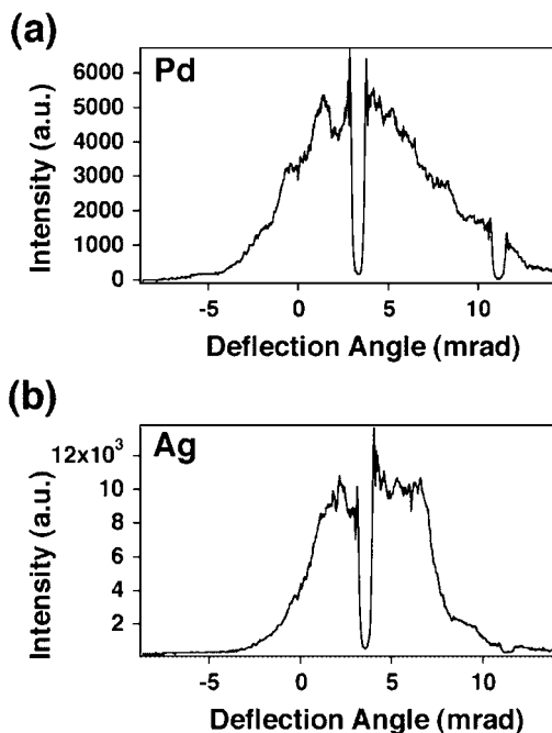
Fig. 15. Plots of the horizontal beam divergence and deflection angles for the (a) Ni-like Pd and (b) Ag spectral lines relative to the target surface. The dips in the profiles are from fiducial wires aligned between the target and the on axis spectrometer.
