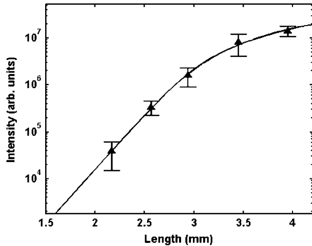
Fig. 12. Laser output intensity of the 32.6-nm line of Ne-like Ti as a function of target length. A best fit of the data with an analytical expression that relates the gain and the output laser intensity taking into account gain saturation yields a small signal gain coefficient of 56.5 \text{ cm}^{-1} , and a gain-length product g \times l = 18.4 .
