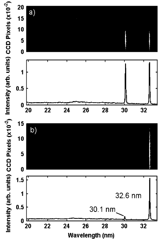
Fig. 10. On-axis Ne-like Ti spectra, measured at 20^\circ grazing incidence. (a) 520-ps delay between prepulse and short pulse, both lines show similar intensity. (b) 620-ps delay, where the 32.6-nm dominates the spectrum.
