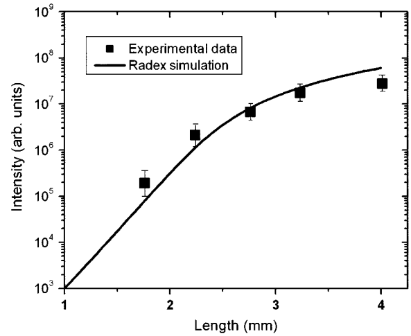
Fig. 6. Intensity versus length for the 14.7-nm line of Ni-like Pd. Each of the points is an average of ten or more laser shots. The line is the result of a simulation performed with the code RADEX corresponding to a small signal gain coefficient is 63 \text{ cm}^{-1} and the gain-length product is g \times l = 17.2 .
