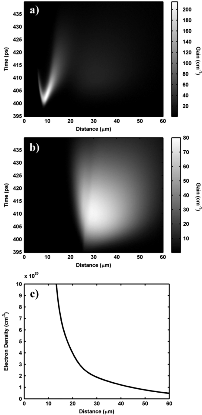
Fig. 2. Simulated gain maps for a Ni-like Pd 14.7-nm laser at the moment of peak gain for (a) normal incidence irradiation, (b) 20^\circ grazing incidence irradiation, and (c) simulated electron density profile of the prepulse at the moment of the short pulse arrival. At normal incidence the region of large gain coefficient coincides with large density gradients that rapidly refract the beam out of the narrow gain region. For a pump angle of 20^\circ the beam heats the plasma where N_e = 2 \times 10^{20} \text{ cm}^{-3} , creating large gain in a region where reduced refraction allows the beam to effectively propagate and amplify. The plasma is assumed to be created by a 120-ps normal incidence prepulse with an intensity of 2.4 \times 10^{12} \text{ W}\cdot\text{cm}^{-2} , and heated after a 300-ps delay by an 8-ps duration, 800-nm wavelength, pulse focused to an intensity of 8 \times 10^{13} \text{ W}\cdot\text{cm}^{-2} , both line foci are 30\text{-}\mu\text{m} -wide FWHM.
