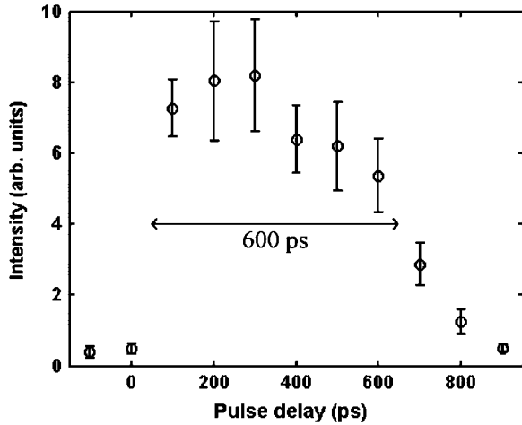
Fig. 7. Intensity versus time delay between the 120-ps main prepulse and the 8-ps grazing incidence short pulse for the 14.7-nm laser line of Ni-like Pd.
