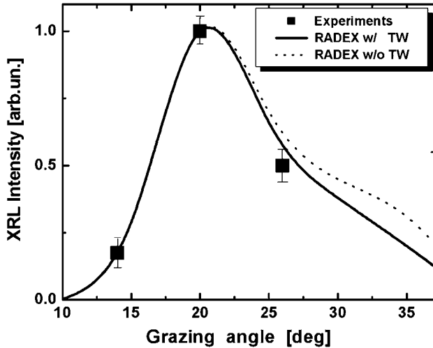
Fig. 5. Measured dependence of laser output intensity of the 14.7-nm laser line of Ni-like Pd as a function of grazing incidence angle. The two curves represent results of RADEX simulations for the cases with and without the traveling wave mismatch effect included.
