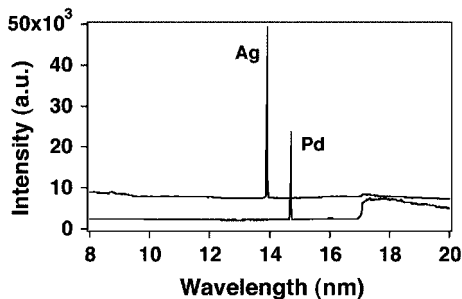
Fig. 14. Ni-like Pd and Ni-like Ag spectra from targets irradiated with a 1.3-J, 1054-nm, 600-ps pulse, and a 1.5-J, 527-nm, 1.5-ps short pulse. Both target lengths are 8 mm. The Pd, Ag spectra are filtered with 200-nm Al and 200-nm Lexan/75 nm Al, respectively, to prevent the CCD detector from saturating.
