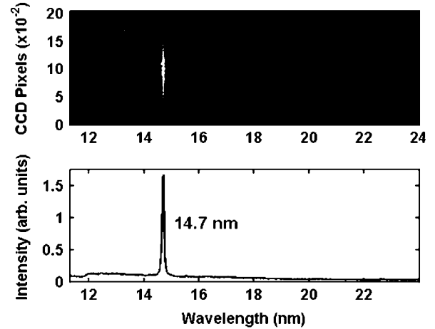
Fig. 4. Single shot on axis spectra of 4-mm-long line focus Pd plasma showing lasing in the 14.7-nm transition.
