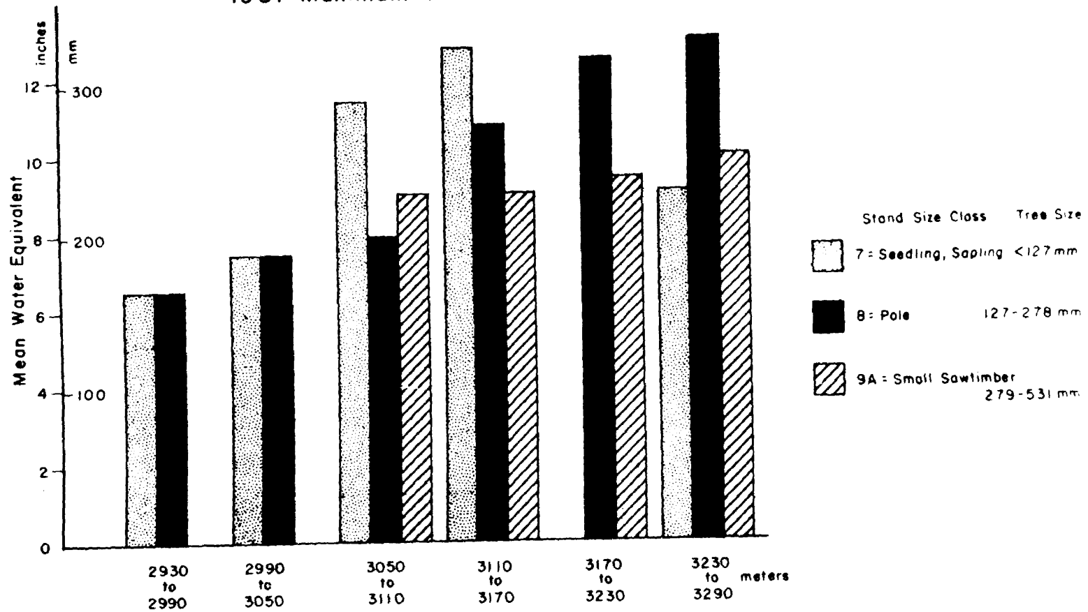
Figure 4 Distribution of Snow Pack by Tree Size Class and Elevation 1967 Maximum Snow Pack
