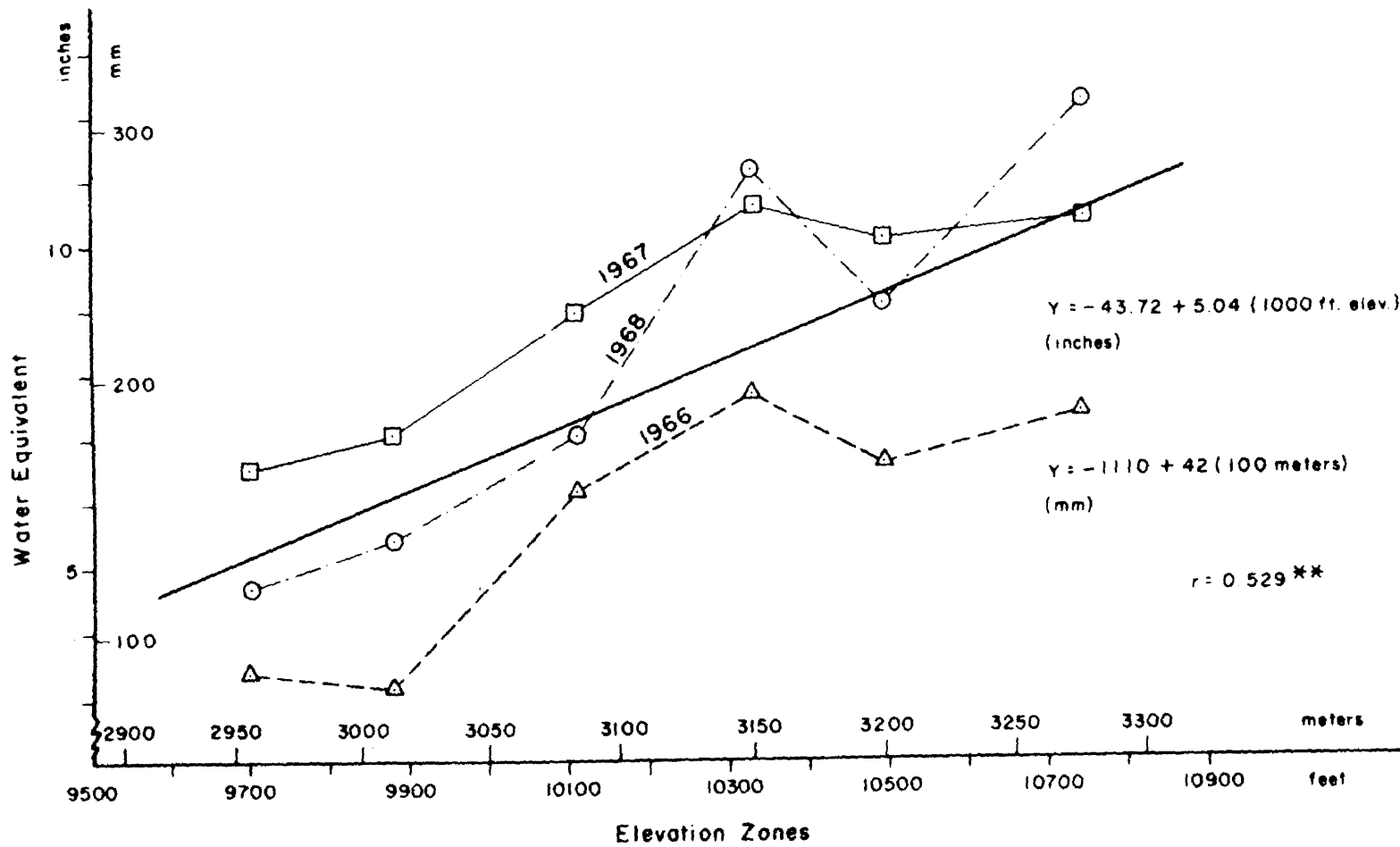
Figure 3. Snow Pack Accumulation Variation by Elevation Zones and Year
