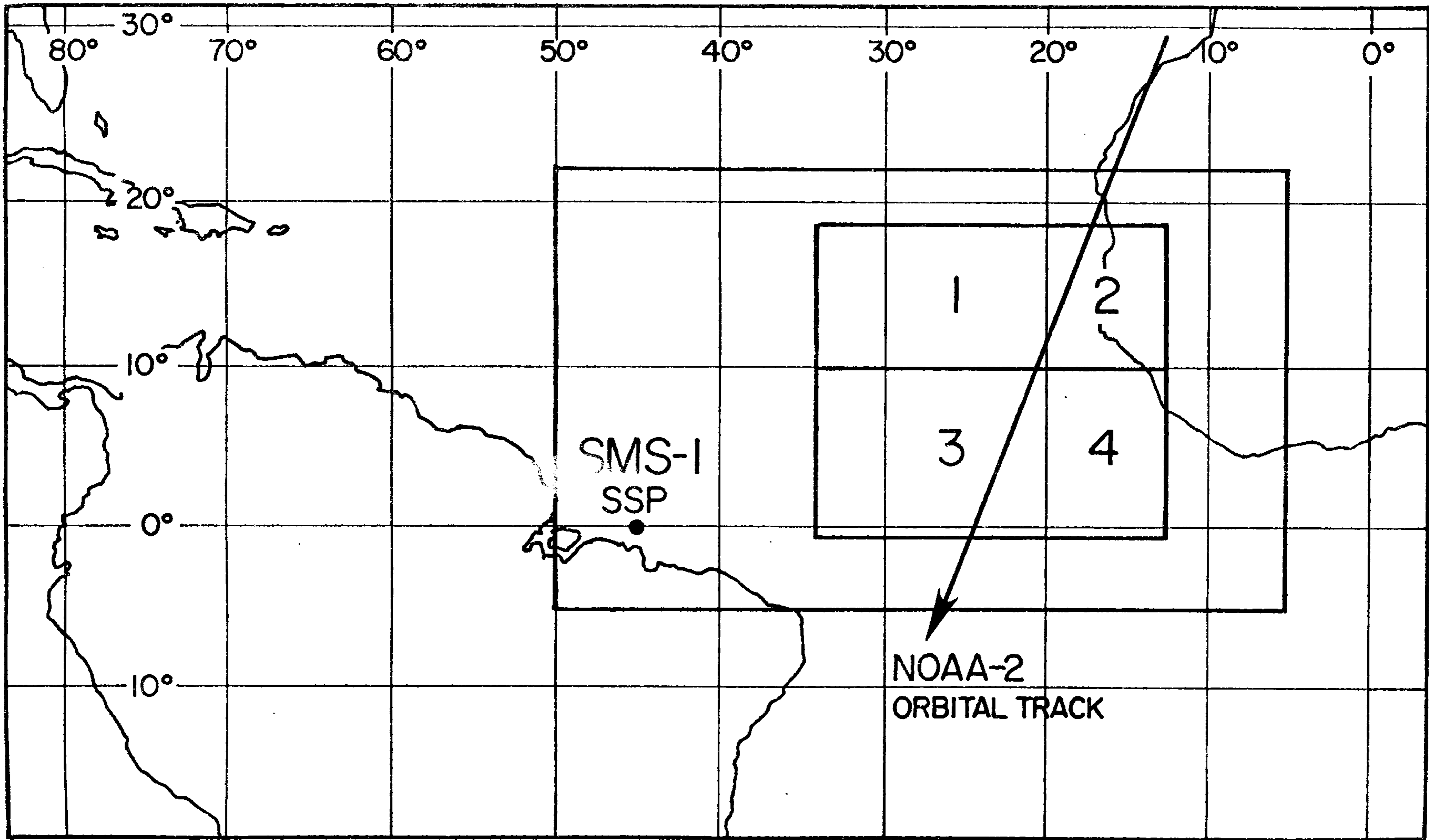
Figure 10. GATE sector and the four regions of simultaneous measurements by SMS-1 and NOAA-2 on September 17, 1974 near 1000 GMT.
