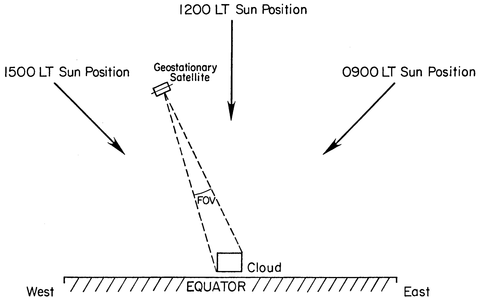
Figure 4. Relative positions of the satellite and a finite cloud situated in the equatorial plane at the equinox.
