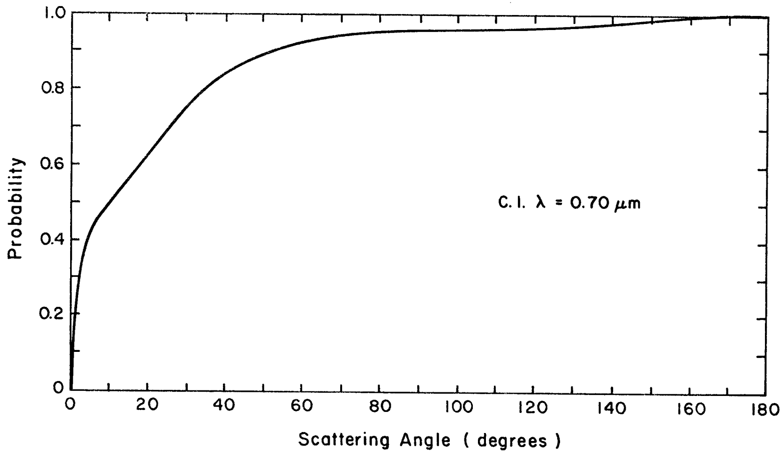
Figure 1. Cumulative distribution function for C1 model at \lambda = 0.7 \mu\text{m} (from DeMaria and McKee, 1979).
