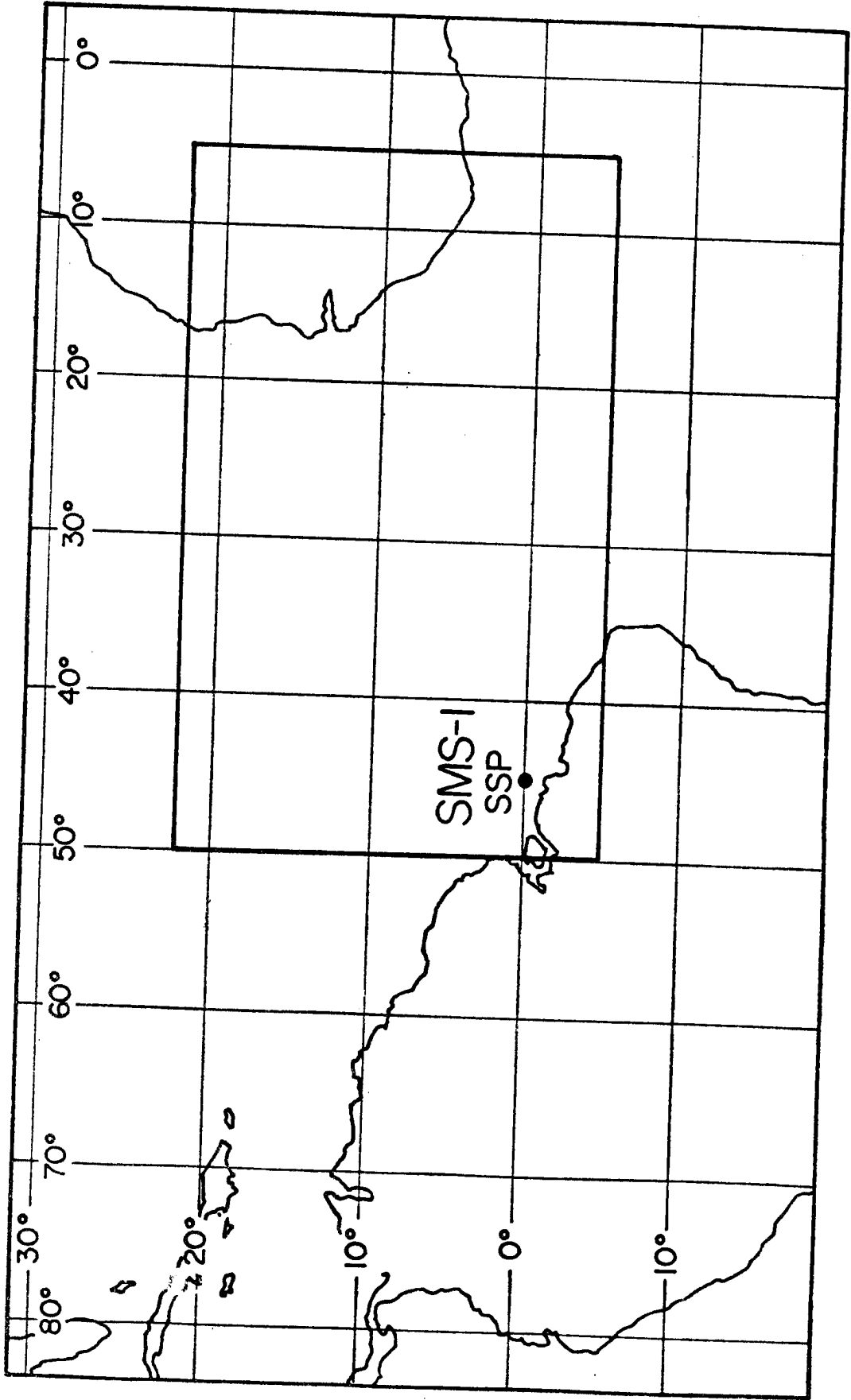
Figure 8. GATE sector and SMS-1 satellite subpoint (SSP).
