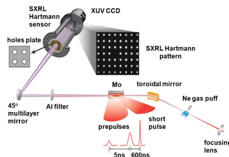
Fig. 1. Schematic diagram of the experimental setup to measure the wavefront of an injection-seeded SXRL based on solid target plasma with a Hartmann sensor.
