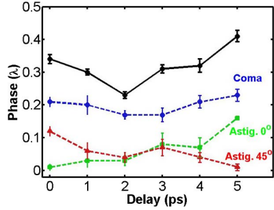
Fig. 4. Total measured SSXRL wavefront distortion (black line, top curve). Aberrations as a function of delay between the injection of the HHG seed and the peak of the amplifier pump pulse for coma (blue dashed line), astigmatism at 0^\circ (green-dashed line), and astigmatism at 45^\circ (red-dashed line).
