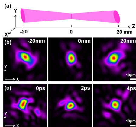
Fig. 5. (a) Diagram of reconstructed SSXRL propagation around the plasma amplifier along the Rayleigh length. (b) False color images of the reconstructed SSXRL transverse intensity distribution at Z = -20, 0 , and 20 mm, with Z = 0 mm corresponding to the central position of the plasma and also to the region of least confusion. The delay is at 2 ps. (c) Reconstructed SSXRL intensity maps at Z = 0 mm for various delays between HHG seed and pump laser pulse. The length of the plasma amplifier is 4 mm. The case at 0 ps corresponds to the seed arriving at the peak of the amplifier short pump pulse.
