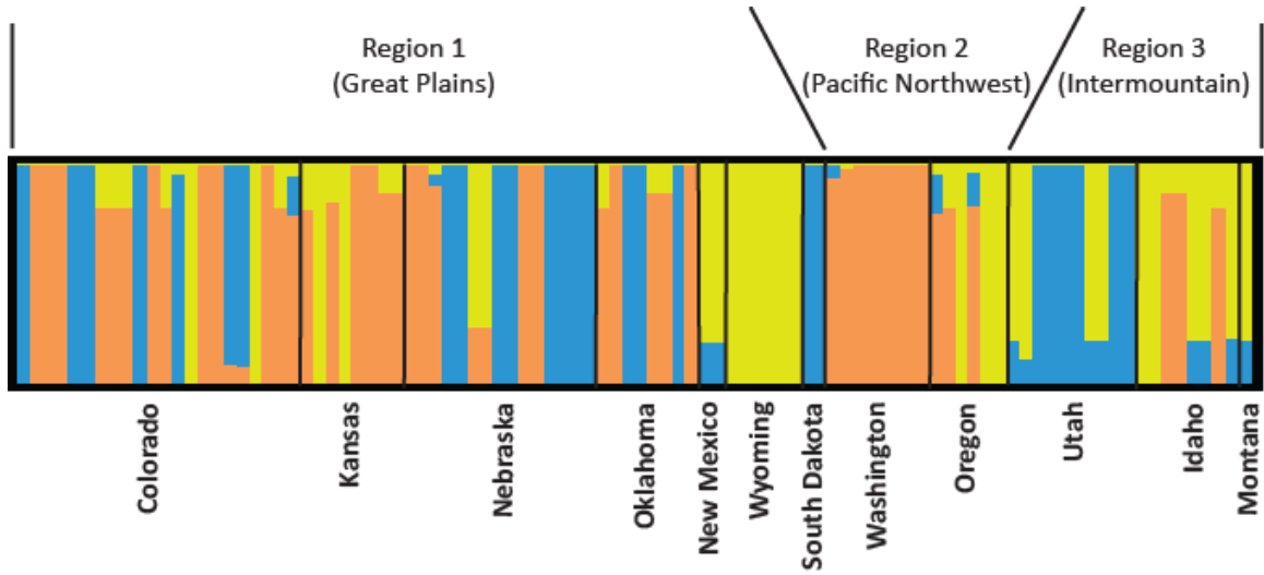
Figure 1.1. Structure results from the large-scale U.S. collection of jointed goatgrass using K=3 , without admixture. Orange depicts K1, blue K2, and yellow K3 for the corresponding ancestry table (Table A1.4).
