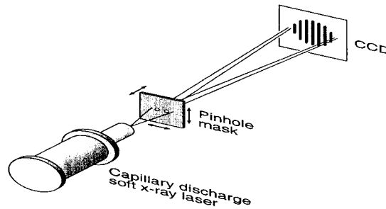
Figure 1. Experiment Setup
