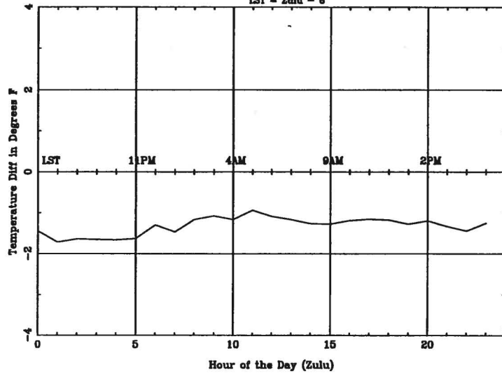
Average Diurnal Cycle for FAR - summer LST = Zulu - 6
