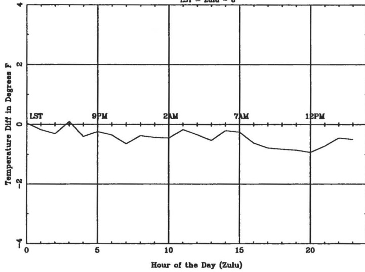
Average Diurnal Cycle for PDX - spring LST = Zulu - 8
