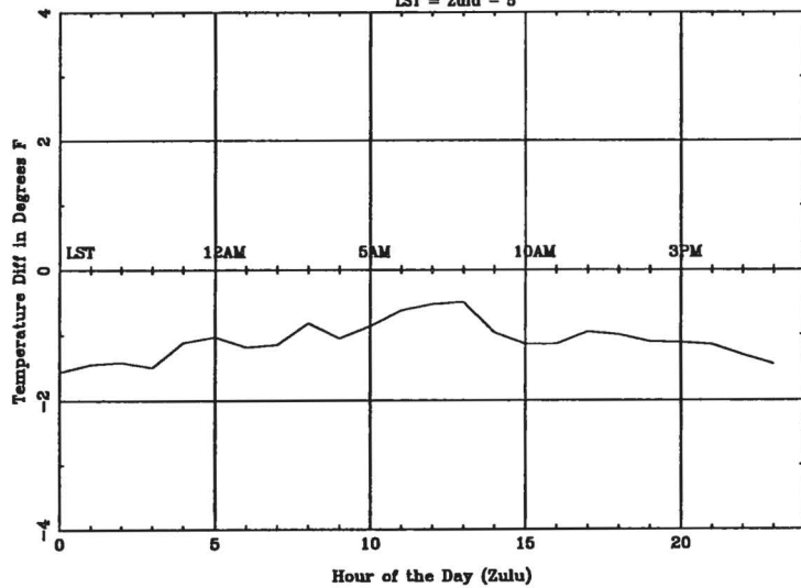
Average Diurnal Cycle for TRI - spring
