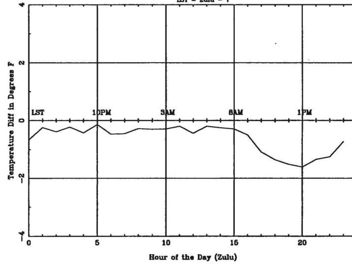
Average Diurnal Cycle for MSO - summer
