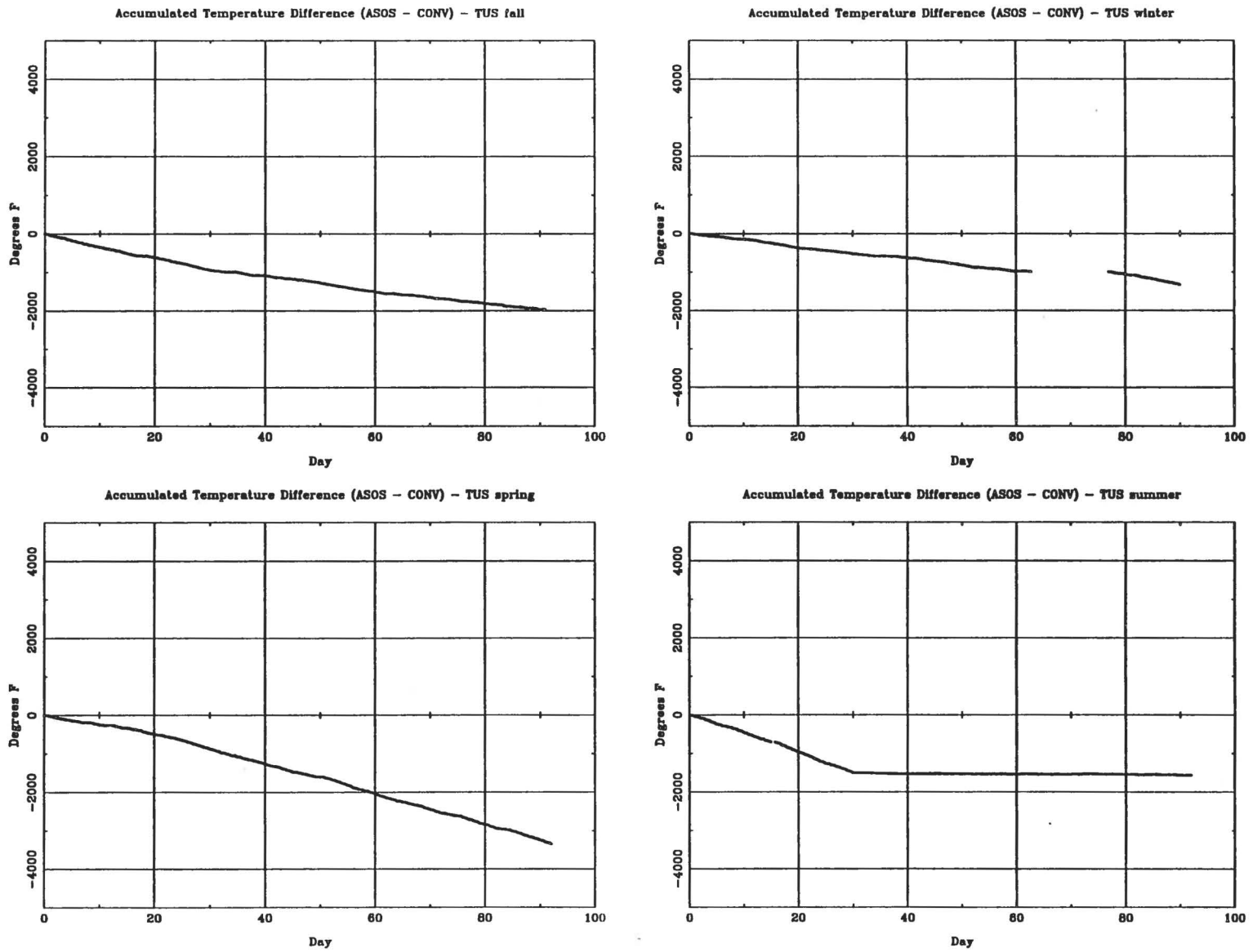
Fig. 3.1 (E) Seasonal accumulated temperature difference plots for Tucson, AZ.
