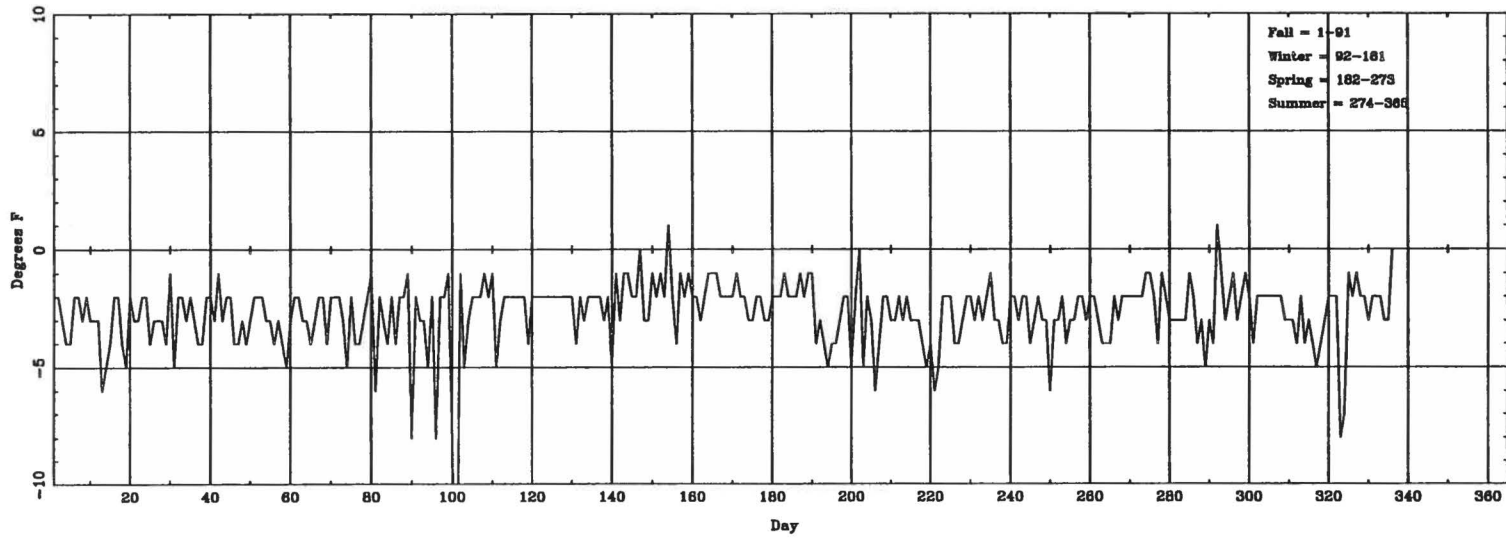
Daily \Delta T_{\text{(lowest hourly)}} (ASOS - CONV) for ATL
