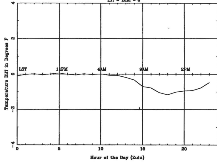
Average Diurnal Cycle for AUS - summer LST = Zulu - 6
