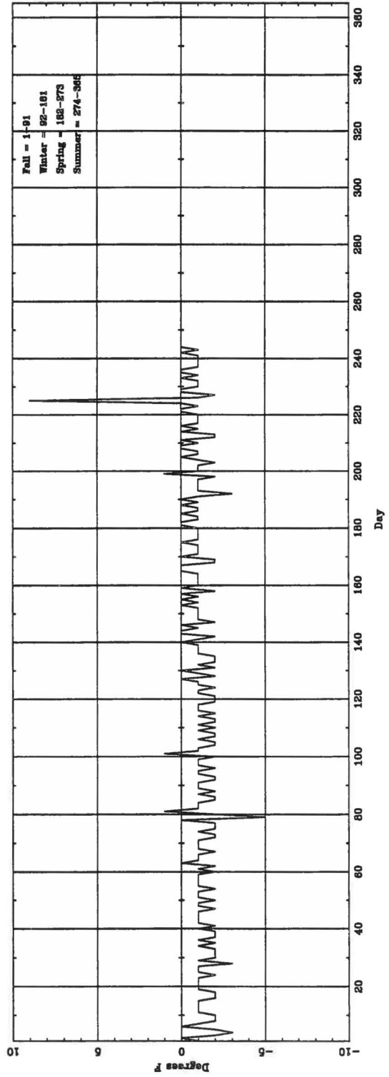
Daily \Delta T_{(correct\ hour)} (ASOS - CONV) for BIL
