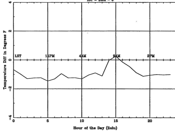
Average Diurnal Cycle for LBB - summer LST = Zulu - 6
