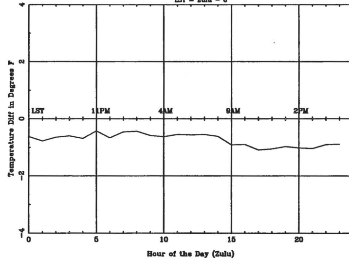
Average Diurnal Cycle for SJT - summer LST = Zulu - 6
