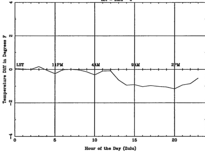
Average Diurnal Cycle for PAH - spring
