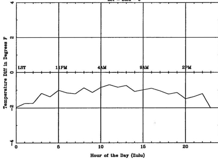
Average Diurnal Cycle for SGF - spring LST = Zulu - 6
