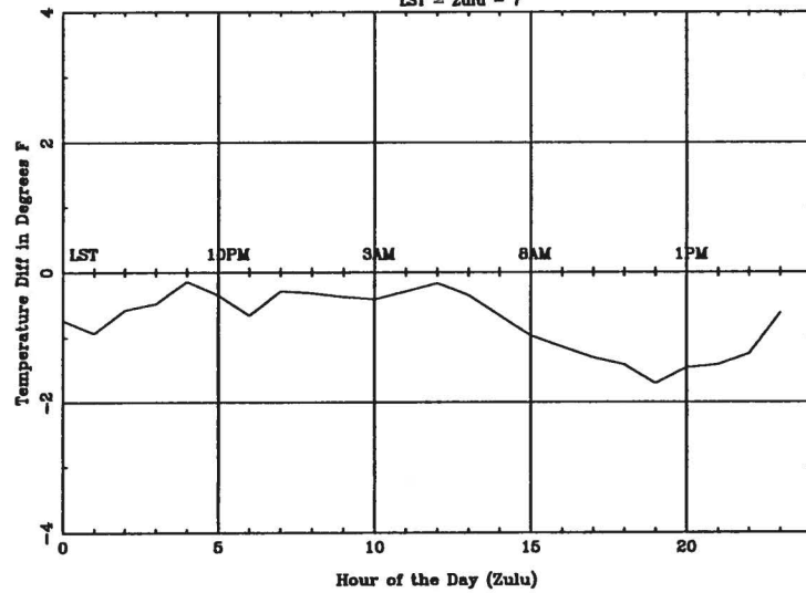
Average Diurnal Cycle for MSO - spring
