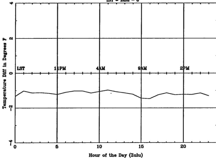
Average Diurnal Cycle for FAR - spring LST = Zulu - 6
