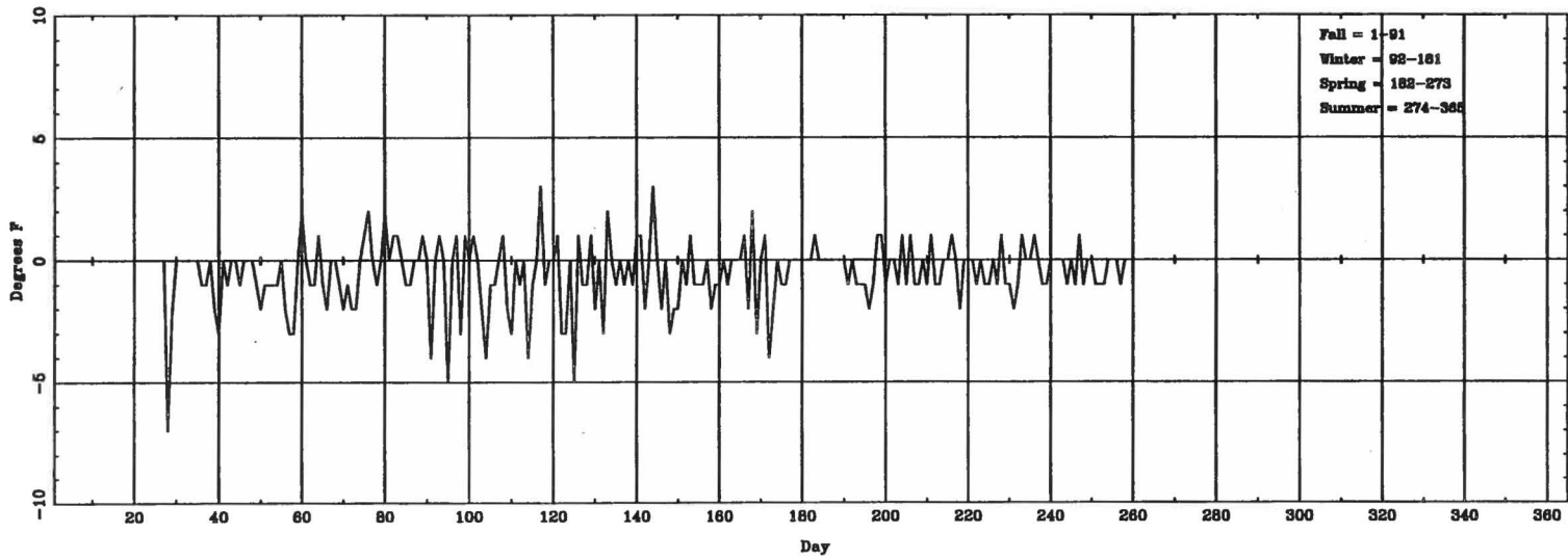
Daily AT (lowest hourly) (ASOS - CONV) for ISN
