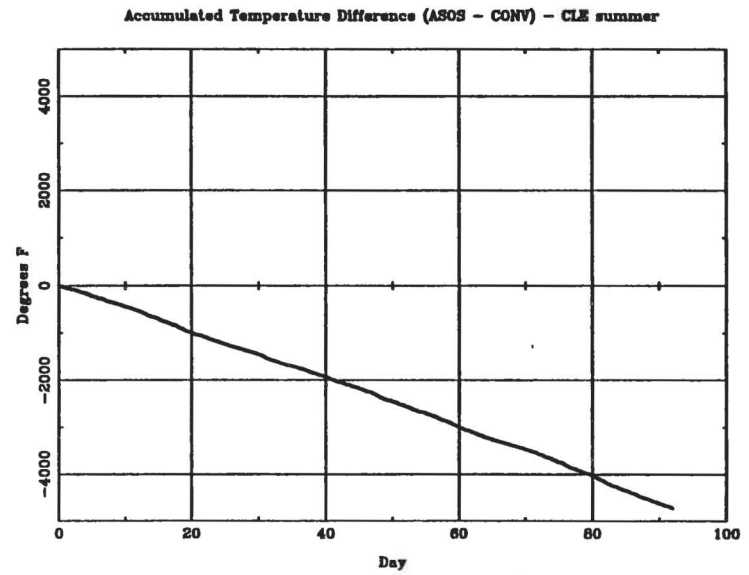
Fig. 3.1 (C) Seasonal accumulated temperature difference plots for Cleveland, OH.
