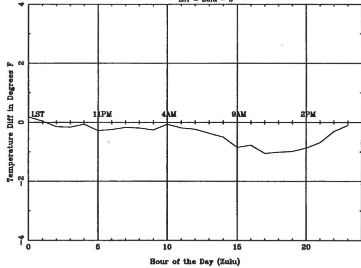
Average Diurnal Cycle for PAH - summer
