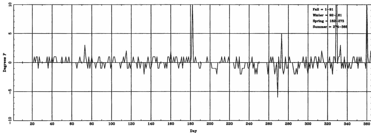
Daily \Delta T_{\text{(lowest hourly)}} (ASOS - CONV) for VTN
