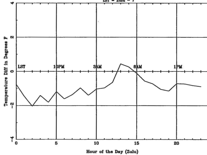
Average Diurnal Cycle for GJT - summer LST = Zulu - 7
