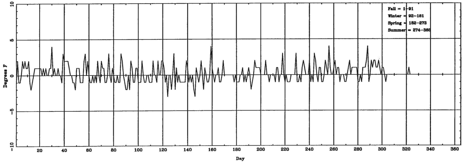
Daily \Delta T_{(lowest\ hourly)} (ASOS - CONV) for MLI
