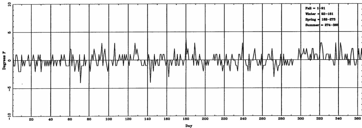
Daily \Delta T_{\text{(lowest hourly)}} (ASOS - CONV) for BIS
