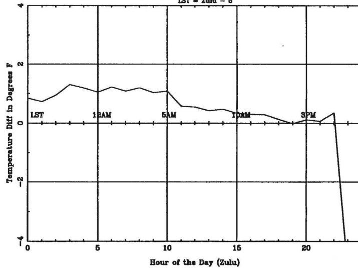
Average Diurnal Cycle for ORH - summer LST = Zulu - 5
