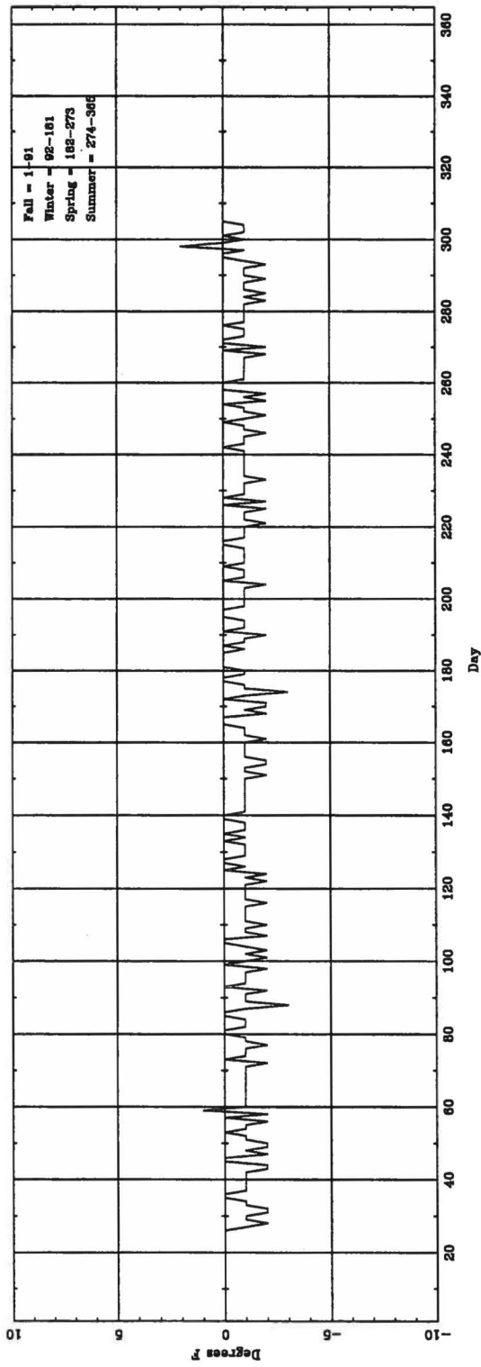
Daily \Delta T_{(night\ hour)} (ASOS - CONY) for AUS
