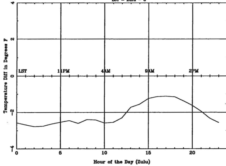
Average Diurnal Cycle for GRB - spring LST = Zulu - 6
