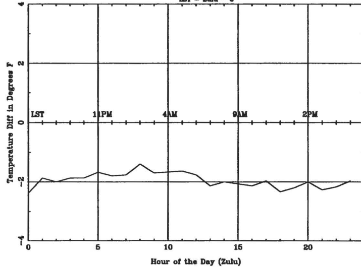
Average Diurnal Cycle for MKE - summer
