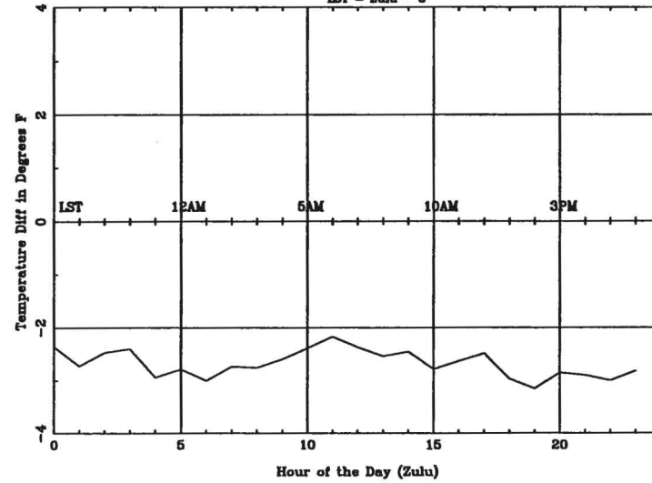
Average Diurnal Cycle for ATL - summer
