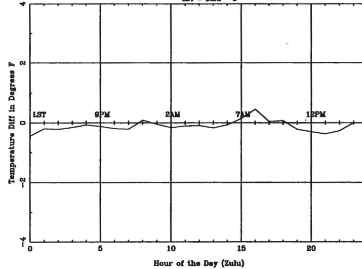
Average Diurnal Cycle for MHS - summer
