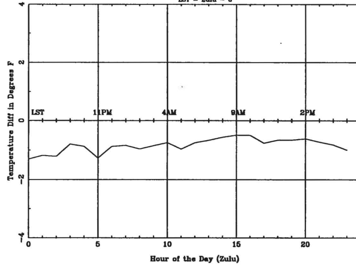
Average Diurnal Cycle for SGF - summer LST = Zulu - 6
