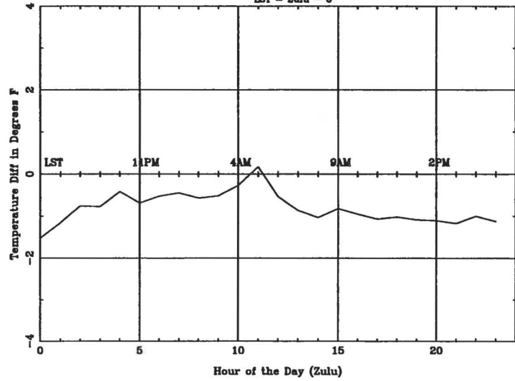
Average Diurnal Cycle for PAH - summer
