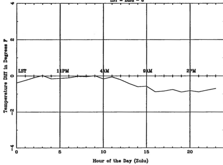
Average Diurnal Cycle for AUS - spring LST = Zulu - 6
