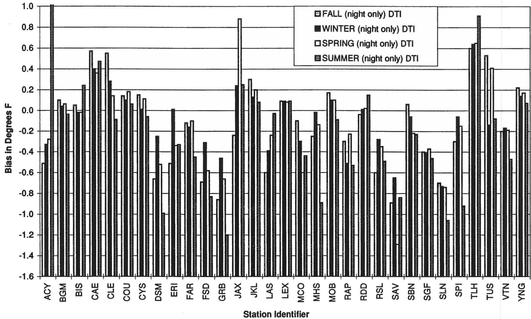
Fig. 3.8 (A) Seasonal distribution of nighttime local effects for four-season stations.
