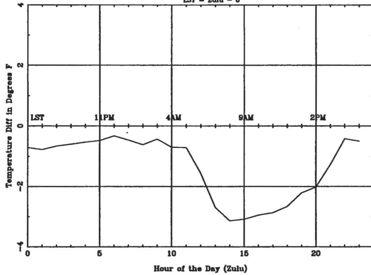
Average Diurnal Cycle for MSN - spring
