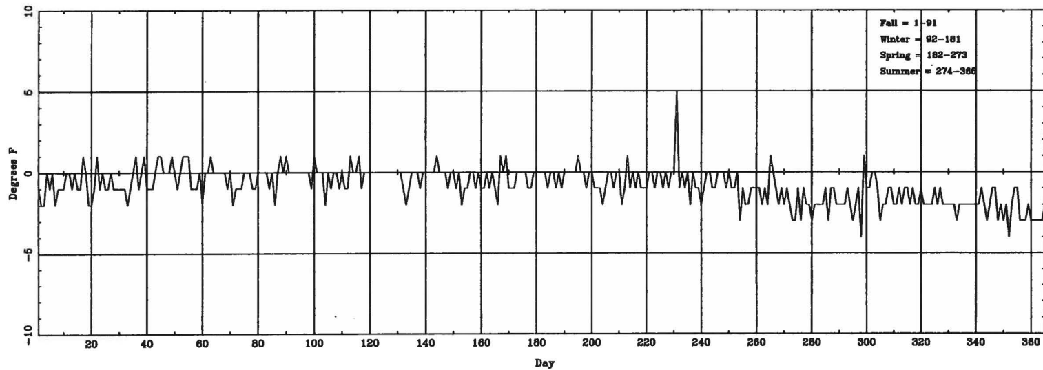
Daily \Delta T_{\text{(lowest hourly)}} (ASOS - CONV) for COU
