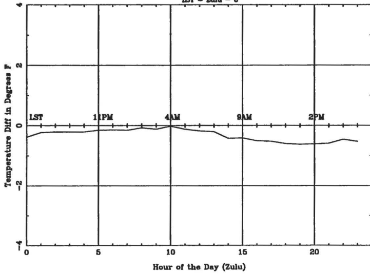
Average Diurnal Cycle for HON - spring LST = Zulu - 6
