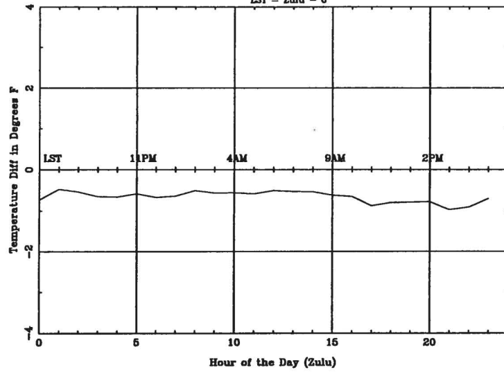
Average Diurnal Cycle for ALO - spring
