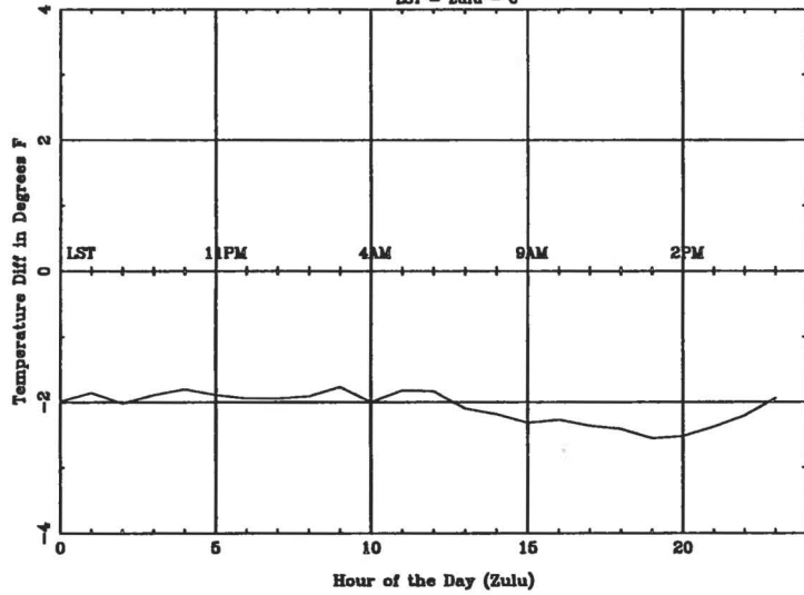
Average Diurnal Cycle for MKE - spring
