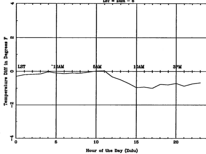
Average Diurnal Cycle for LEK - summer LST = Zulu - 5
