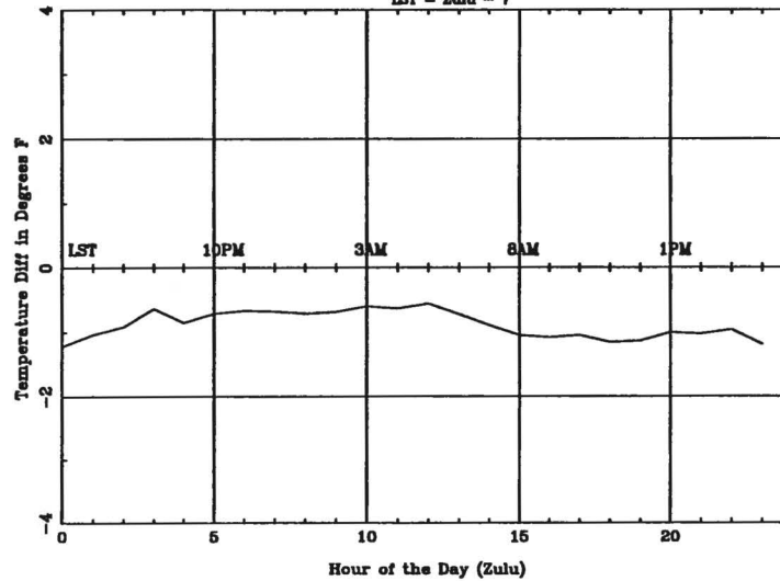
Average Diurnal Cycle for CYS - summer LST = Zulu - 7
