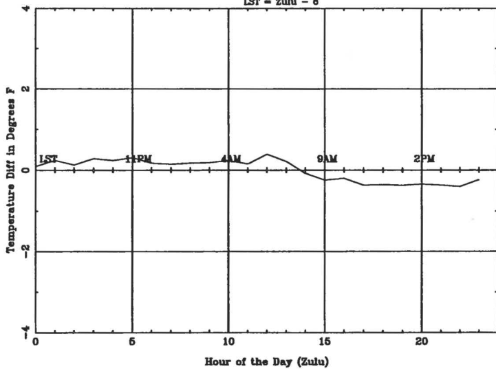
Average Diurnal Cycle for COU - spring
