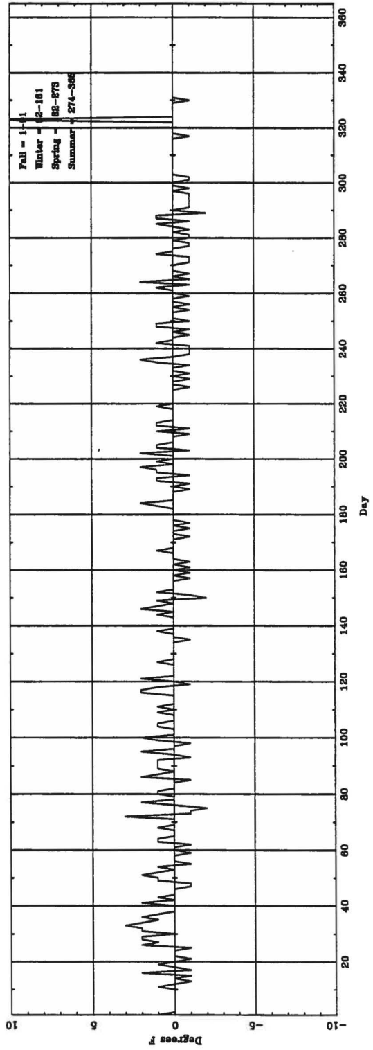
Daily \Delta T_{(nearest\ buoy)} (ASOS - CONV) for RFD
