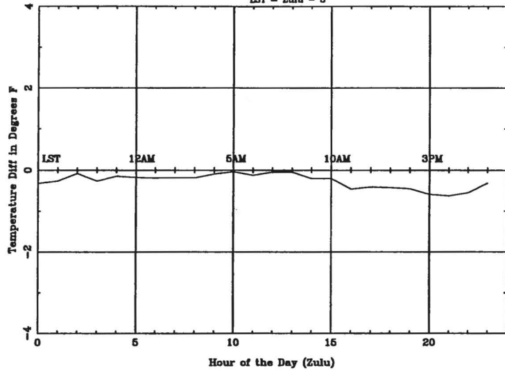
Average Diurnal Cycle for MKG - spring LST = Zulu - 5
