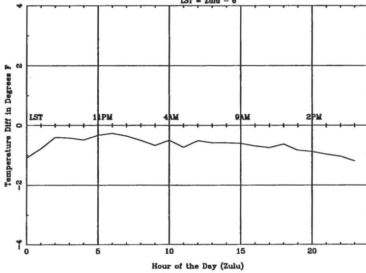
Average Diurnal Cycle for MCI - spring
