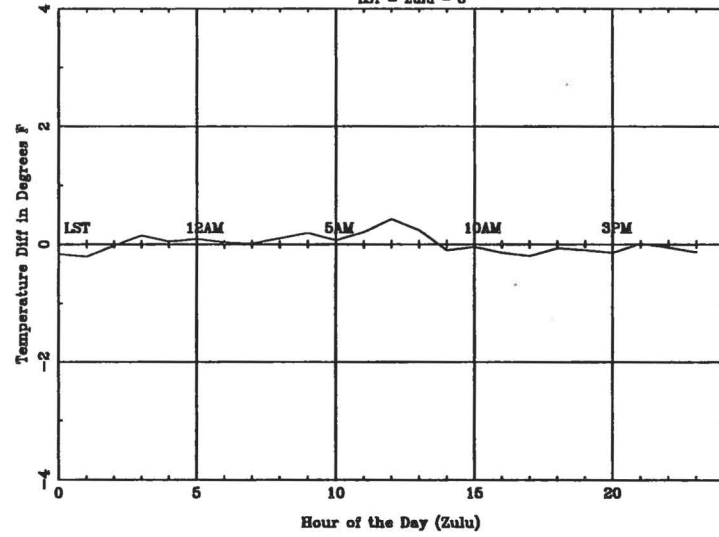
Average Diurnal Cycle for DAB - summer
