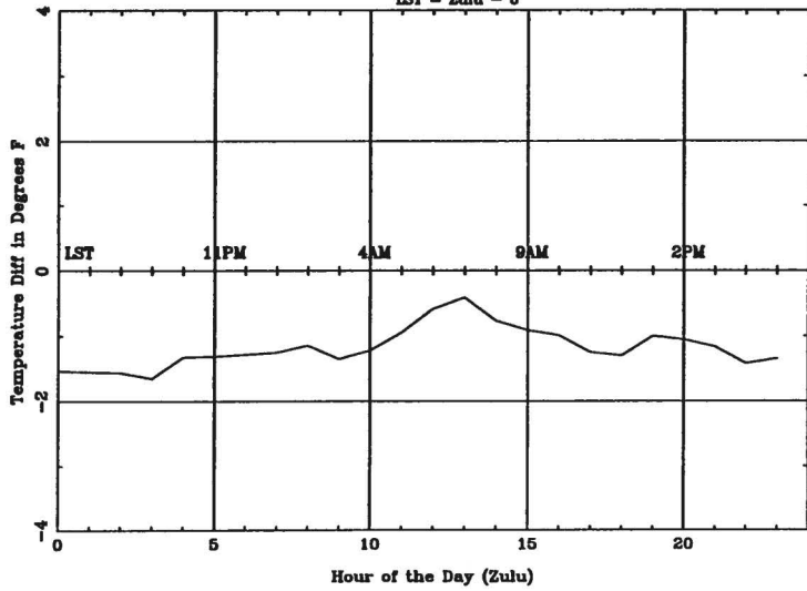
Average Diurnal Cycle for FSD - spring
