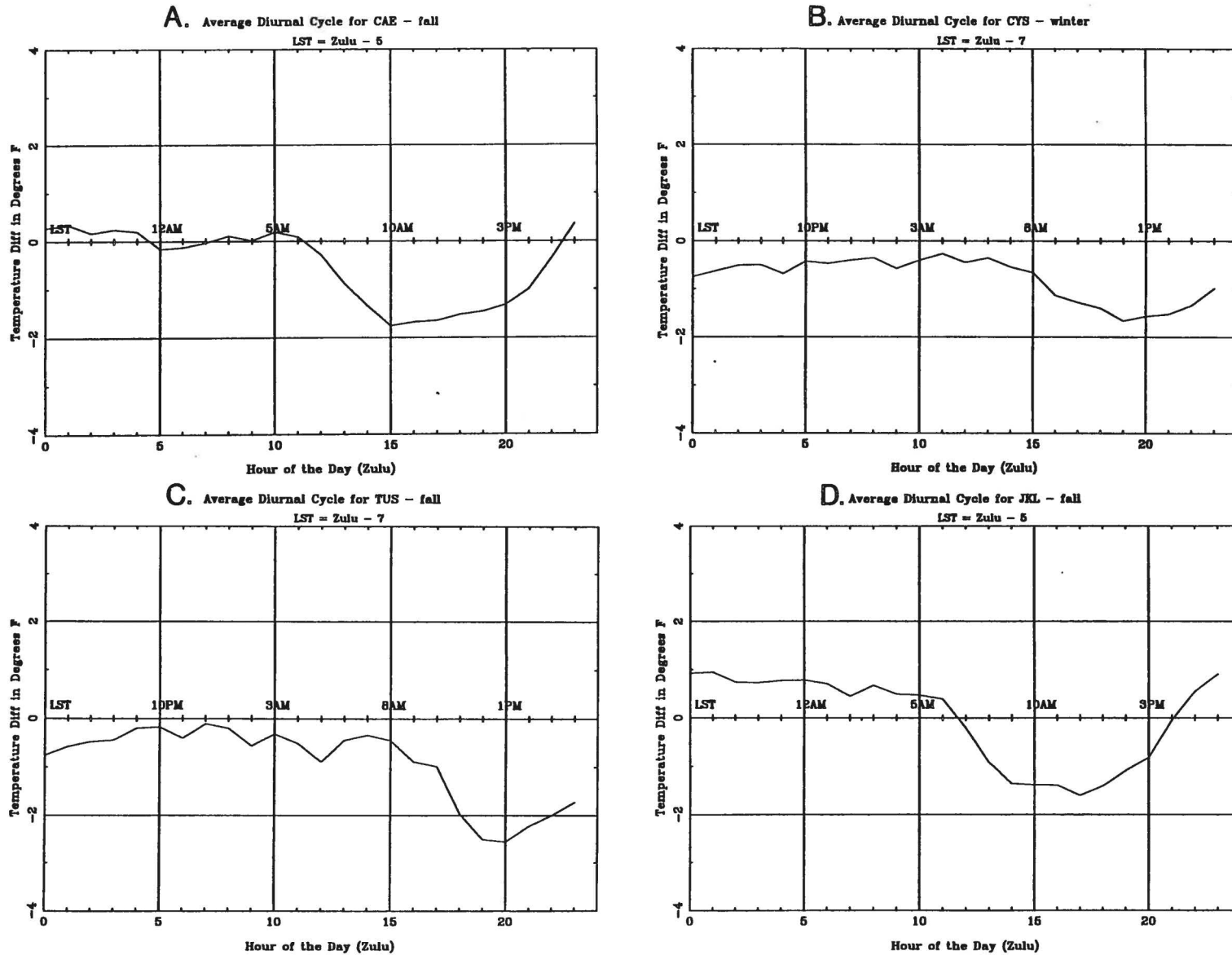
Fig. 3.7 (A) - (D) Seasonal diurnal temperature difference cycles showing daily pattern for majority of stations (daytime exhibits largest negative temperature differences.)
