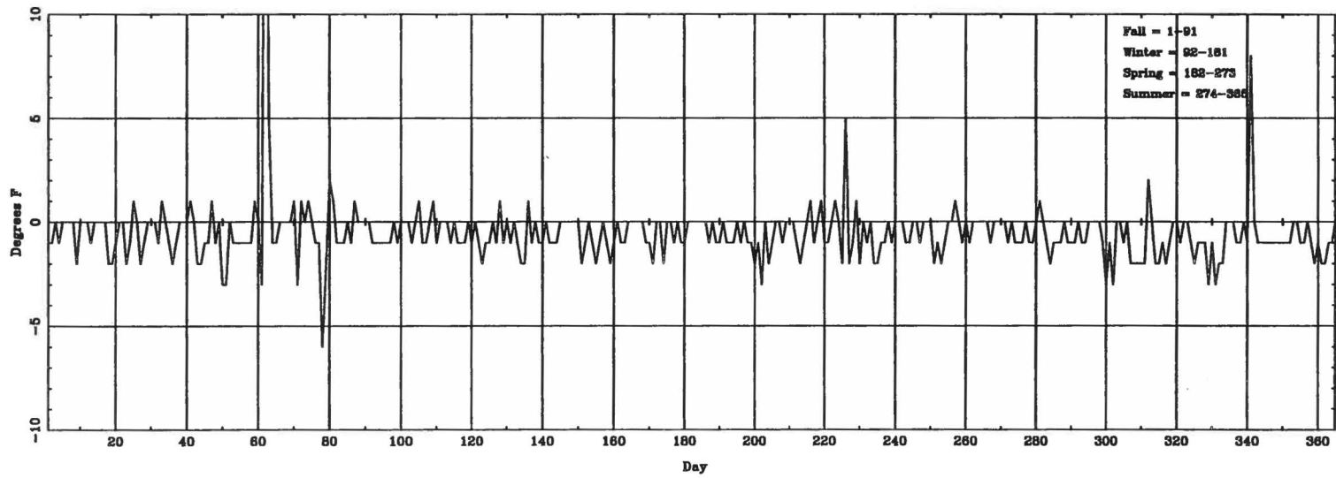
Daily \Delta T_{\text{(lowest hourly)}} (ASOS - CONV) for RSL
