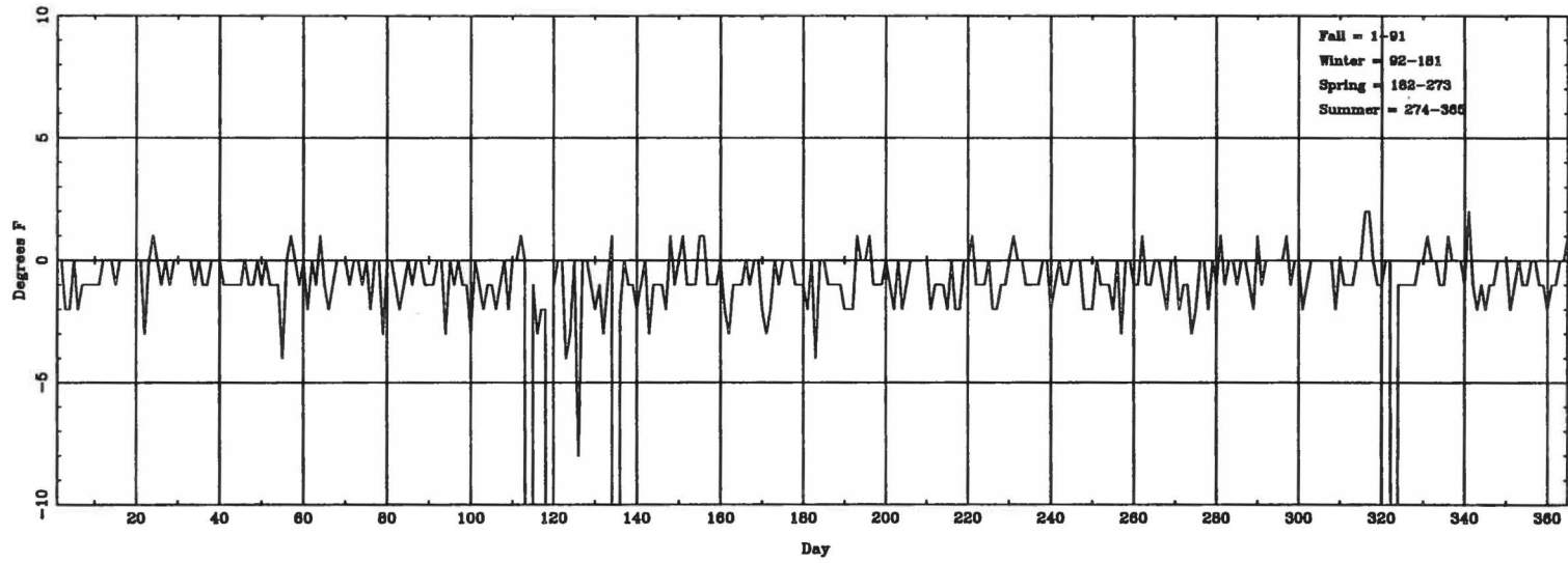
Daily \Delta T_{\text{(lowest hourly)}} (ASOS - CONV) for RSL
