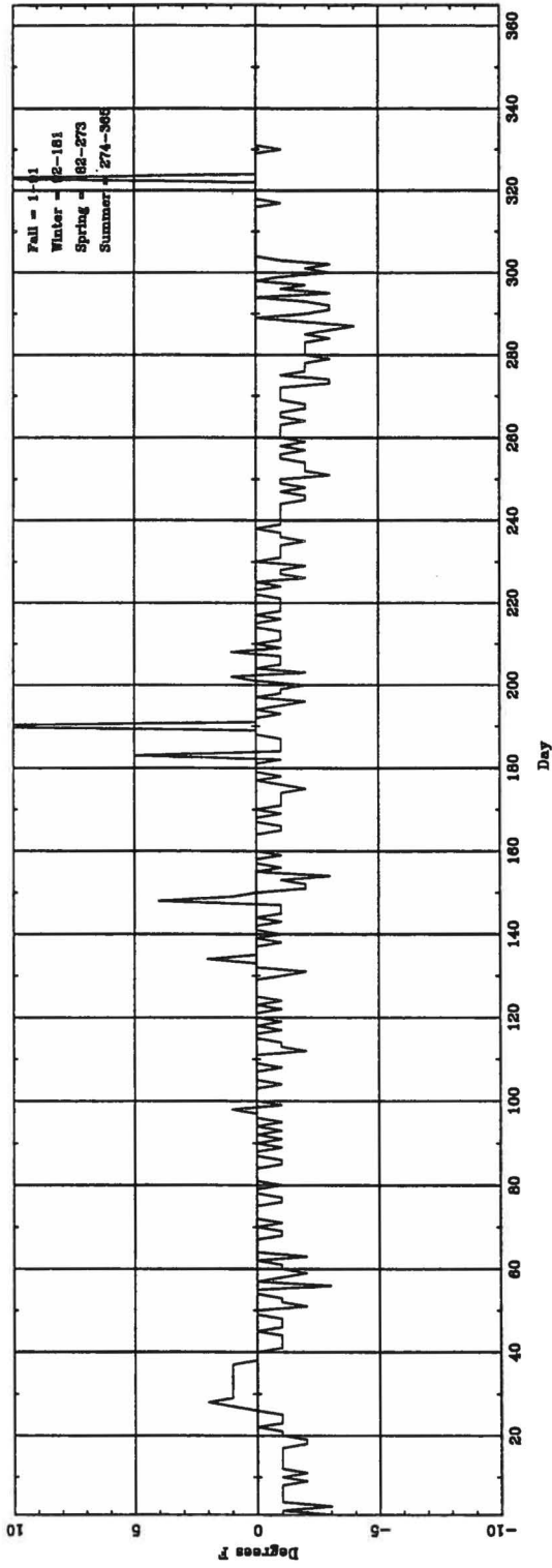
Daily \Delta T_{(distant\ buoy)} (ASOS - CONV) for RFD
