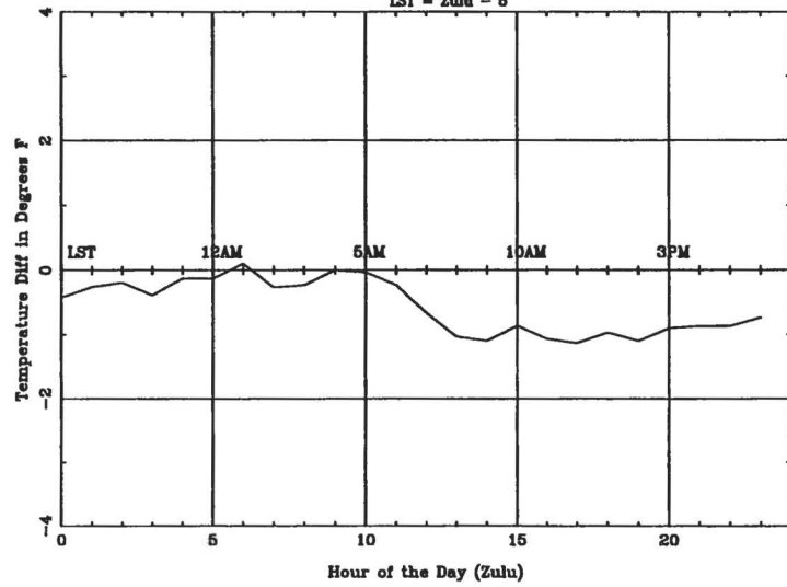
Average Diurnal Cycle for DTW - summer LST = Zulu - 5
