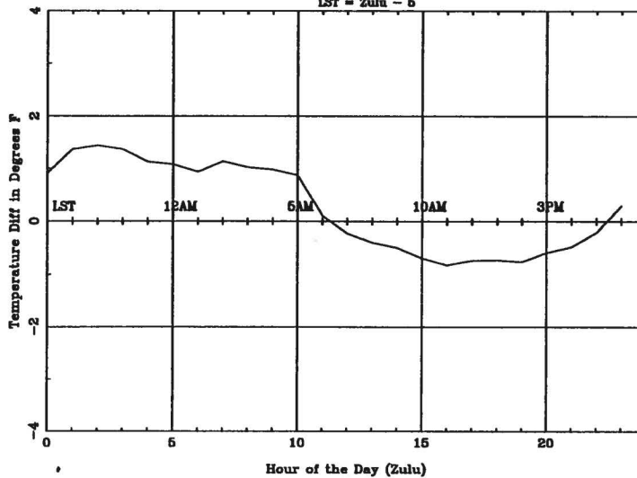
Average Diurnal Cycle for ACY - summer LST = Zulu - 5
