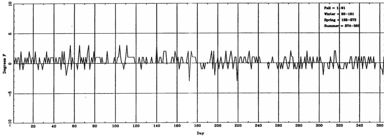
Fig. 3.10 (A) Temperature time series analysis for Jackson, KY.
