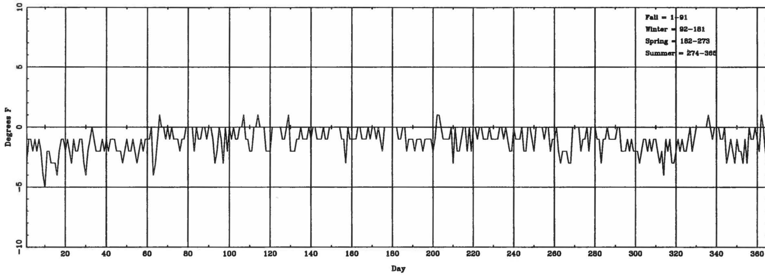
Daily \Delta T_{\text{(lowest hourly)}} (ASOS - CONV) for CAE
