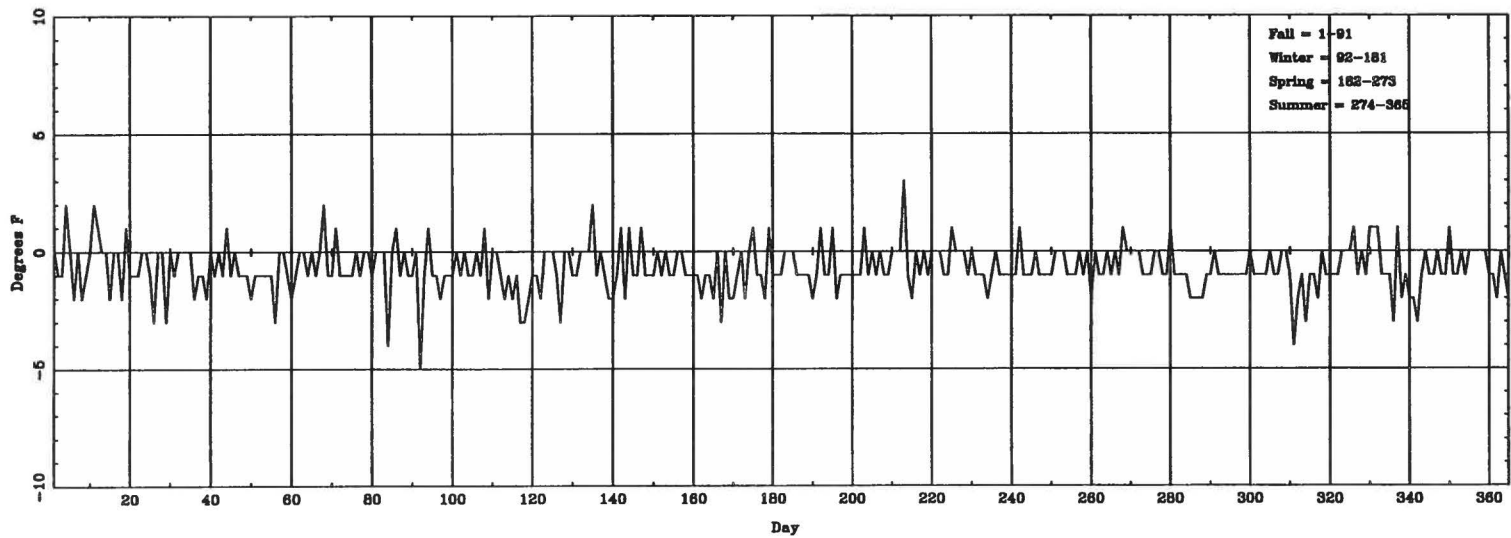
Daily \Delta T_{(lowest\ hourly)} (ASOS - CONV) for CYS
