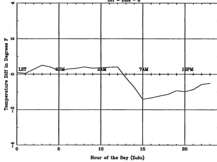
Average Diurnal Cycle for PDX - summer LST = Zulu - 8
