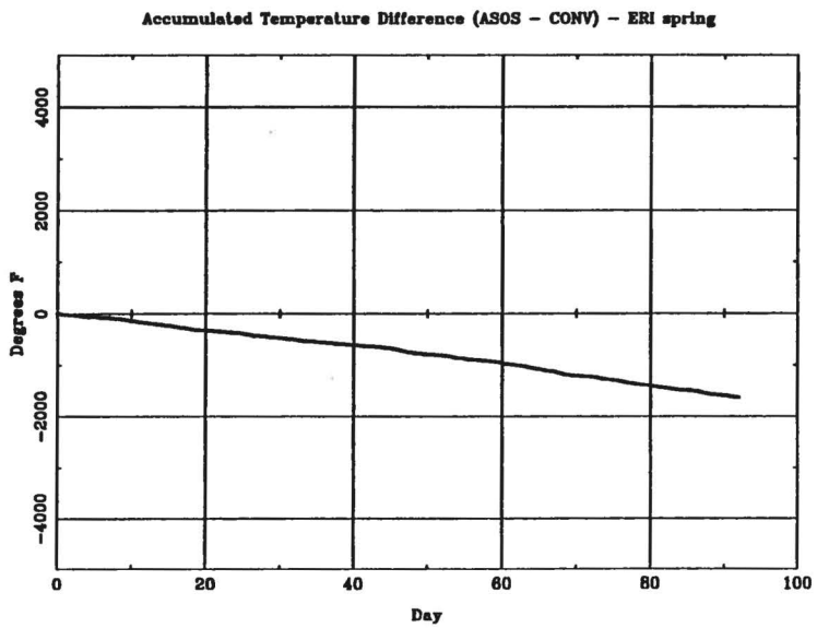
Fig. 3.1 (D) Seasonal accumulated temperature difference plots for Erie, PA.
