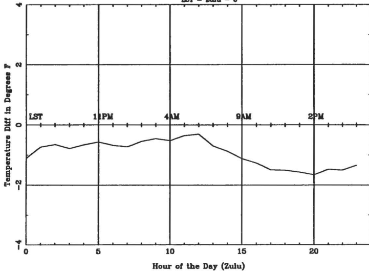
Average Diurnal Cycle for PAH - spring
