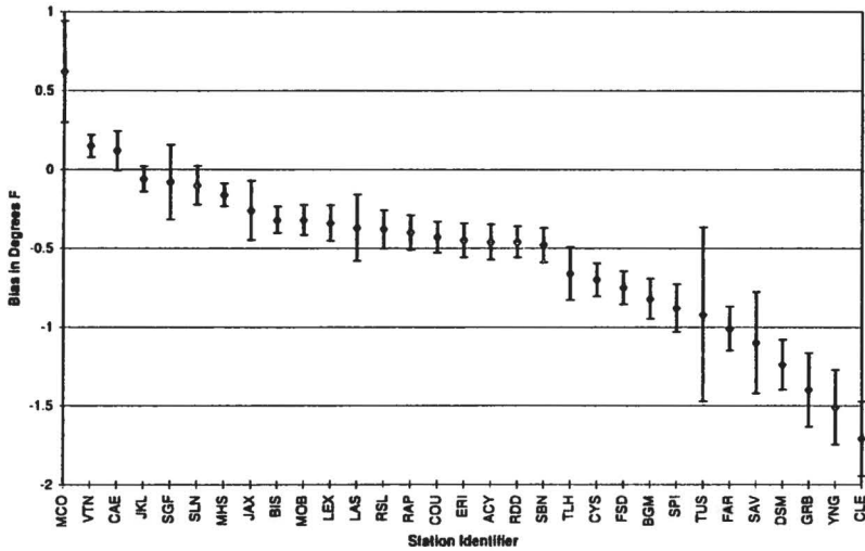
Fig. 3.5 Seasonal Instrument Biases for four-season stations plotted in order from most positive to most negative for the (A) fall, (B) winter, (C) spring, and (D) summer seasons.
