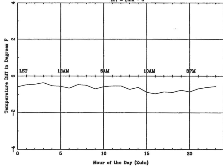
Average Diurnal Cycle for BGM - summer LST = Zulu - 5
