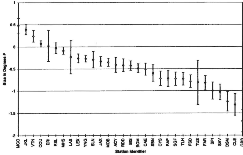
C. Instrument Bias for 4-season stations for Spring
