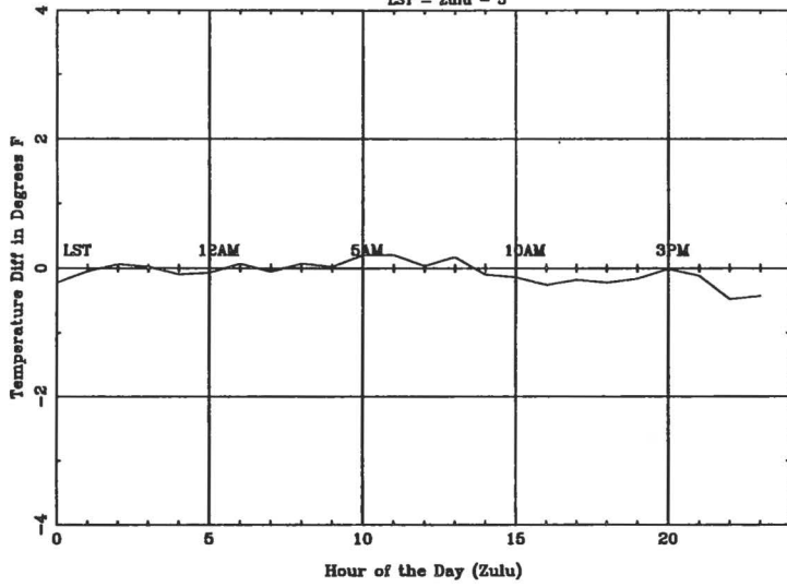
Average Diurnal Cycle for LAN - spring LST = Zulu - 5
