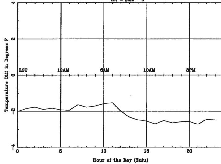
Average Diurnal Cycle for CLE - summer
