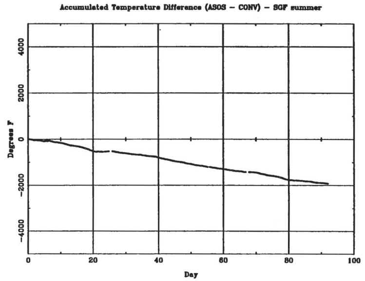
Fig. 3.1 (G) Seasonal accumulated temperature difference plots for Springfield, MO.
