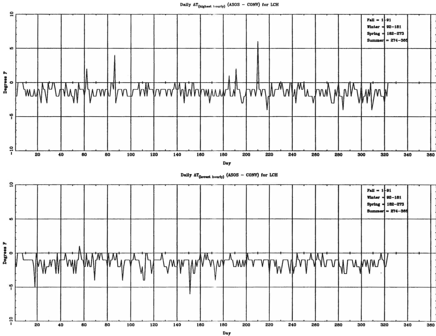
Fig. 3.11 (B) Temperature time series analysis for the coastal site of Lake Charles, LA.
