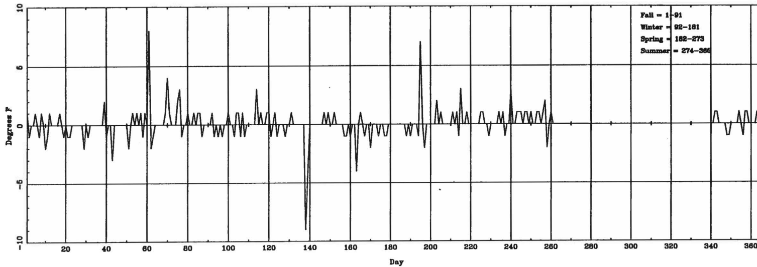
Daily \Delta T_{\text{(lowest hourly)}} (ASOS - CONV) for RST
