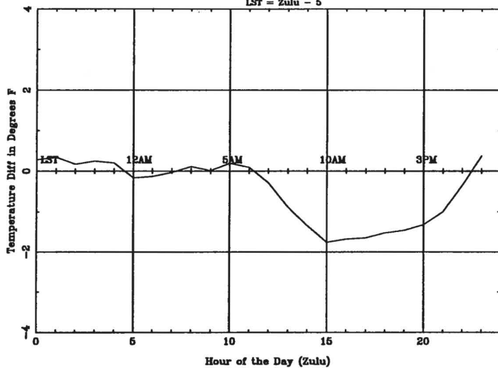
Average Diurnal Cycle for CAE - spring
