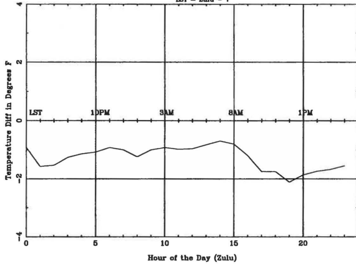
Average Diurnal Cycle for ABQ - spring LST = Zulu - 7
