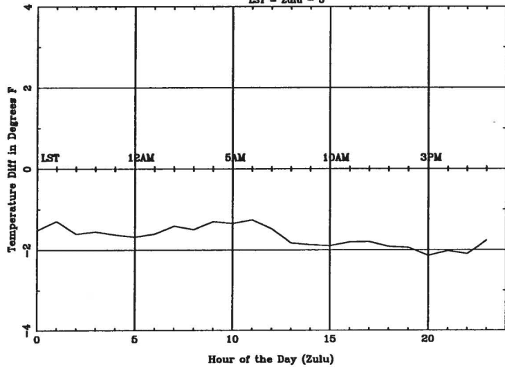
Average Diurnal Cycle for CLE - spring
