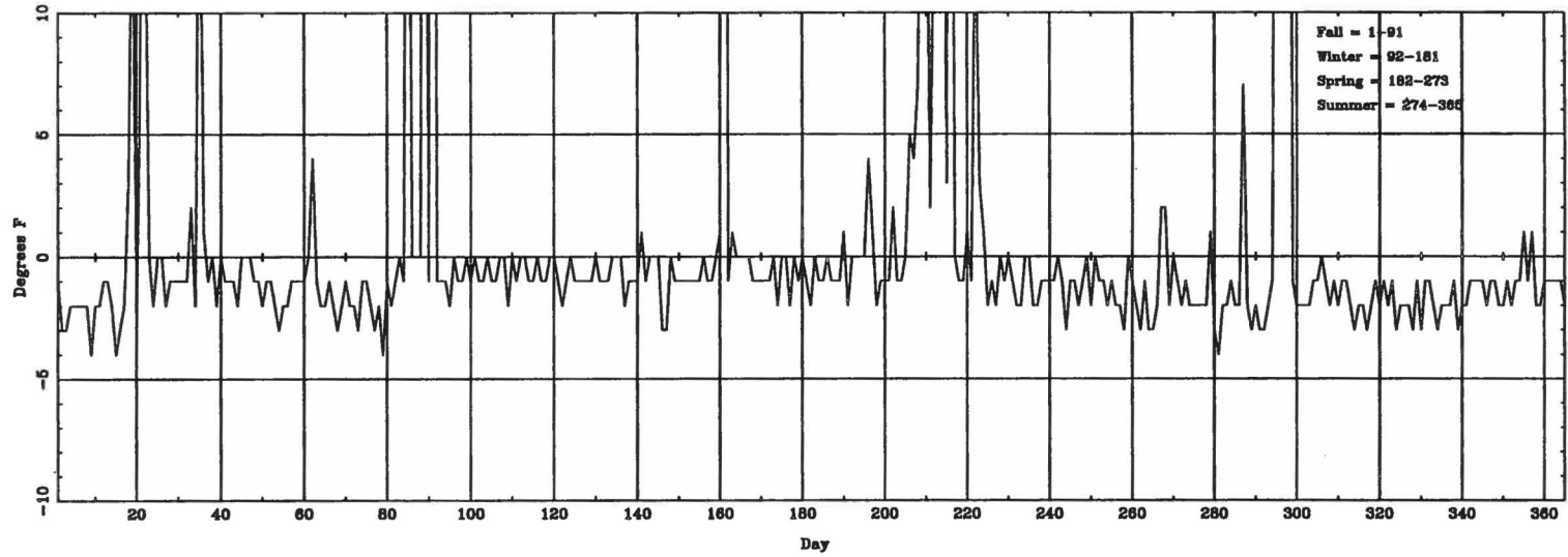
Daily \Delta T_{(\text{lowest hourly})} (ASOS - CONV) for SGF
