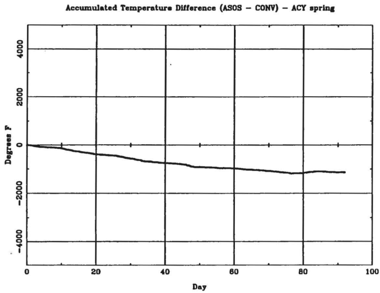
Fig. 3.1 (B) Seasonal accumulated temperature difference plots for Atlantic City, NJ.
