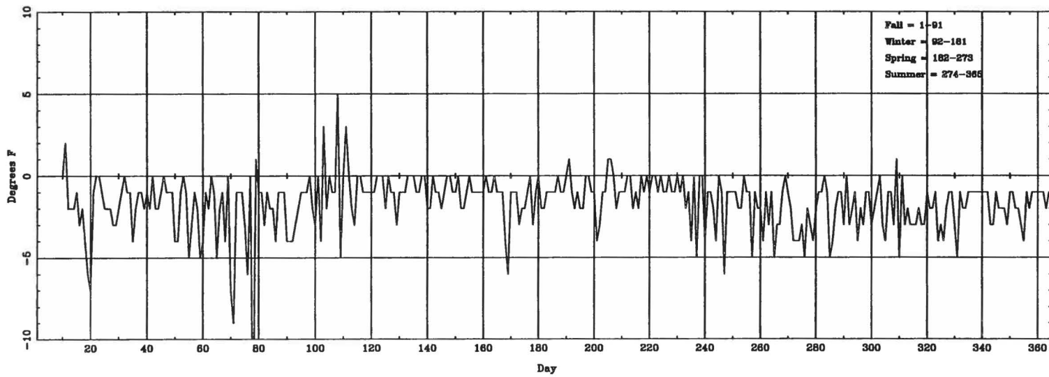
Daily \Delta T_{\text{(lowest hourly)}} (ASOS - CONV) for FSD
