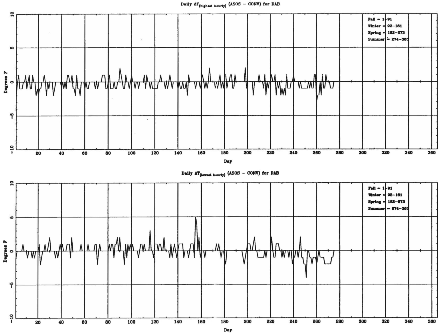
Fig. 3.11 (A) Temperature time series analysis for the coastal site of Daytona Beach, FL.
