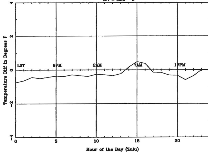
Average Diurnal Cycle for MHS - spring
