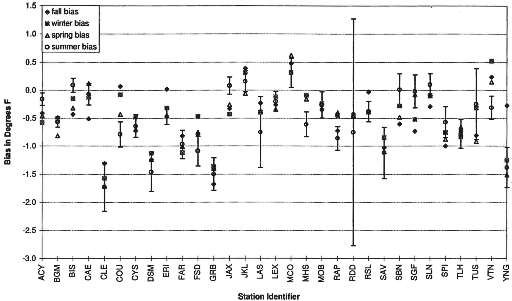
Fig. 3.6 Seasonal instrument biases for four-season stations plotted with summer season 95% confidence intervals.
