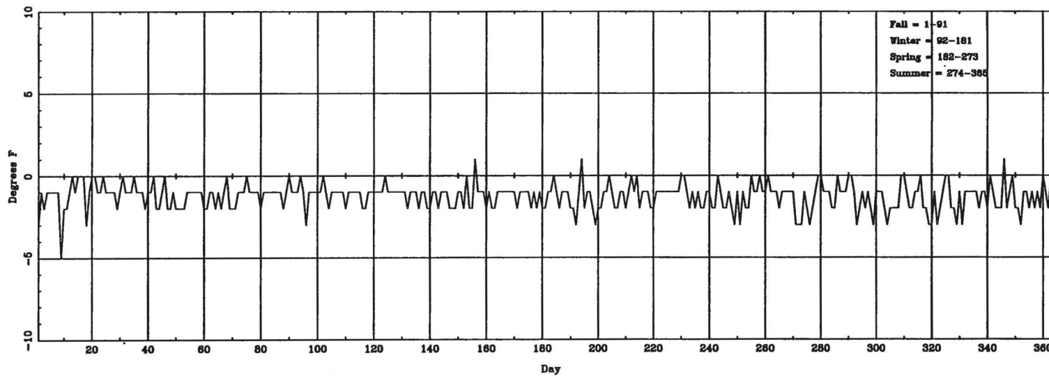
Daily \Delta T_{(lowest\ hourly)} (ASOS - CONV) for TLH
