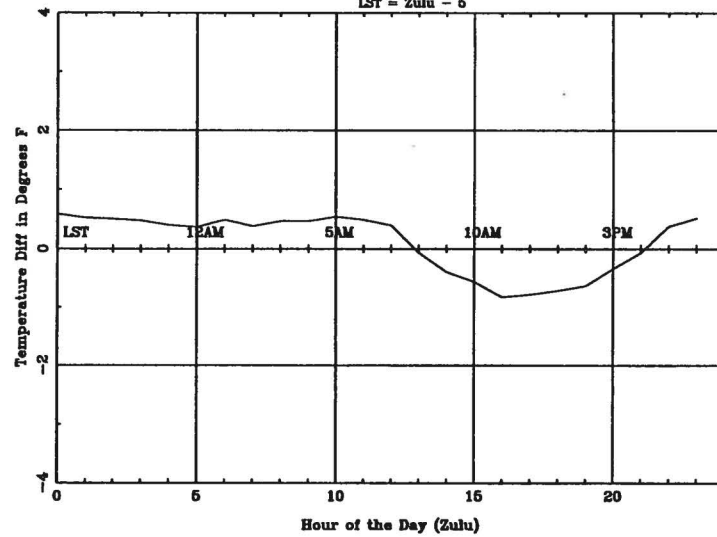
Average Diurnal Cycle for JKL - summer
