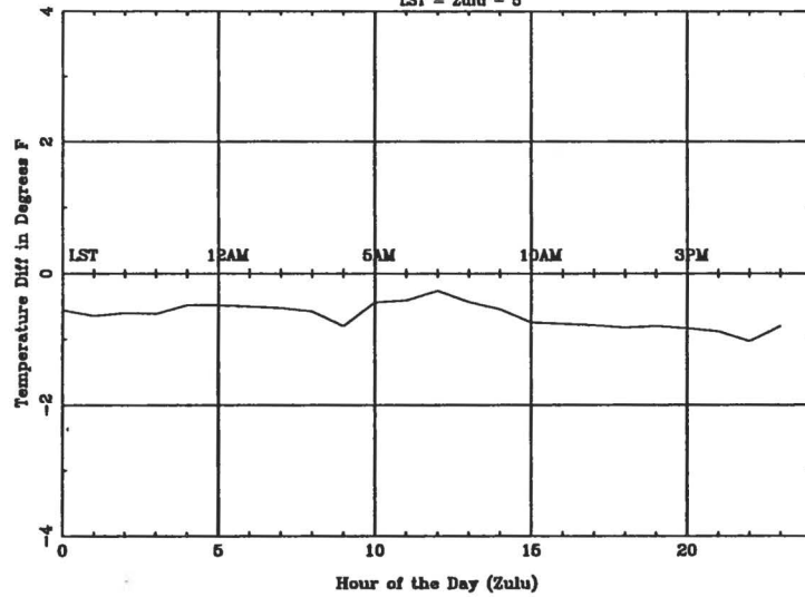
Average Diurnal Cycle for ALB - spring
