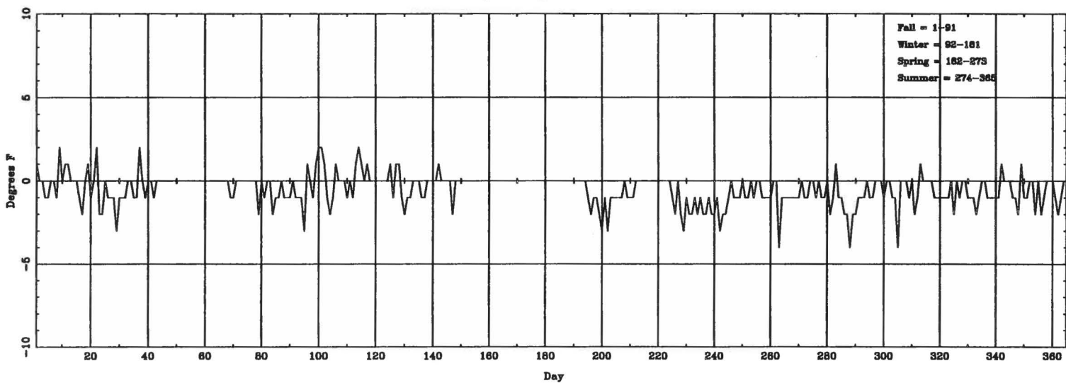
Daily \Delta T_{\text{(lowest hourly)}} (ASOS - CONV) for MSO
