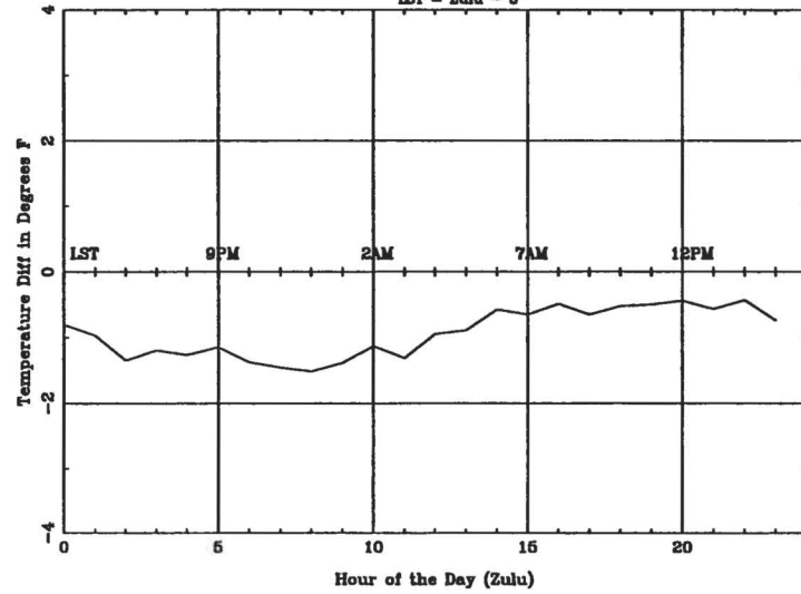
Average Diurnal Cycle for EUG - summer
