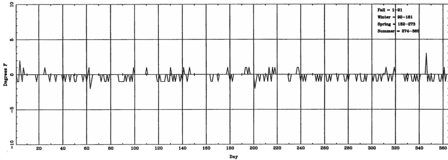
Daily AT_{(lowest\ hourly)} (ASOS - CONV) for MOB
