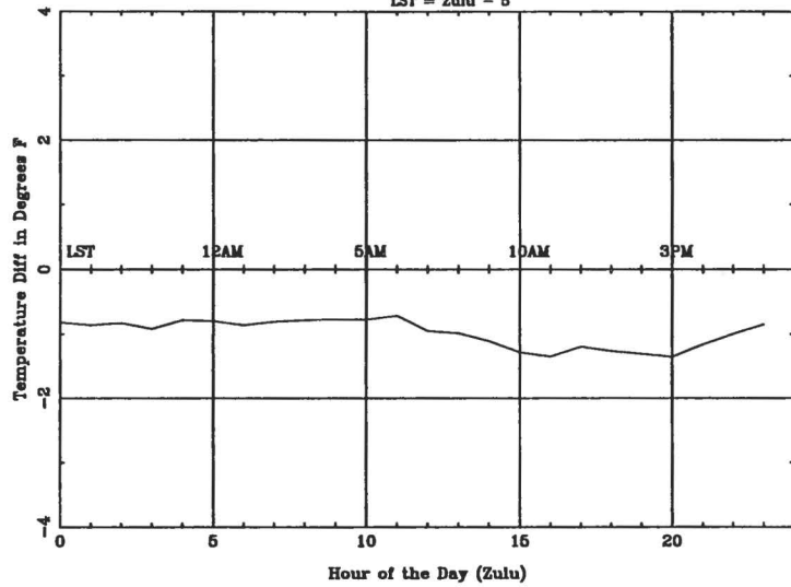
Average Diurnal Cycle for DTW - spring LST = Zulu - 5
