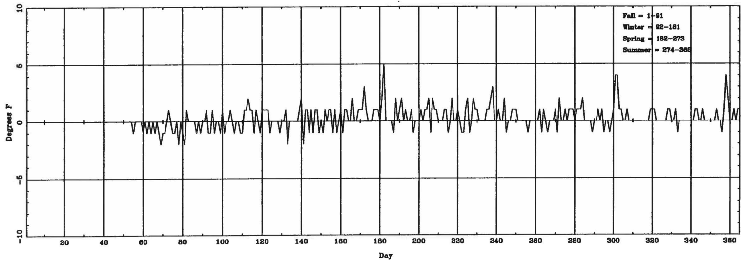
Daily \Delta T_{(lowest\ hourly)} (ASOS - CONV) for PDX
