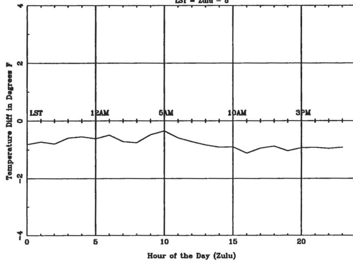
Average Diurnal Cycle for ALB - spring
