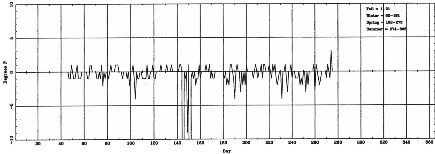
Daily \Delta T_{\text{(lowest hourly)}} (ASOS - CONV) for FNT
