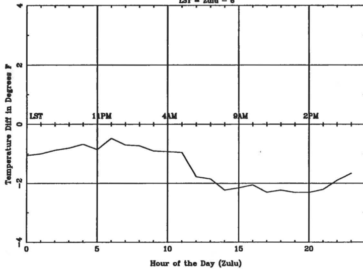
Average Diurnal Cycle for MSN - spring
