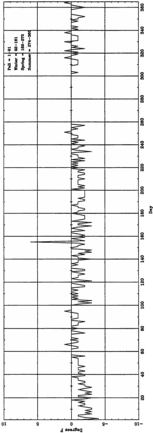
Daily \Delta T_{(high\text{-}hourly)} (ASOS - CONV) for PIA
