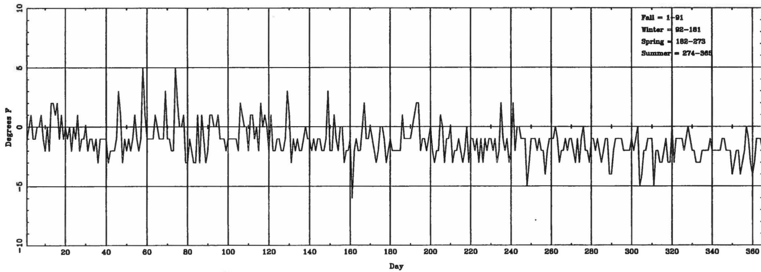
Daily \Delta T_{(lowest\ hourly)} (ASOS - CONV) for CLE
