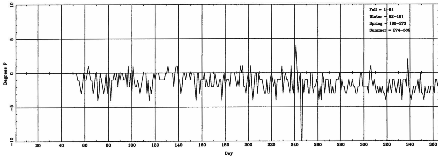
Daily \Delta T_{\text{(lowest hourly)}} (ASOS - CONV) for LBB
