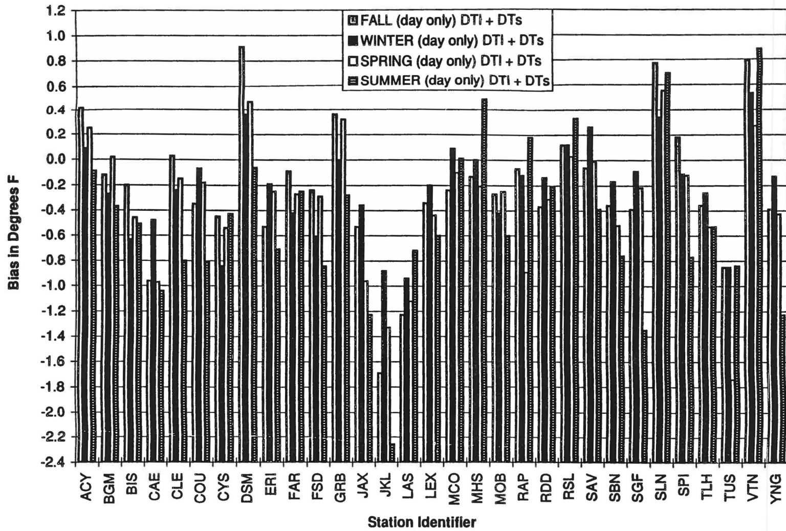
Fig. 3.9 (A) Seasonal distribution of daytime local and solar effects for four-season stations.
