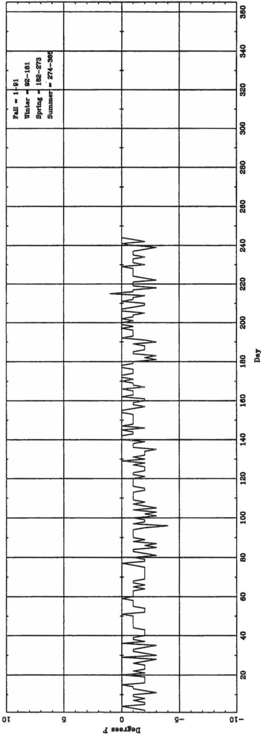
Daily \Delta T_{(light\ hour)} (ASOS - CONV) for BIL
