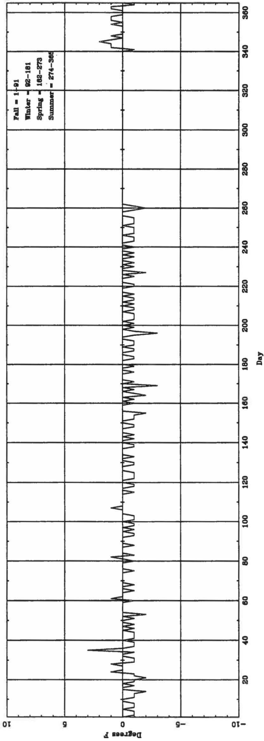
Daily \Delta T (lightest hourly) (ASOS - CONY) for MKG
