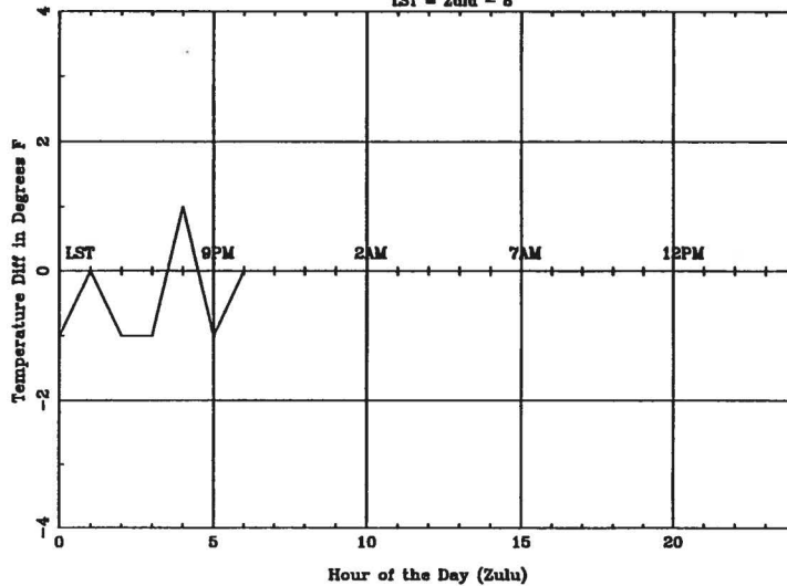
Average Diurnal Cycle for PDT - summer
