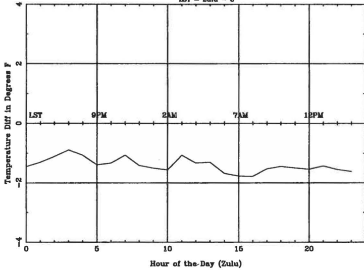
Average Diurnal Cycle for DRA - spring LST = Zulu - 8
