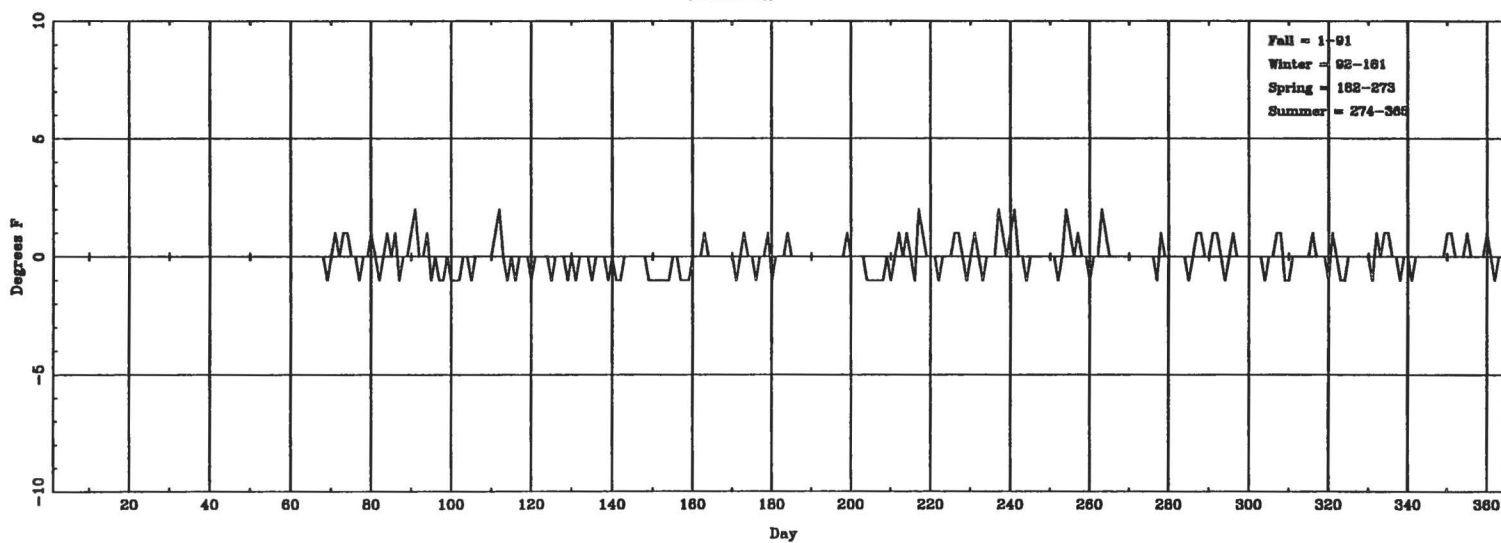
Daily \Delta T_{(lowest\ hourly)} (ASOS - CONV) for DAY
