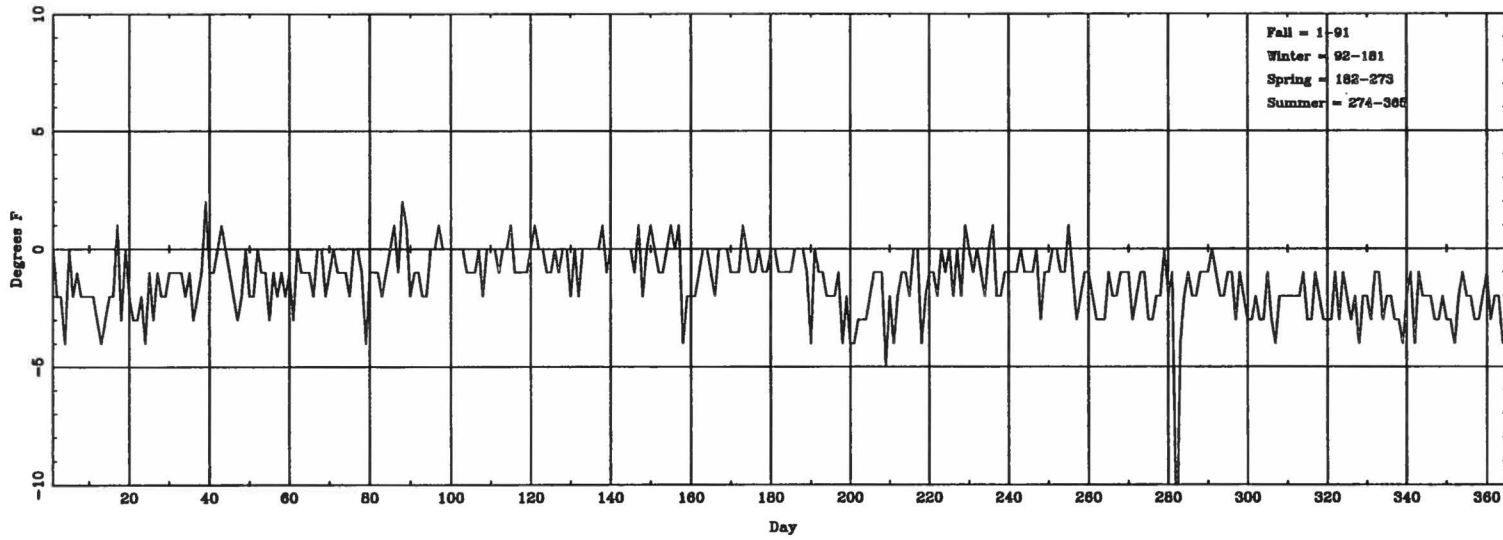
Daily \Delta T_{\text{(lowest hourly)}} (ASOS - CONV) for JKL
