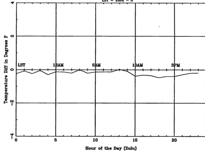
Average Diurnal Cycle for MKG - summer LST = Zulu - 5
