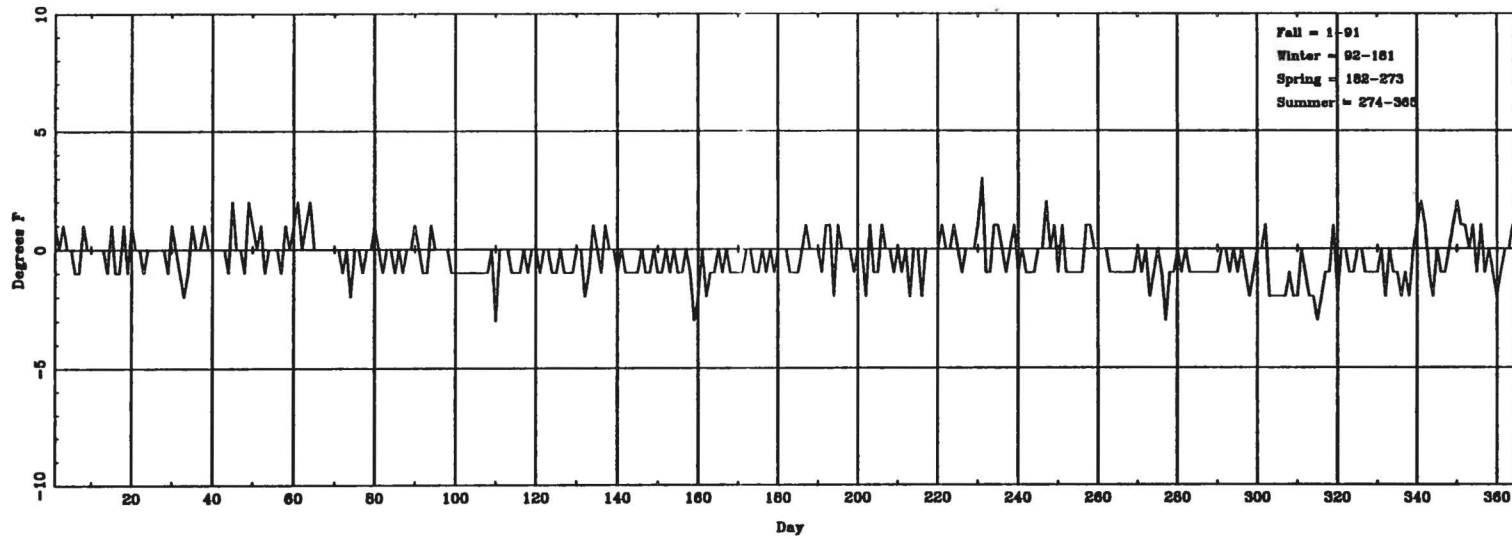
Daily \Delta T_{\text{(lowest hourly)}} (ASOS - CONV) for ACY
