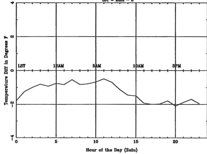
Average Diurnal Cycle for FWA - summer LST = Zulu - 5
