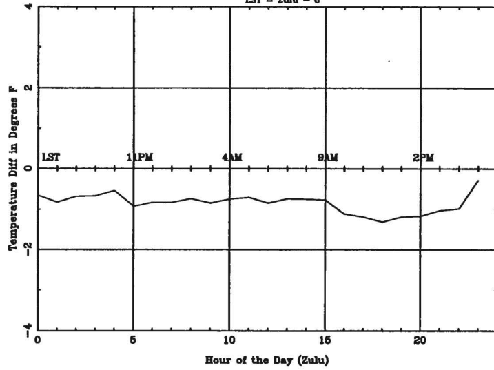
Average Diurnal Cycle for FSD - summer
