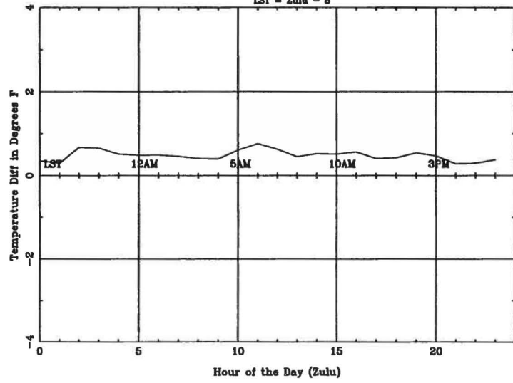
Average Diurnal Cycle for LAN - summer LST = Zulu - 5
