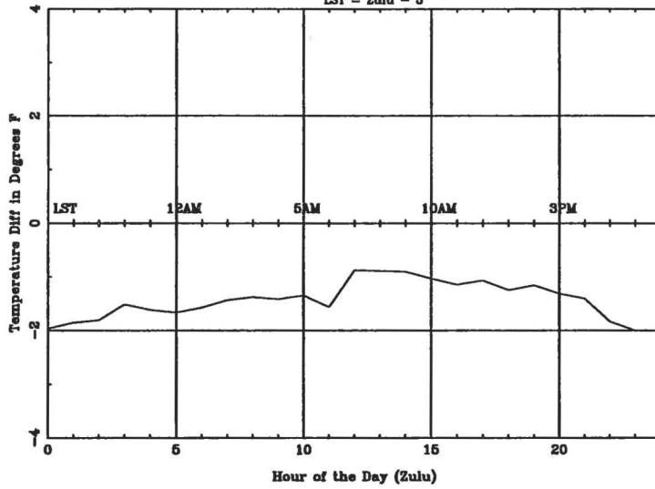
Average Diurnal Cycle for FWA - spring LST = Zulu - 5
