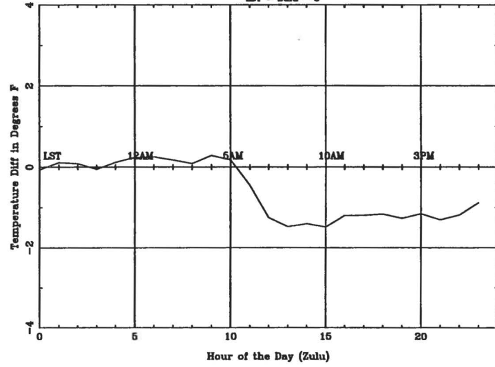
Average Diurnal Cycle for TLH - summer LST = Zulu - 5
