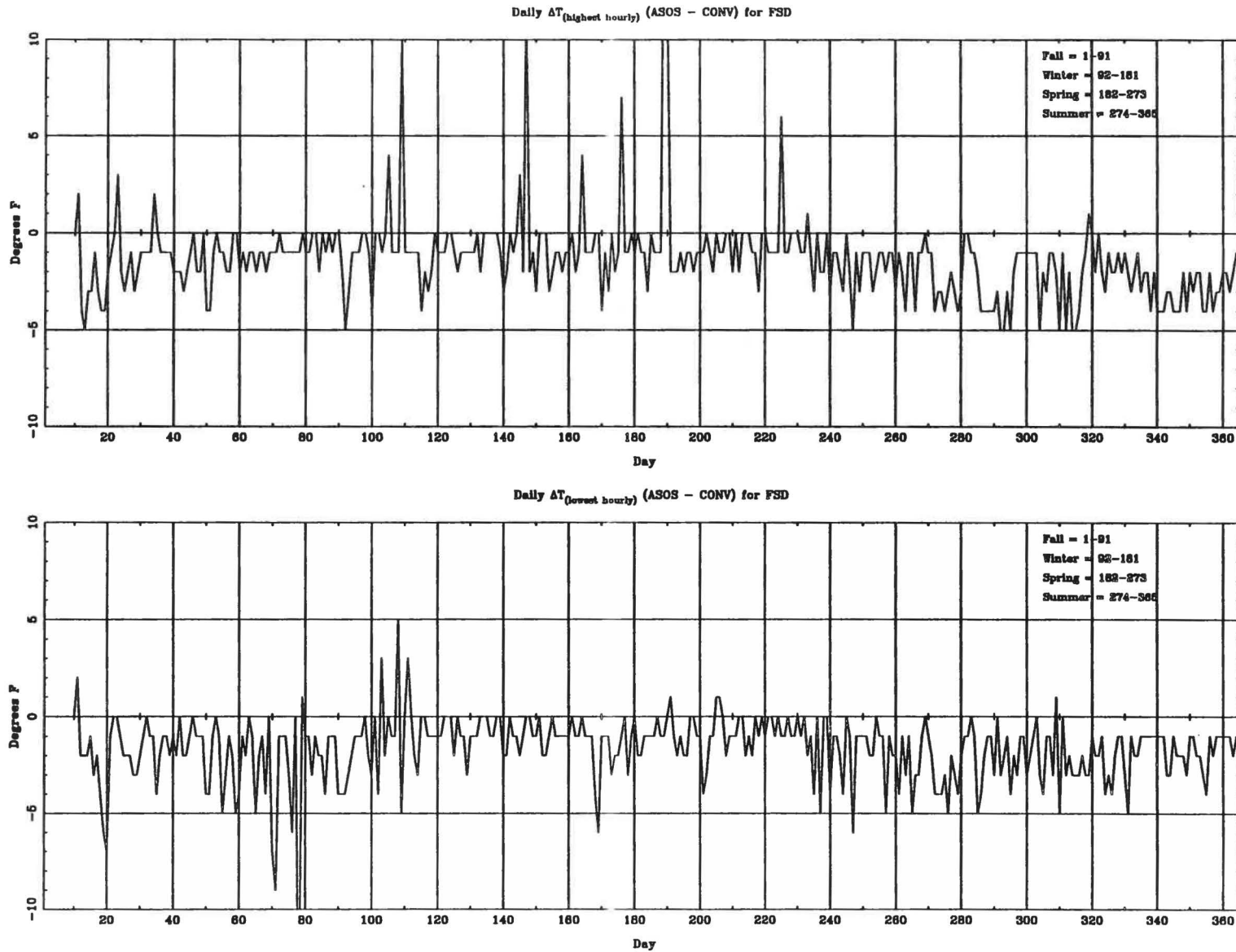
Fig. 3.11 (C) Temperature time series analysis for the continental site of Sioux Falls, SD.
