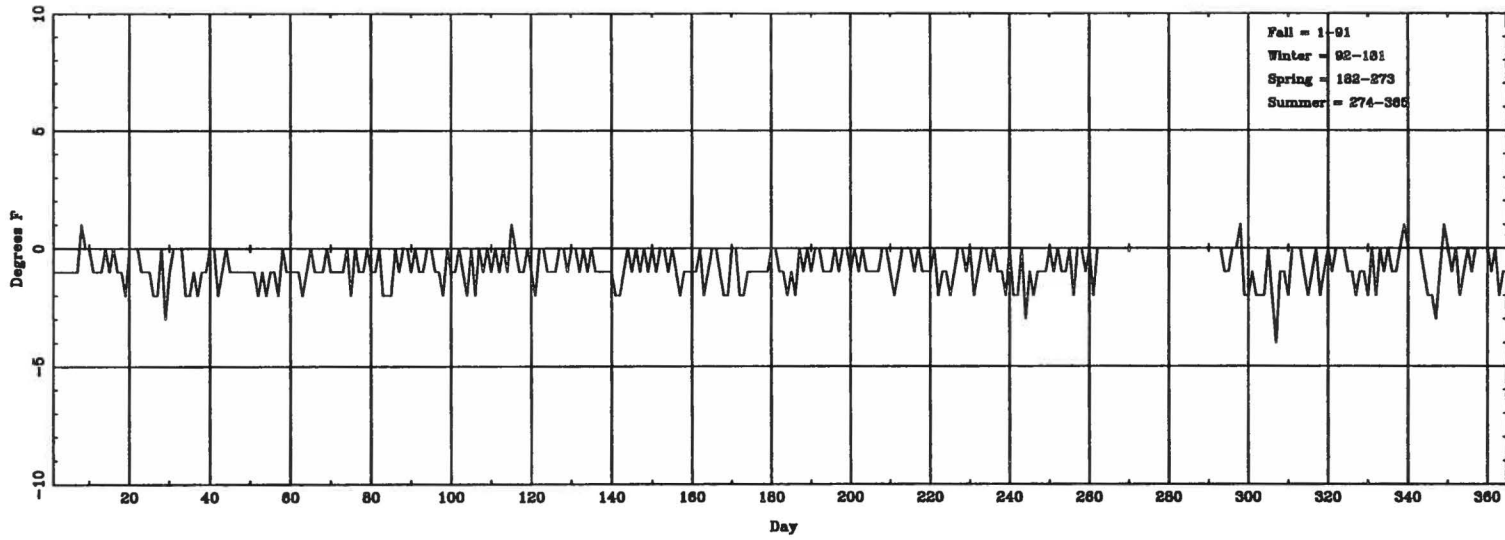
Daily \Delta T_{\text{(lowest hourly)}} (ASOS - CONV) for RDD
