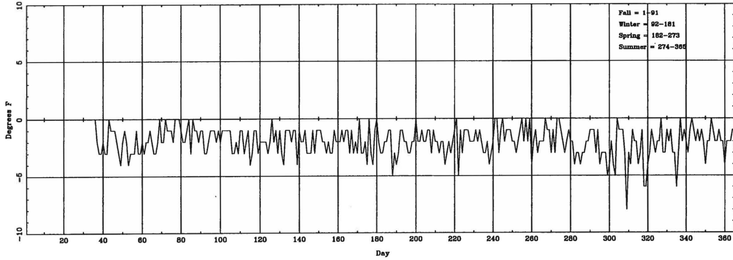
Daily \Delta T_{(lowest\ hourly)} (ASOS - CONV) for ABQ
