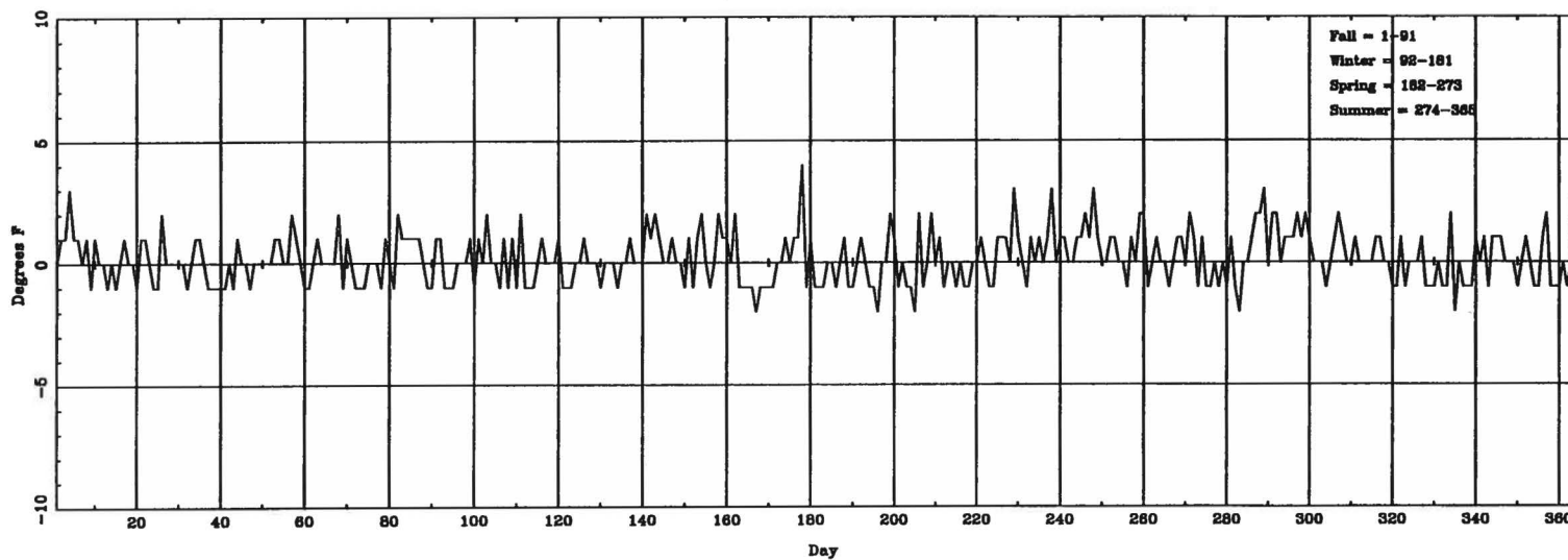
Daily \Delta T_{(lowest\ hourly)} (ASOS - CONV) for TLH
