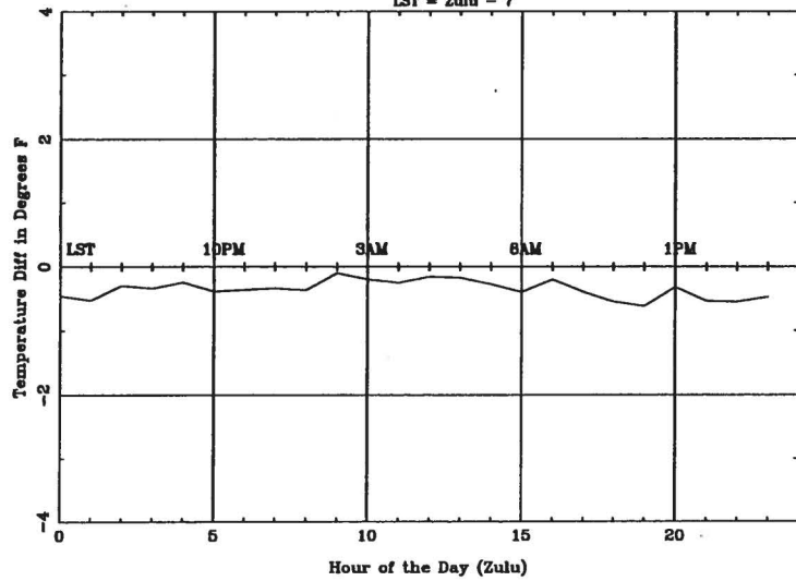
Average Diurnal Cycle for BFF - spring
