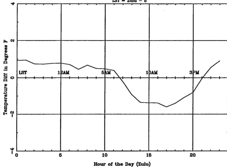
Average Diurnal Cycle for JKL - spring
