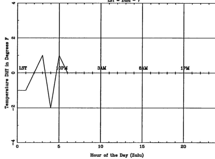
Average Diurnal Cycle for BFF - summer
