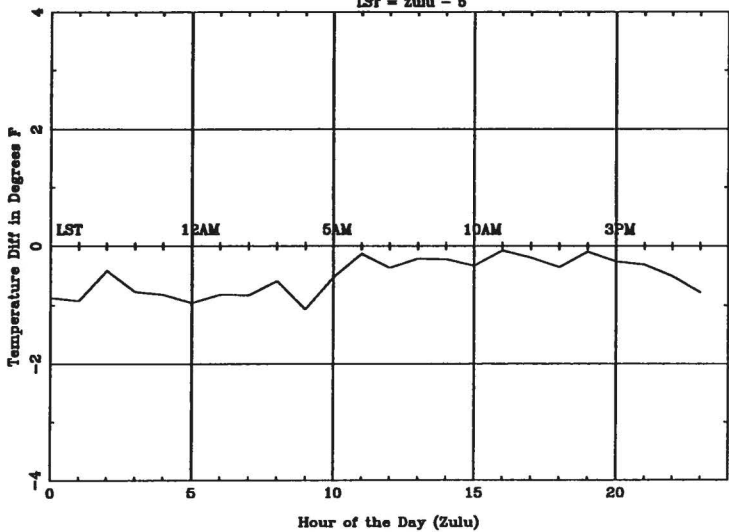
Average Diurnal Cycle for ACY - spring LST = Zulu - 5
