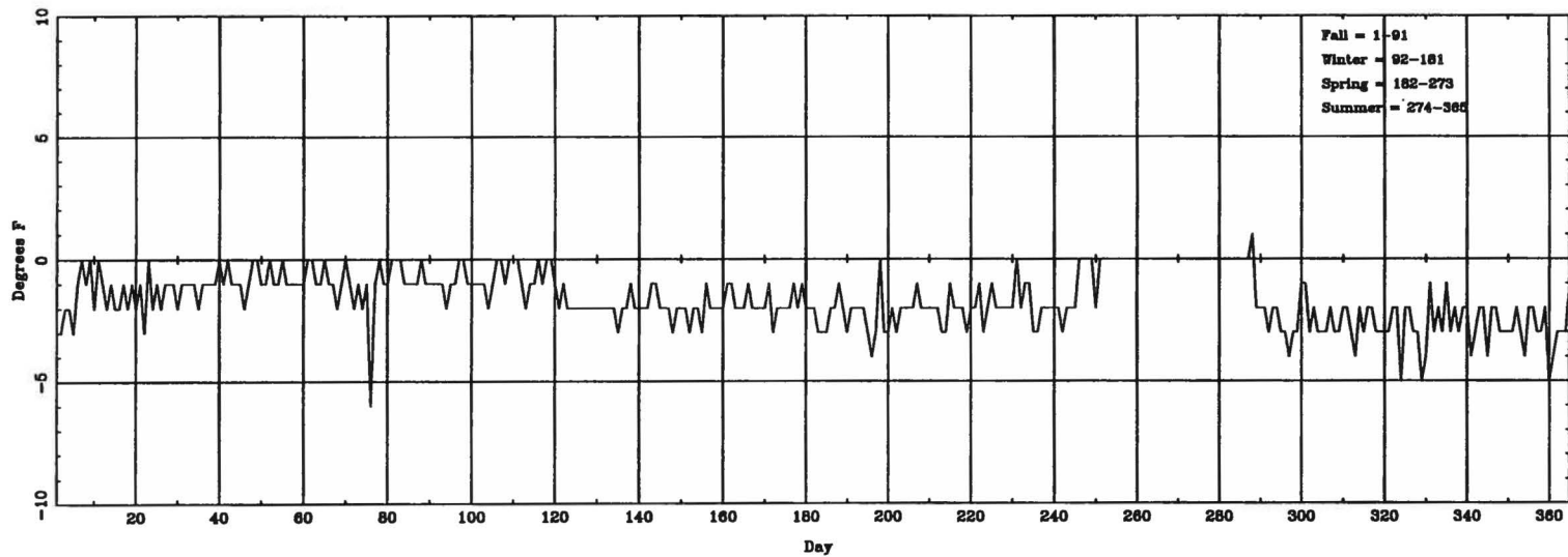
Daily \Delta T_{(lowest\ hourly)} (ASOS - CONV) for YNG
