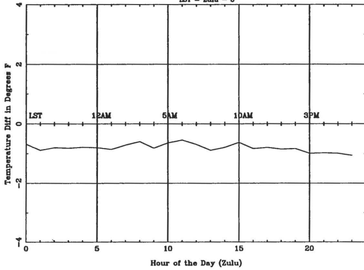
Average Diurnal Cycle for BGM - spring LST = Zulu - 5
