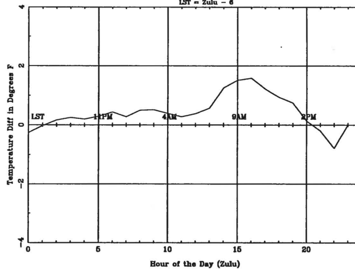
Average Diurnal Cycle for VTN - summer
