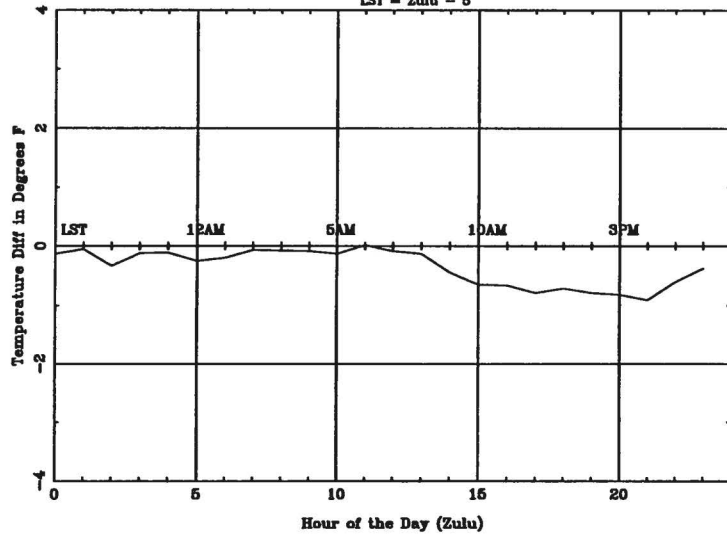
Average Diurnal Cycle for LEK - spring LST = Zulu - 5
