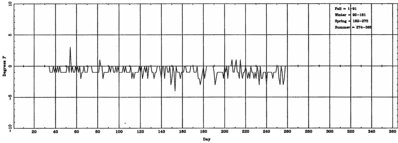
Daily AT (lowest hourly) (ASOS - CONV) for ISN
