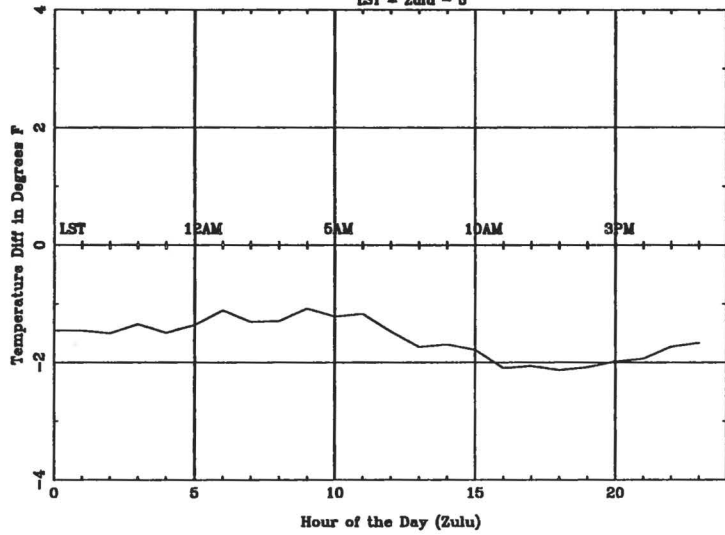
Average Diurnal Cycle for YNG - spring LST = Zulu - 5
