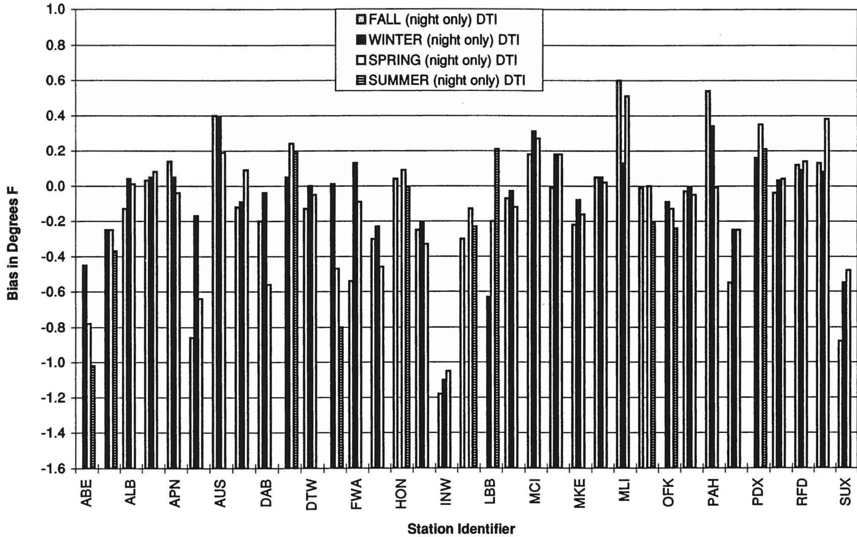
Fig. 3.8 (B) Seasonal distribution of nighttime local effects for three-season stations.
