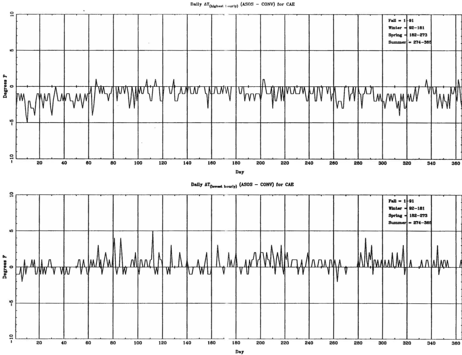
Fig. 3.10 (B) Temperature time series analysis for Columbia, SC.
