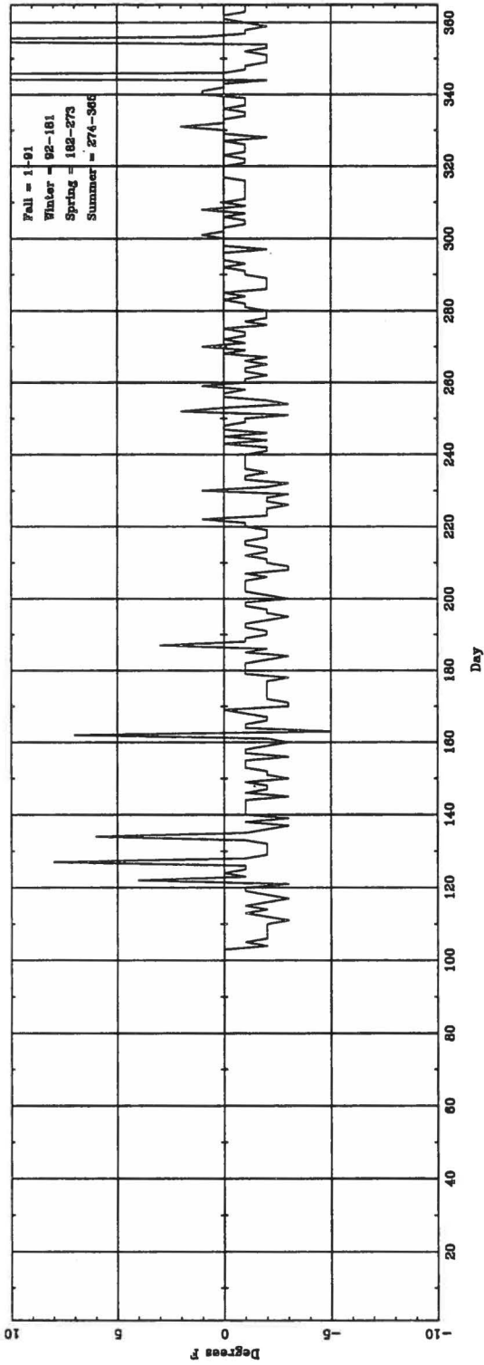
Daily AT (light hourly) (ASOS - CONV) for ABE
