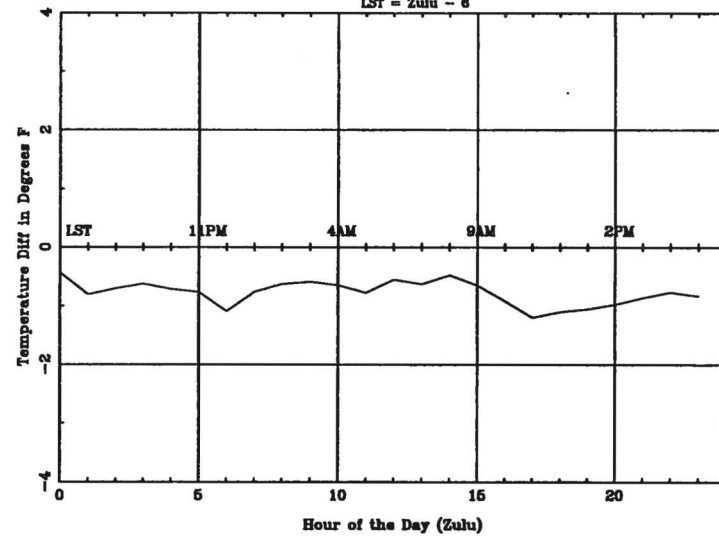
Average Diurnal Cycle for INL - summer
