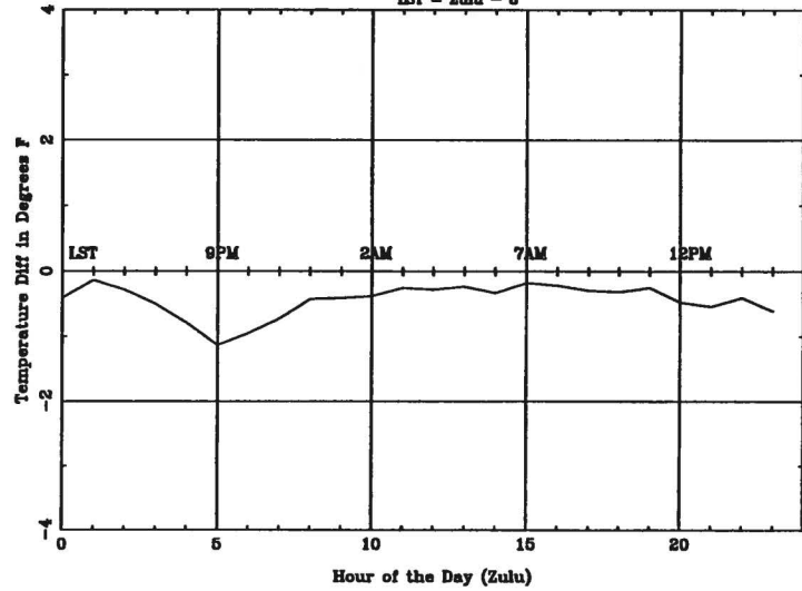
Average Diurnal Cycle for GEG - summer
