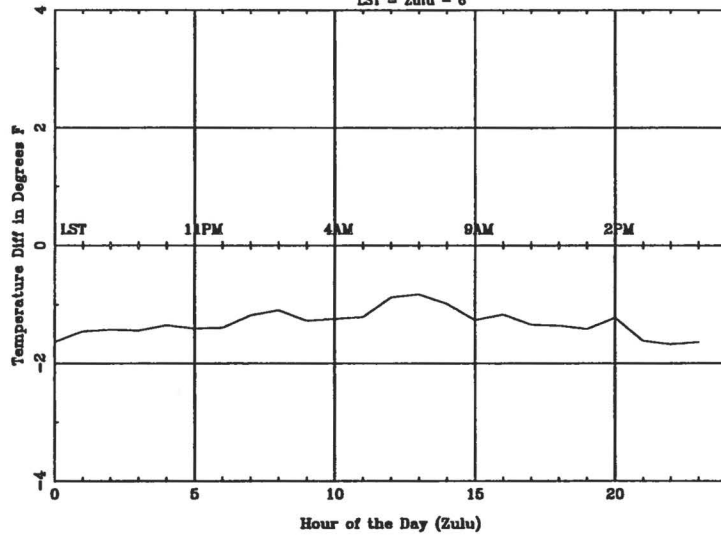
Average Diurnal Cycle for LCH - spring
