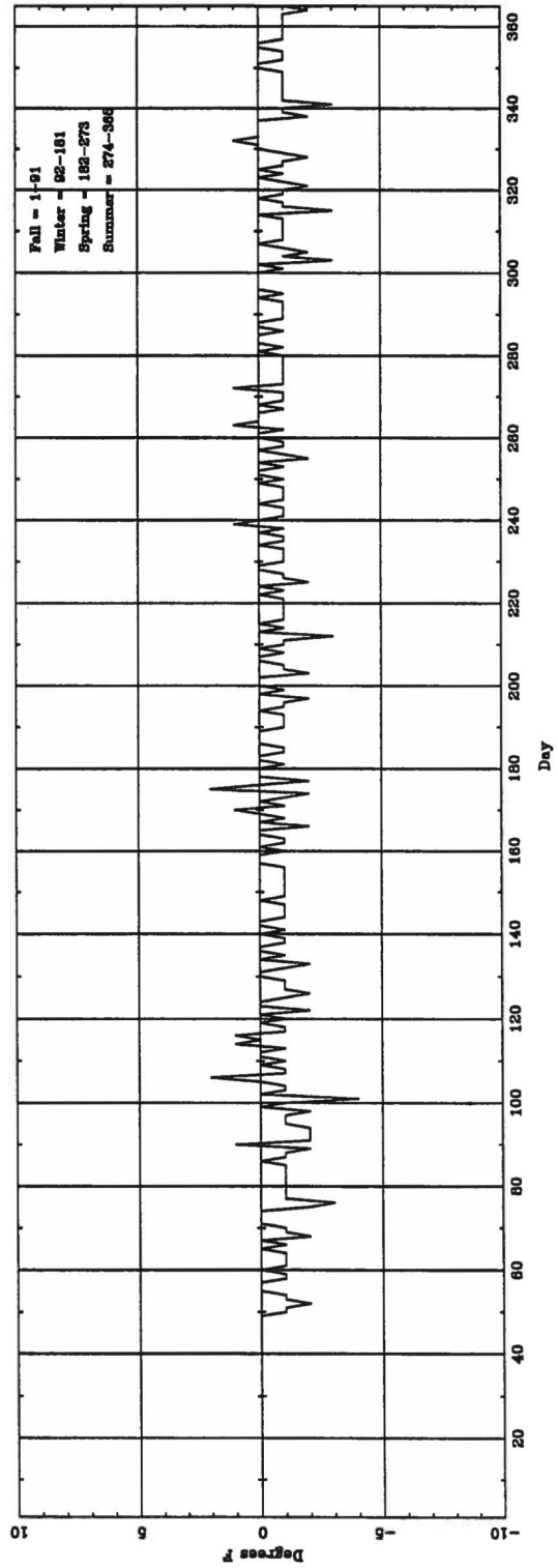
Daily \Delta T (current hourly) (ASOS - CONV) for OFK
