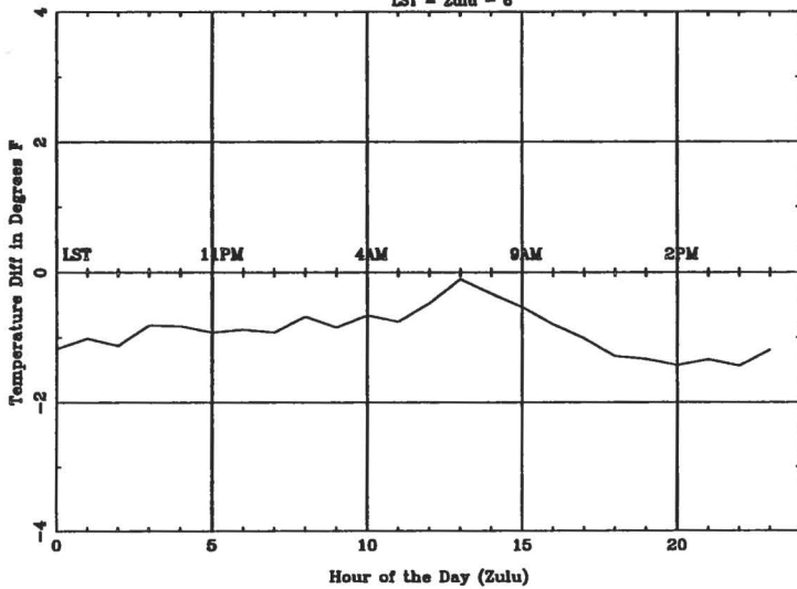
Average Diurnal Cycle for LBB - spring LST = Zulu - 6
