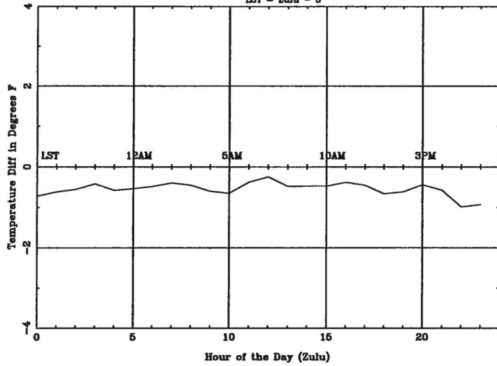
Average Diurnal Cycle for ERI - spring LST = Zulu - 6
