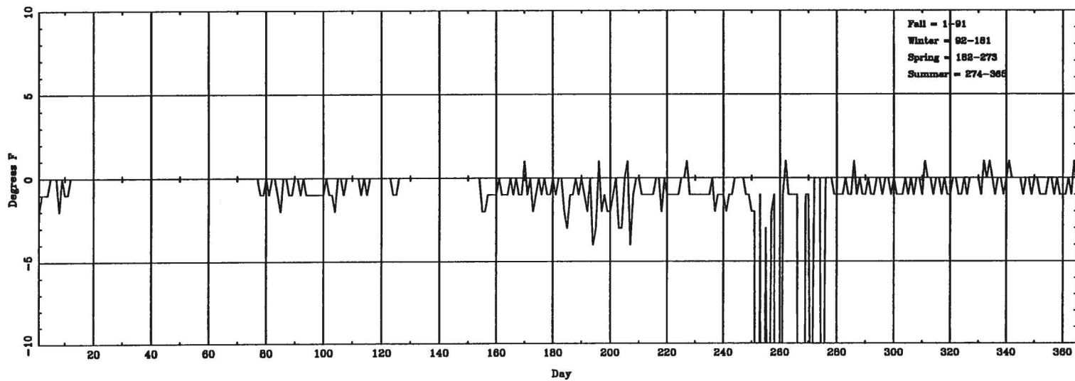
Daily \Delta T_{(\text{lowest hourly})} (ASOS - CONV) for CAK
