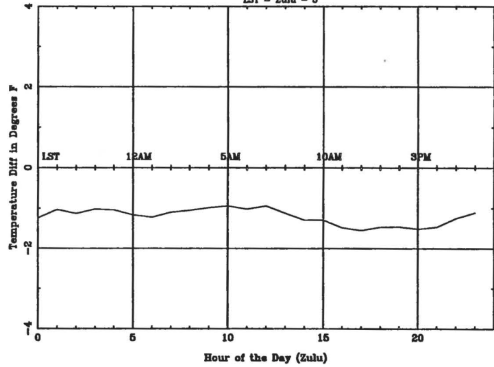
Average Diurnal Cycle for YNG - summer LST = Zulu - 5
