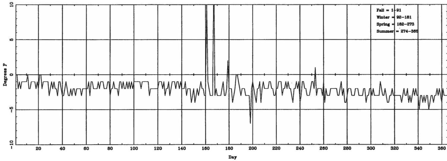
Daily \Delta T_{(lowest\ hourly)} (ASOS - CONV) for CLE
