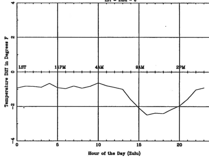
Average Diurnal Cycle for MSN - summer
