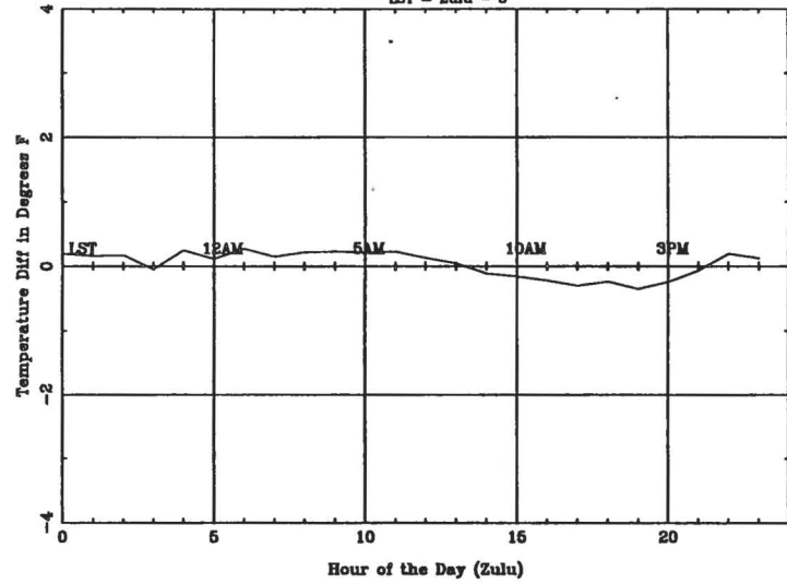
Average Diurnal Cycle for FNT - summer LST = Zulu - 6
