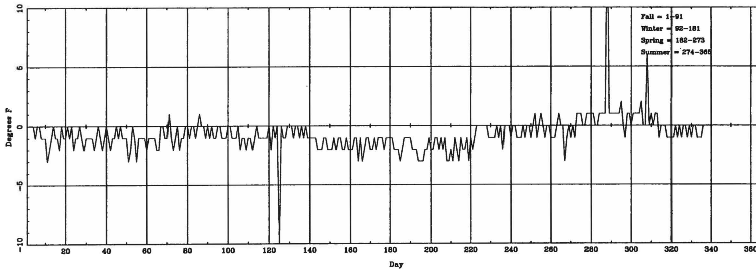
Daily \Delta T_{(lowest\ hourly)} (ASOS - CONV) for ALB
