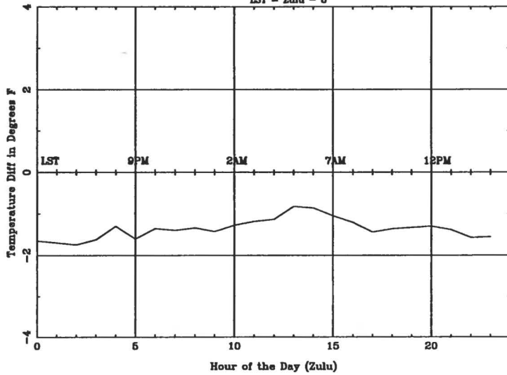
Average Diurnal Cycle for EUG - spring
