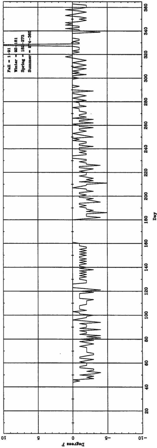
Daily \Delta T_{(night\ hour)} (ASOS - CONV) for EUG
