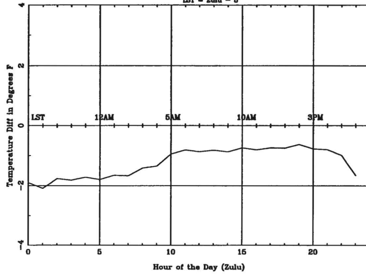
Average Diurnal Cycle for ABE - summer LST = Zulu - 5
