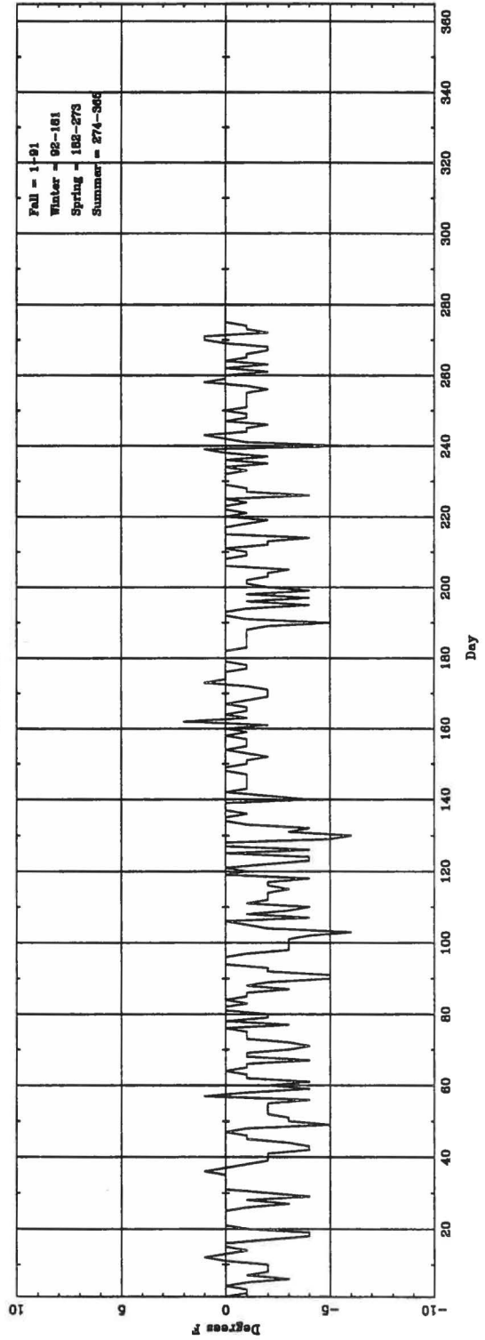
Daily \Delta T_{(low\text{-}w\text{-}h\text{-}h)} (ASOS - CONV) for SUX
