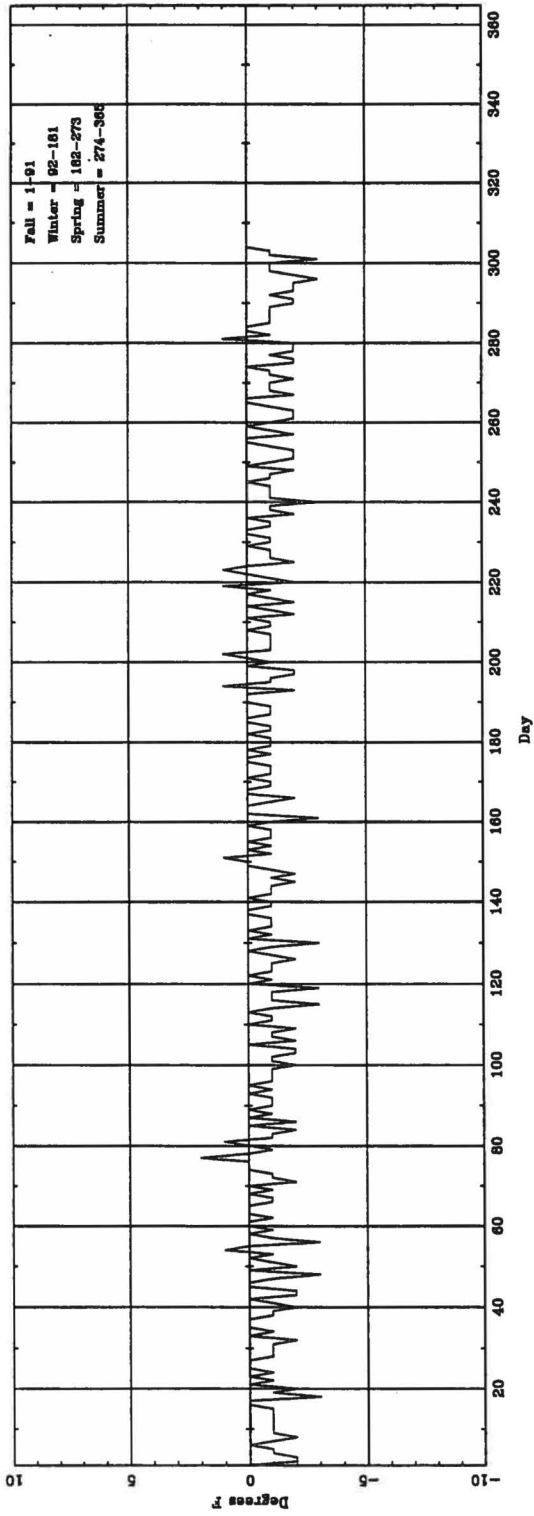
Daily \Delta T_{\text{(highest hourly)}} (ASOS - CONV) for MCI
