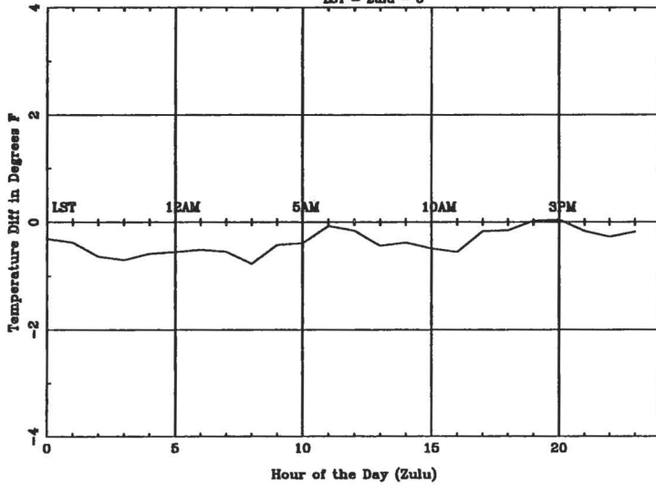
Average Diurnal Cycle for DAB - spring
