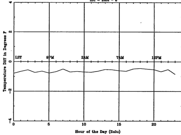
Average Diurnal Cycle for GEG - summer
