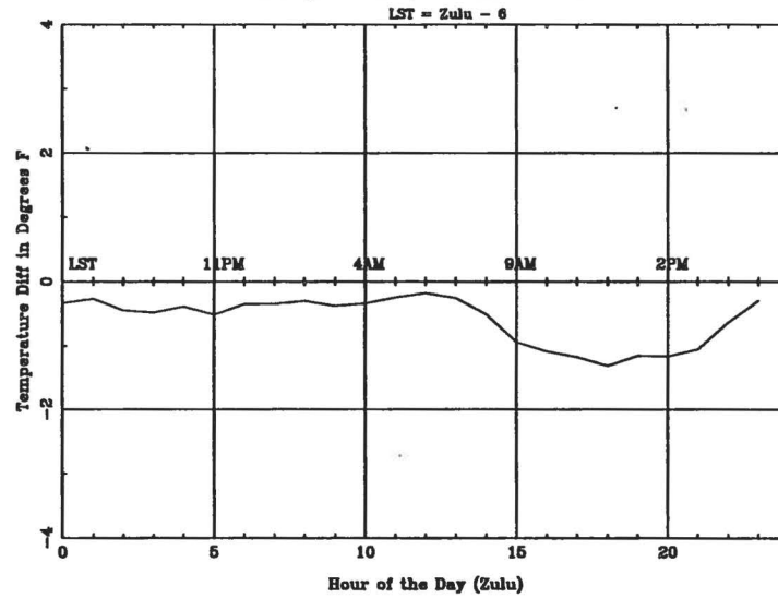
Average Diurnal Cycle for MLI - summer
