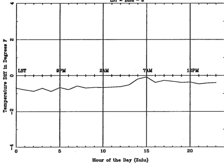
Average Diurnal Cycle for PDT - spring
