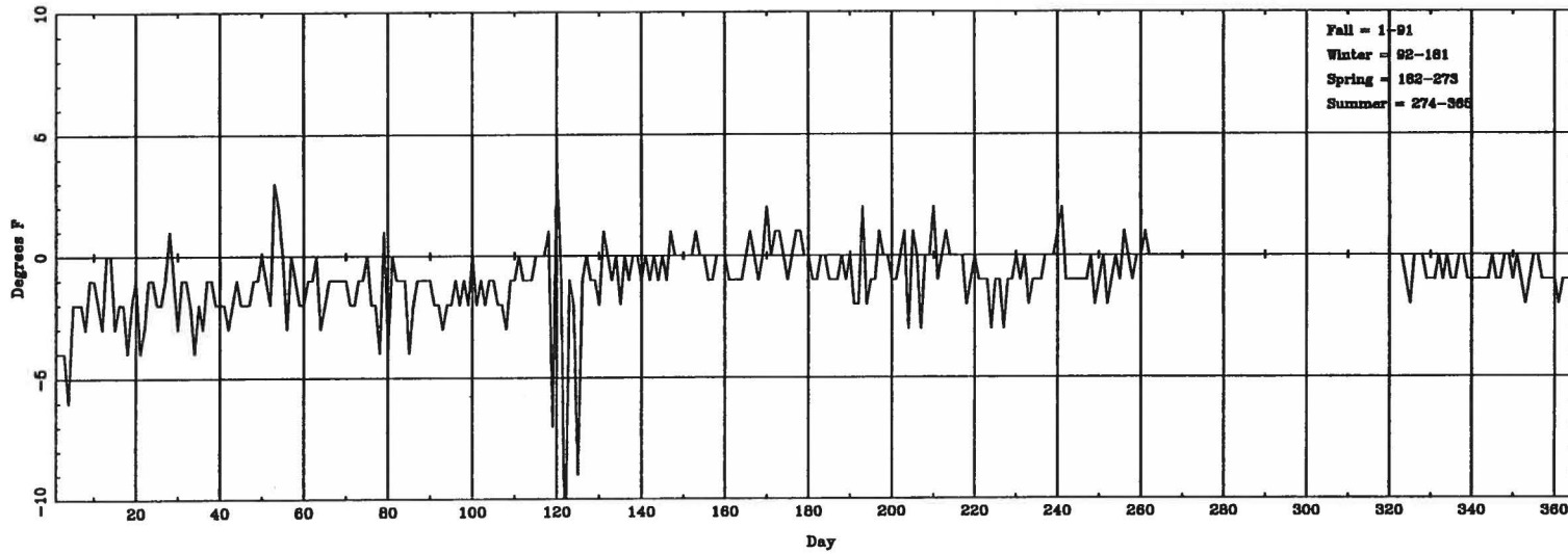
Daily \Delta T_{(lowest\ hourly)} (ASOS - CONV) for FWA
