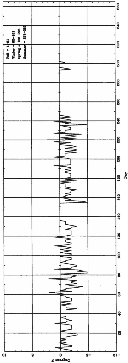
Daily \Delta T_{(prewet\ hour)} (ASOS - CONV) for MGM
