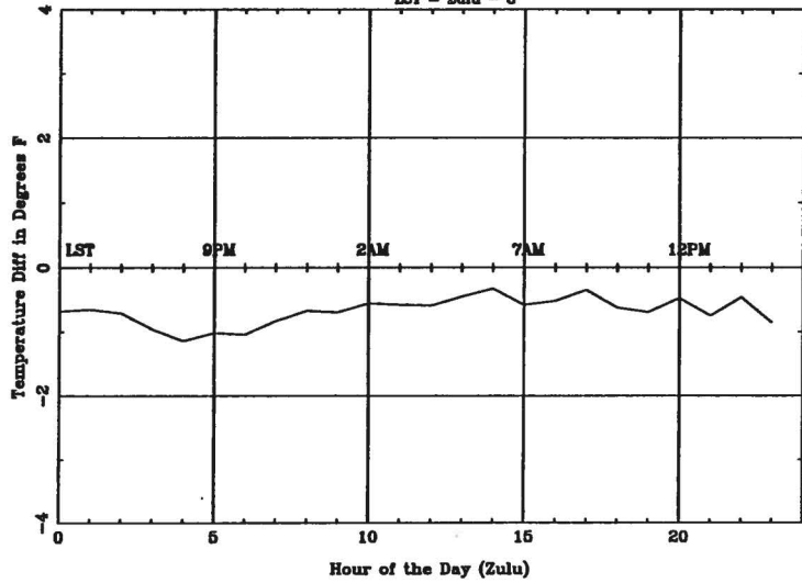
Average Diurnal Cycle for GEG - spring
