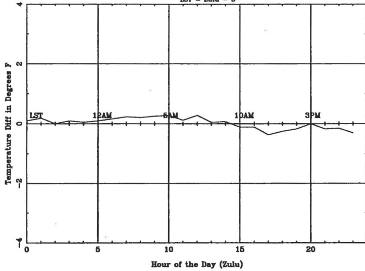
Average Diurnal Cycle for FNT - spring LST = Zulu - 6
