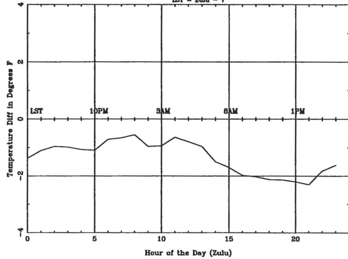
Average Diurnal Cycle for ABQ - summer LST = Zulu - 7
