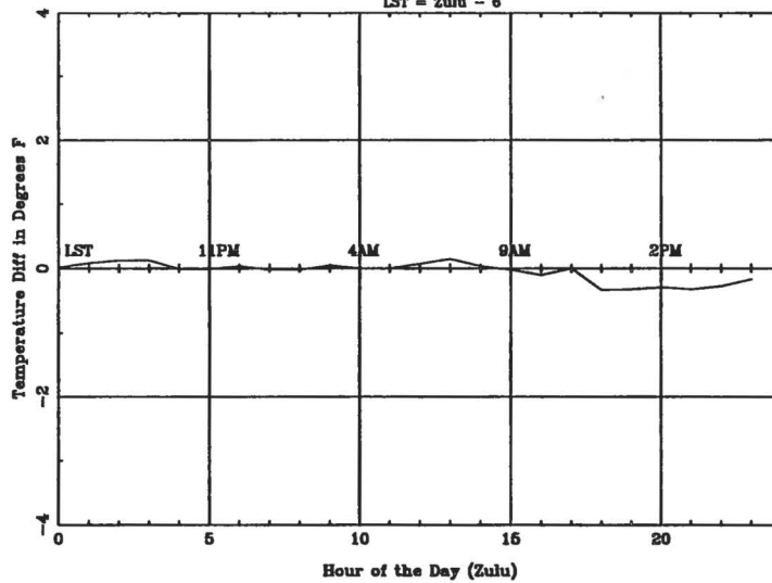
Average Diurnal Cycle for COU - summer
