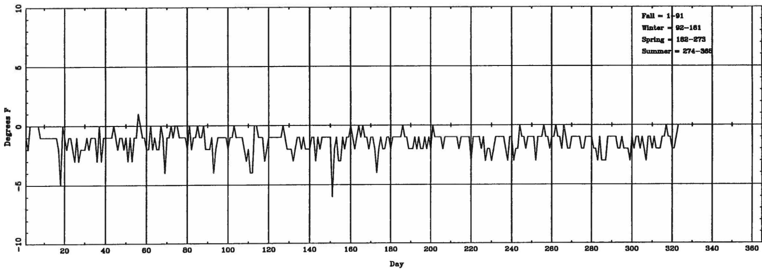
Daily \Delta T_{(lowest\ hourly)} (ASOS - CONV) for LCH
