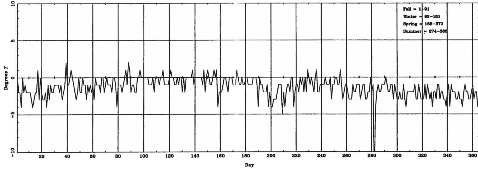
Daily \Delta T_{(lowest\ hourly)} (ASOS - CONV) for JKL
