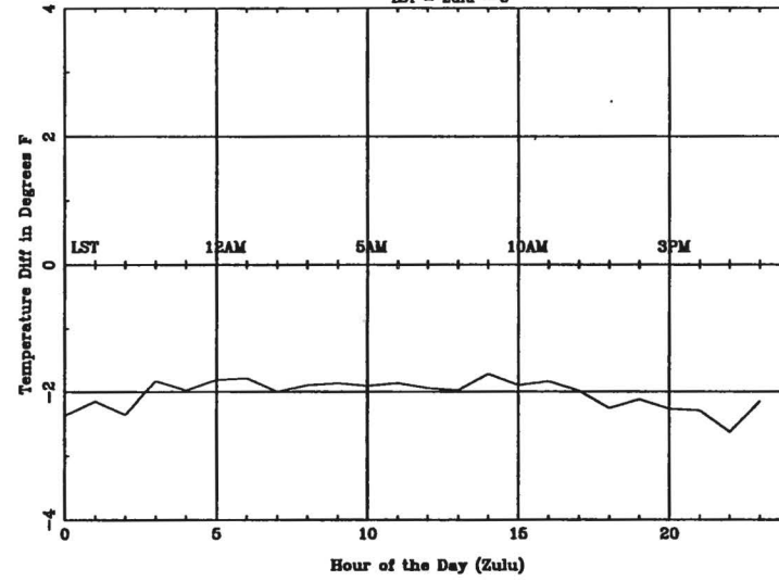
Average Diurnal Cycle for ATL - summer
