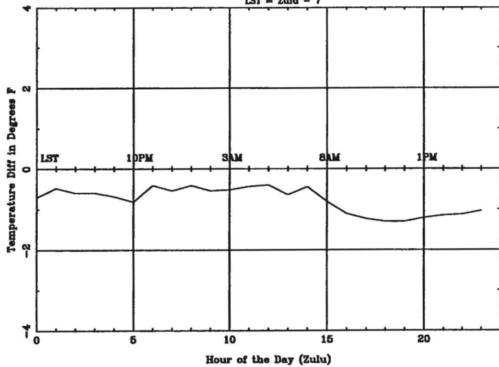
Average Diurnal Cycle for CYS - spring LST = Zulu - 7
