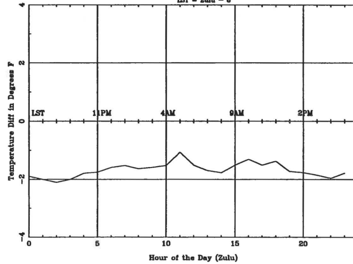
Average Diurnal Cycle for LCH - summer
