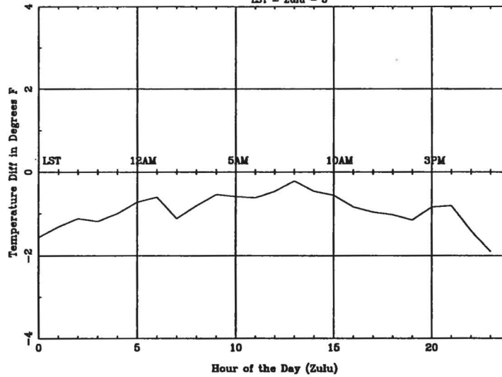
Average Diurnal Cycle for TRI - summer
