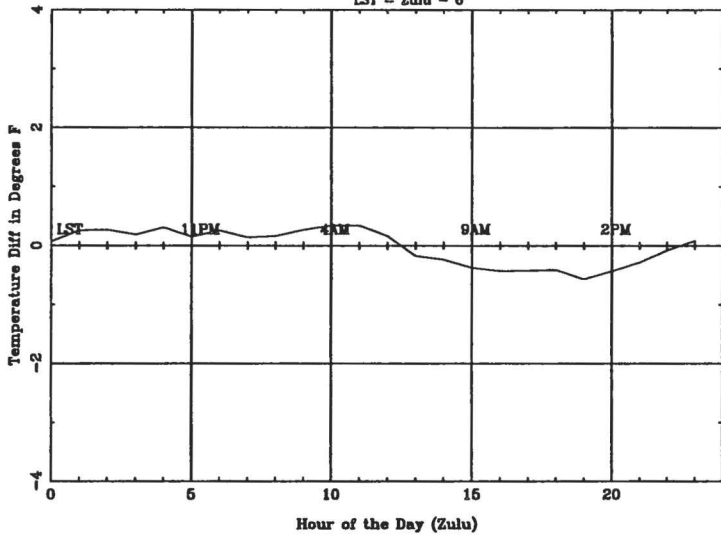
Average Diurnal Cycle for RFD - spring LST = Zulu - 6
