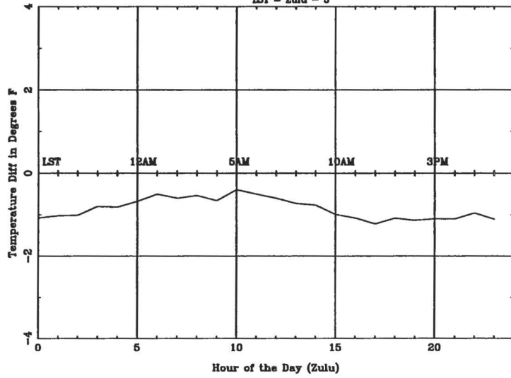
Average Diurnal Cycle for SBN - spring LST = Zulu - 5
