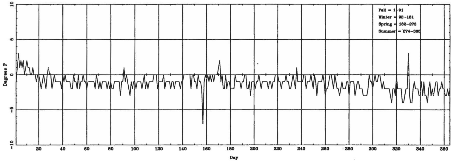
Daily \Delta T (lowest hourly) (ASOS - CONV) for DSM
