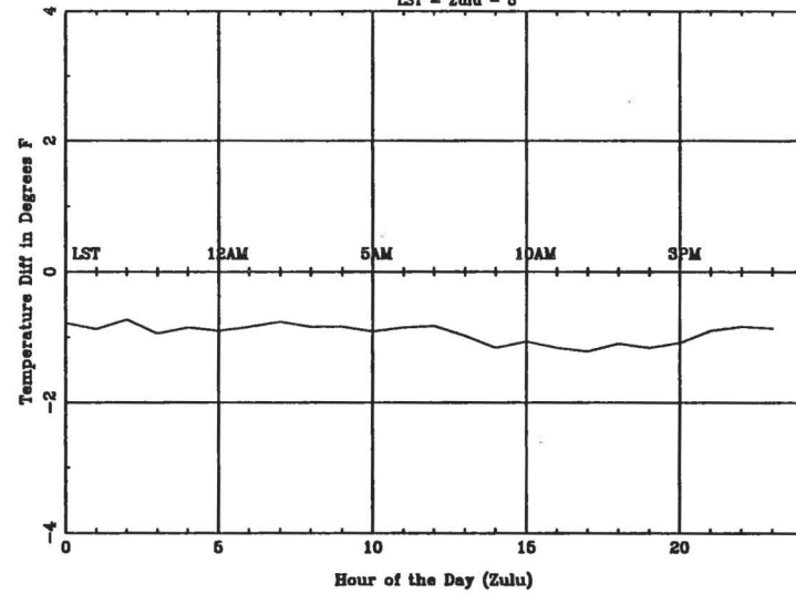
Average Diurnal Cycle for ALB - summer
