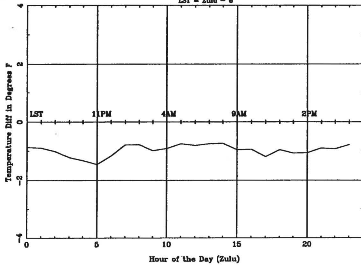
Average Diurnal Cycle for INL - spring
