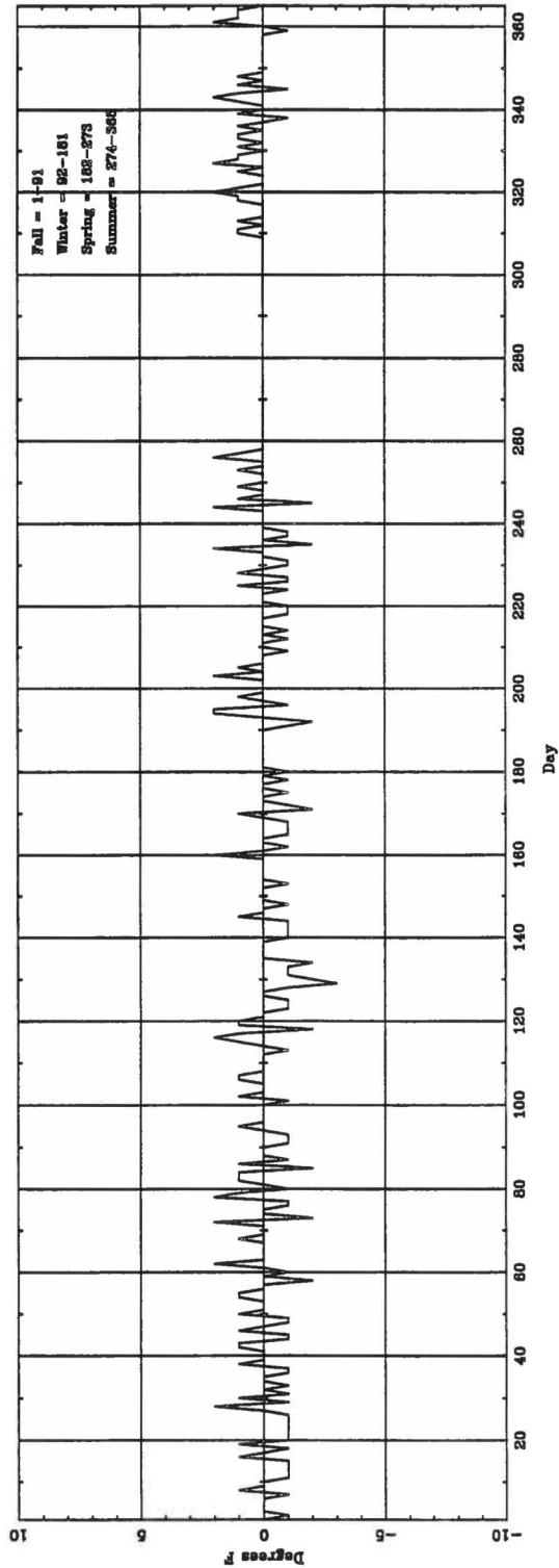
Daily \Delta T_{(low\text{-}hourly)} (ASOS - CONV) for PIA
