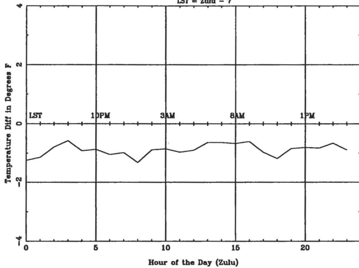
Average Diurnal Cycle for GJT - spring LST = Zulu - 7
