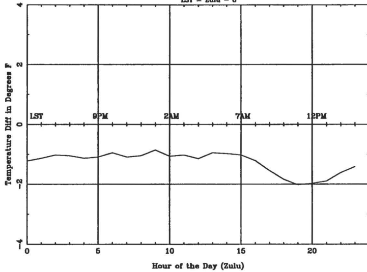
Average Diurnal Cycle for EUG - spring
