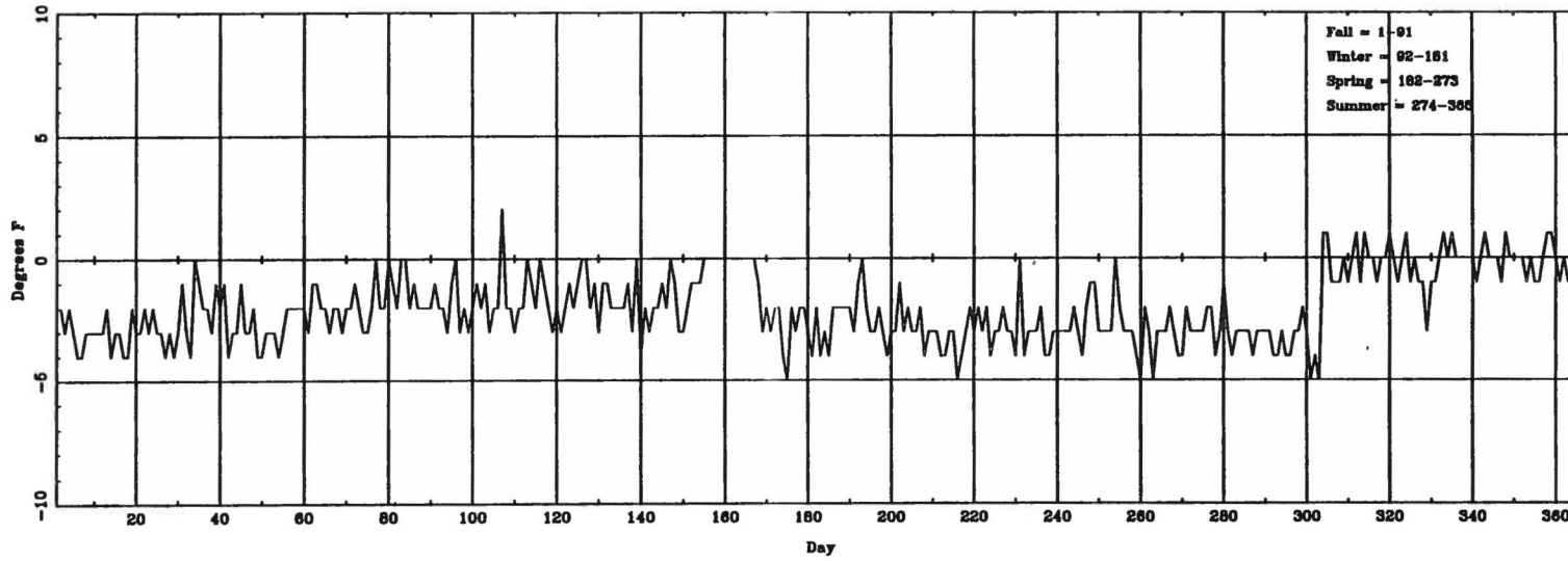
Daily \Delta T_{(lowest\ hourly)} (ASOS - CONV) for TUS
