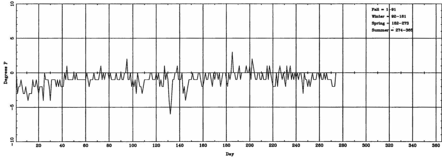
Daily \Delta T_{(lowest\ hourly)} (ASOS - CONV) for BFF
