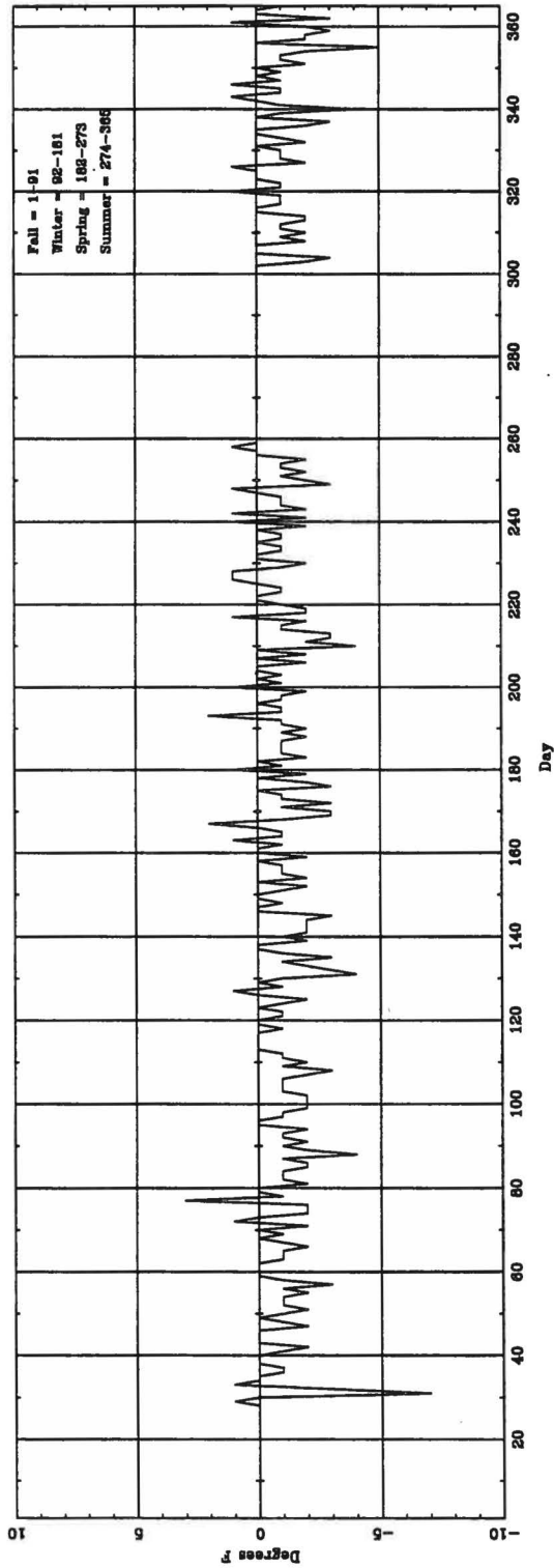
Daily \Delta T_{(highest\ beauty)} (ASOS - CONY) for GJT
