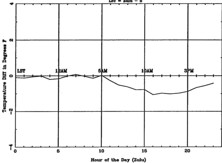
Average Diurnal Cycle for DAY - spring LST = Zulu - 5
