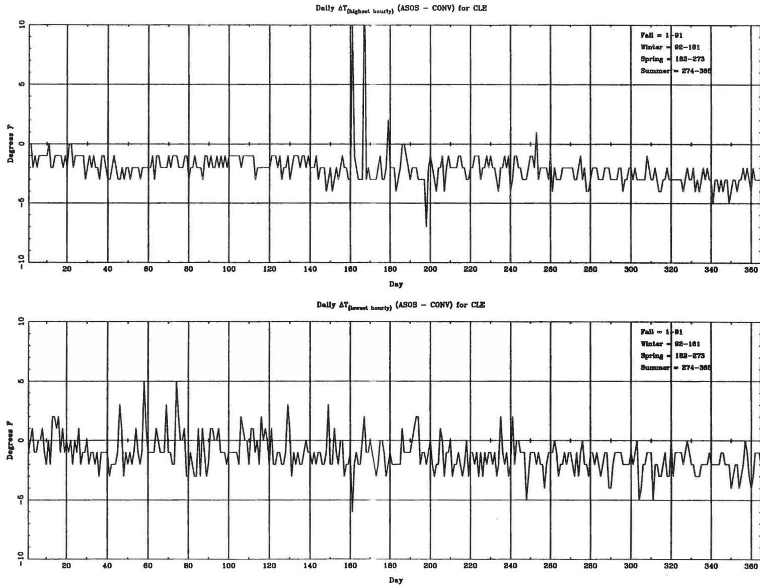
Fig. 3.2 (B) Temperature time series plots for Cleveland, OH.
