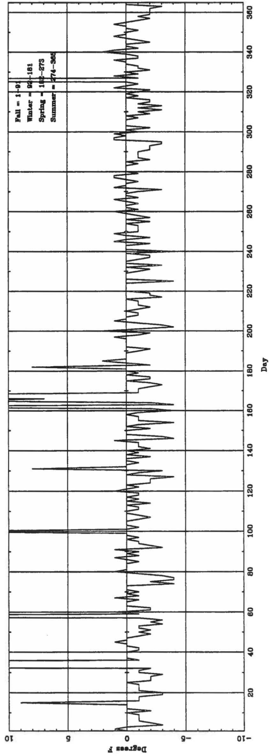
Daily AT (rawest hourly) (ASOS - CONY) for SLN
