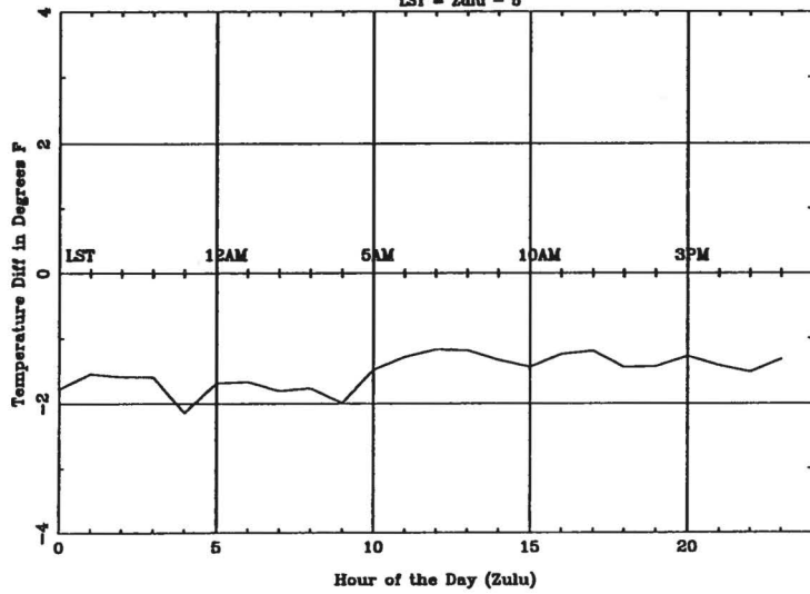
Average Diurnal Cycle for ABE - spring LST = Zulu - 5
