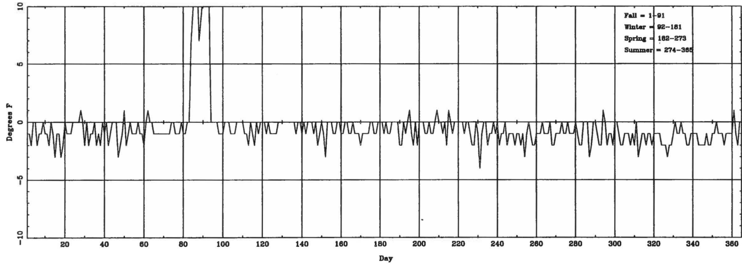
Daily \Delta T_{\text{(lowest hourly)}} (ASOS - CONV) for ERI
