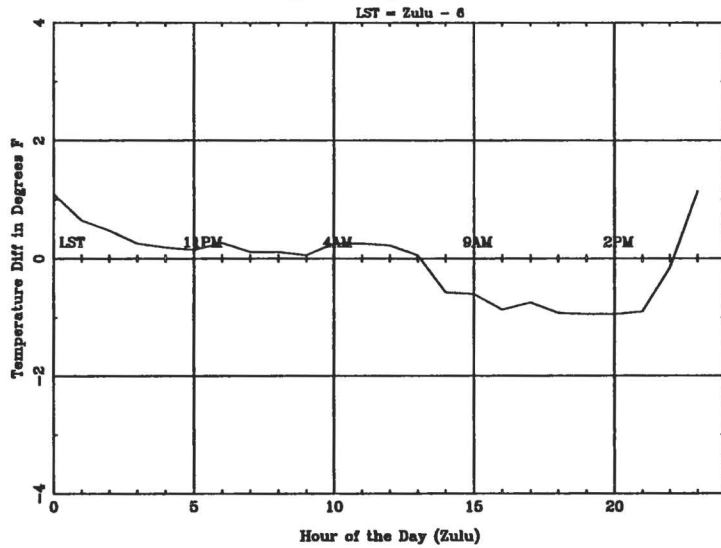
Average Diurnal Cycle for MLI - spring
