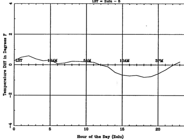
Average Diurnal Cycle for CAE - summer
