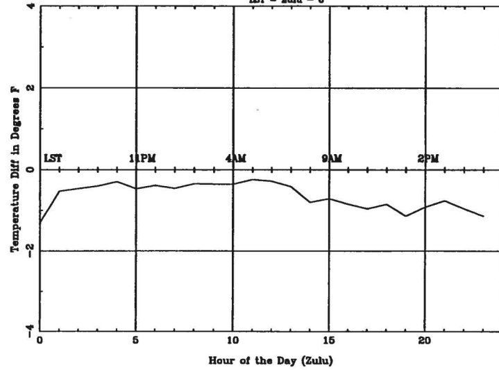
Average Diurnal Cycle for ALO - summer
