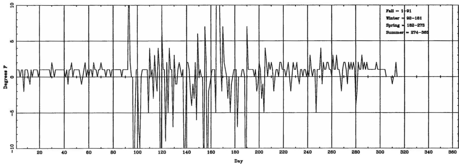
Daily \Delta T (lowest hourly) (ASOS - CONV) for ORH
