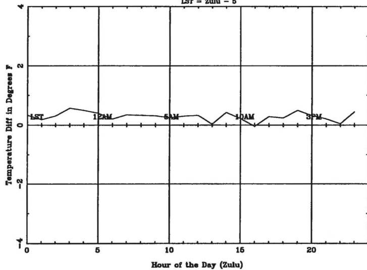
Average Diurnal Cycle for MCO - spring LST = Zulu - 5
