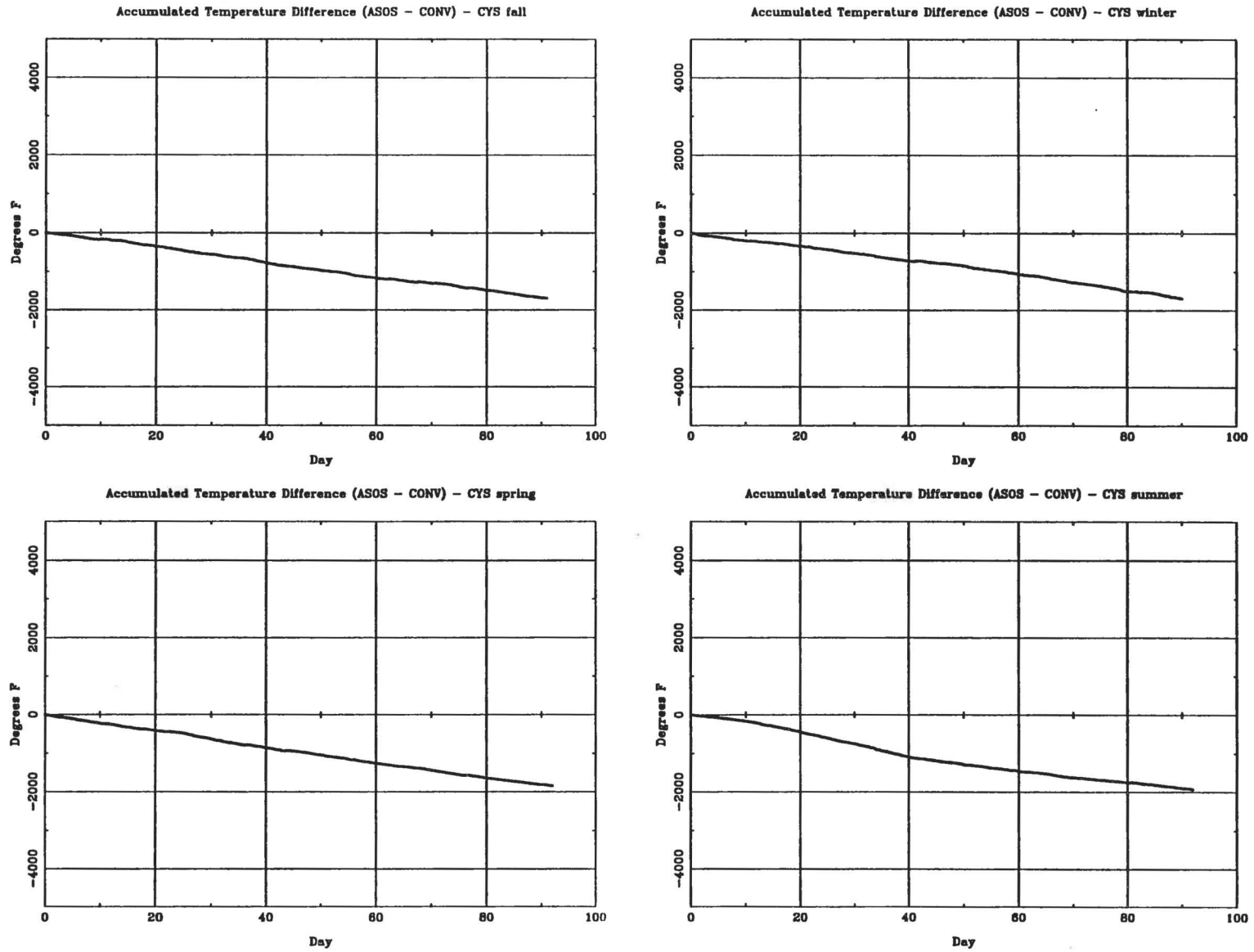
Fig. 3.1 (A) Seasonal accumulated temperature difference plots for Cheyenne, WY.
