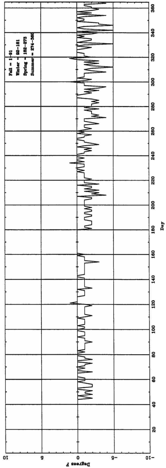
Daily \Delta T_{(morn\ hour)} (ASOS - CONV) for EUG
