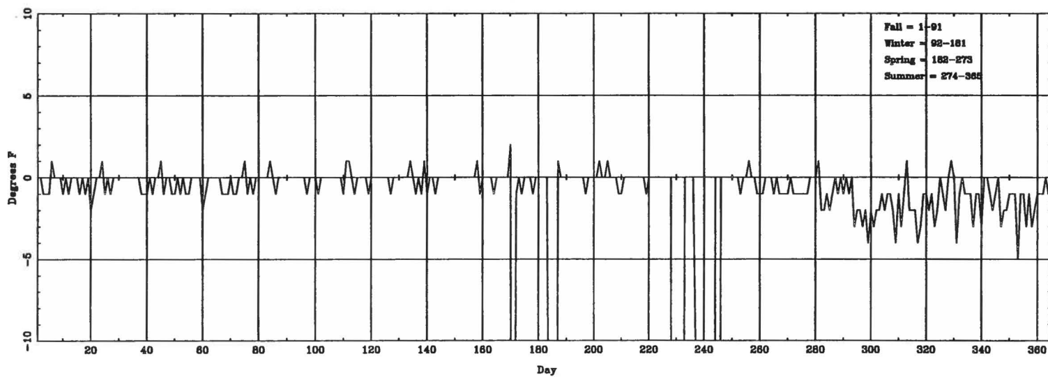
Daily \Delta T_{\text{(lowest hourly)}} (ASOS - CONV) for MHS
