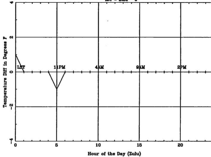
Average Diurnal Cycle for SUX - summer
