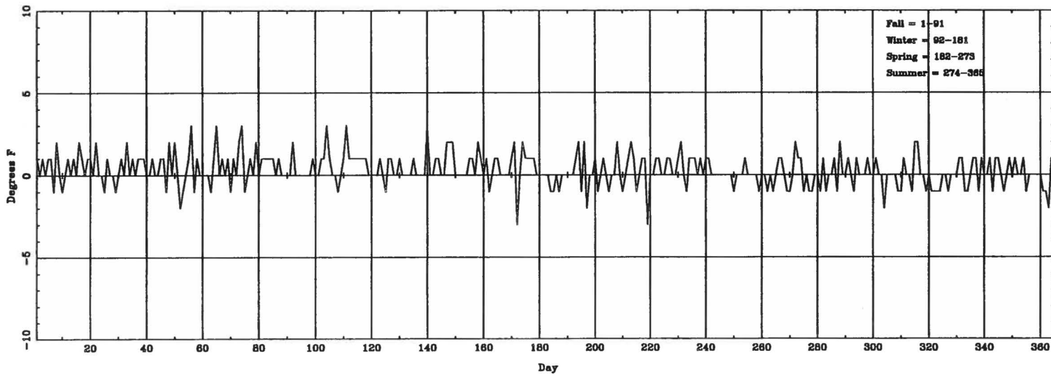
Daily \Delta T_{\text{(lowest hourly)}} (ASOS - CONV) for JKL
