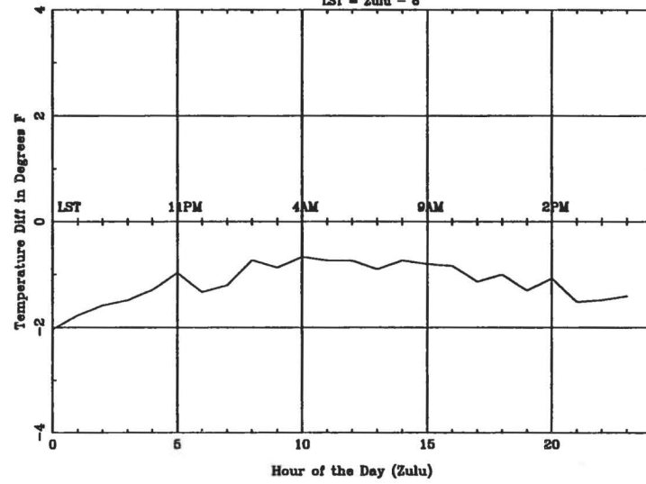
Average Diurnal Cycle for MCI - summer
