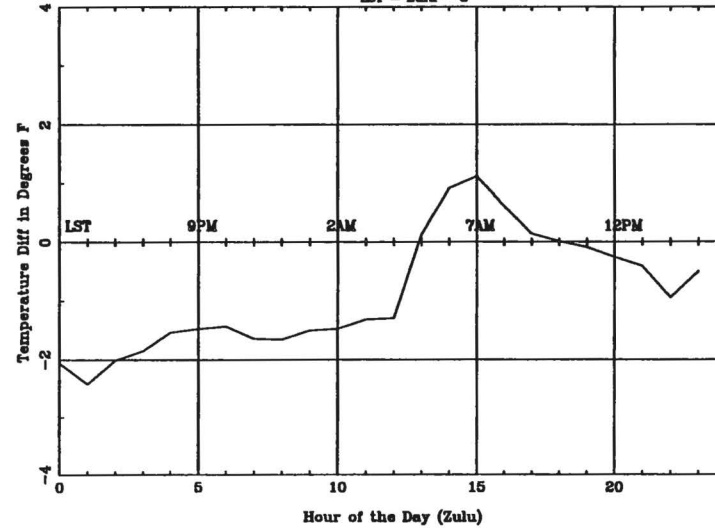
Average Diurnal Cycle for MHS - summer
