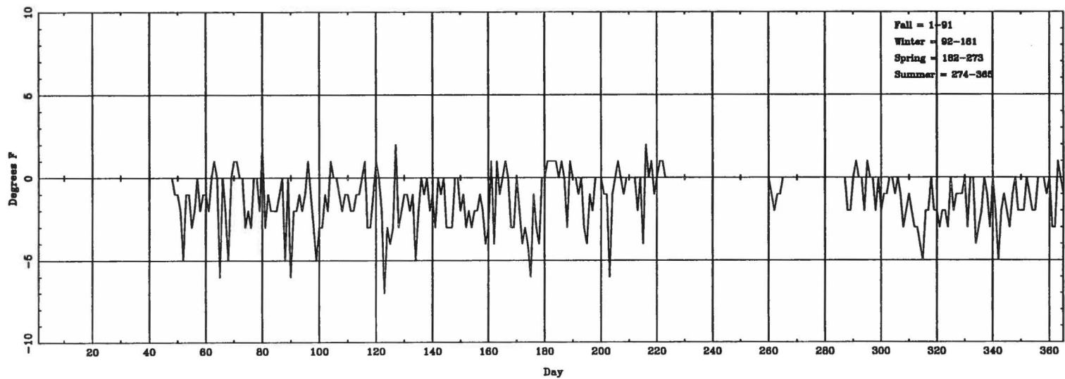
Daily \Delta T_{\text{(lowest hourly)}} (ASOS - CONV) for LBF
