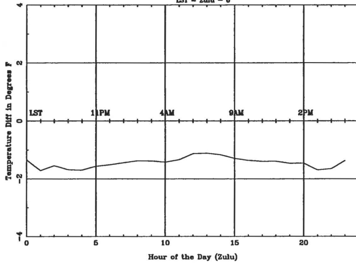
Average Diurnal Cycle for LCH - spring
