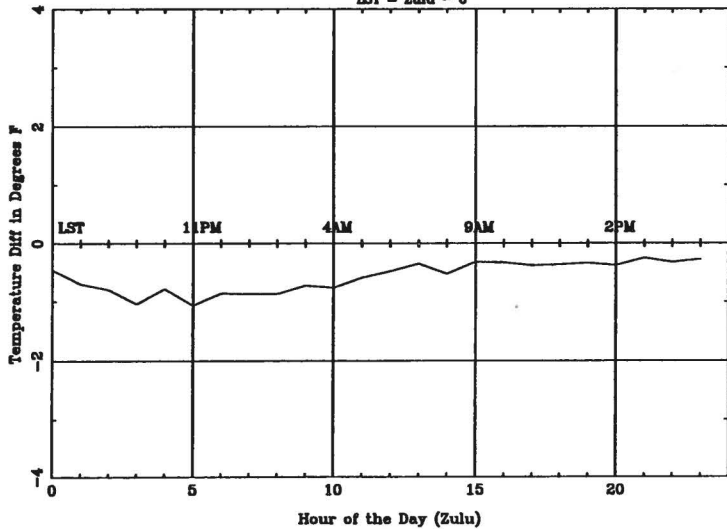
Average Diurnal Cycle for SUX - spring
