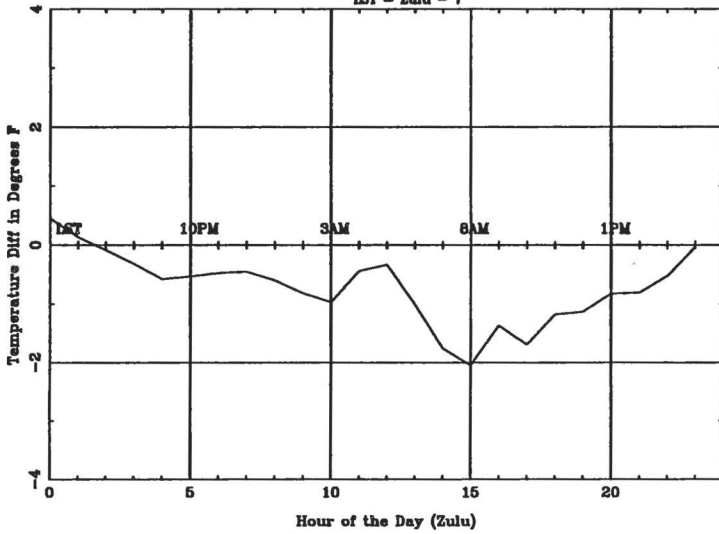
Average Diurnal Cycle for RAP - spring LST = Zulu - 7
