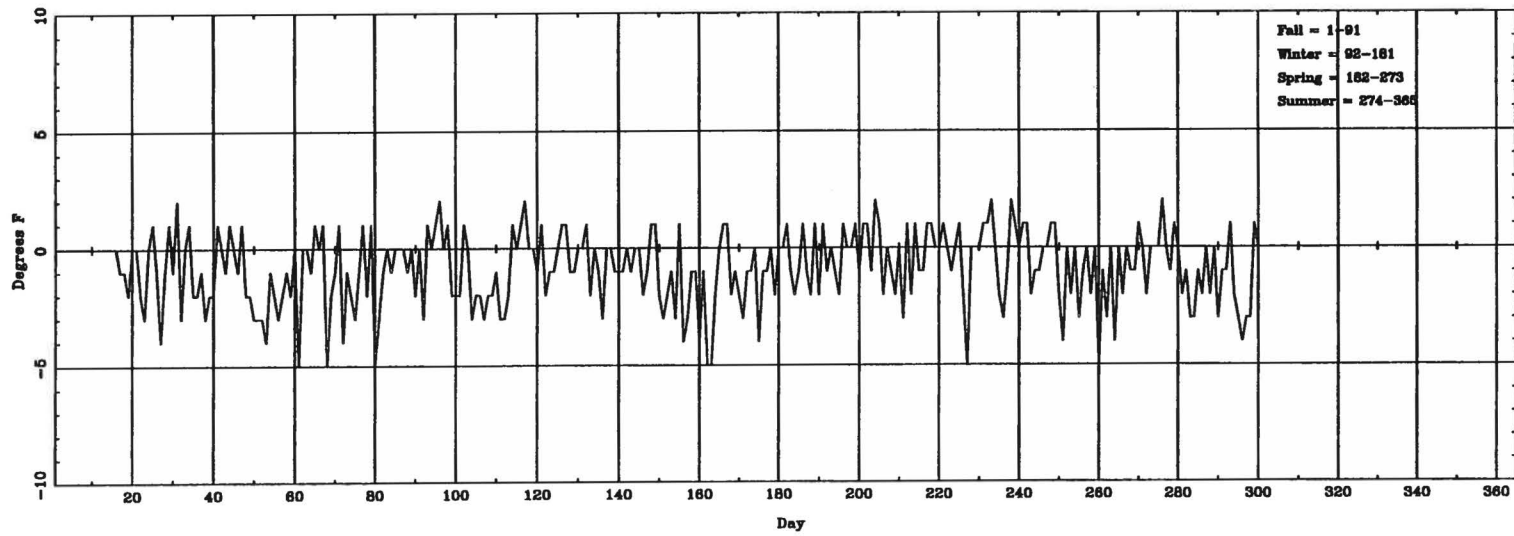
Daily \Delta T_{(lowest\ hourly)} (ASOS - CONV) for INW
