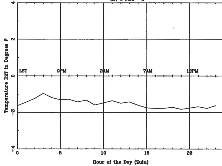
Average Diurnal Cycle for DRA - summer LST = Zulu - 8
