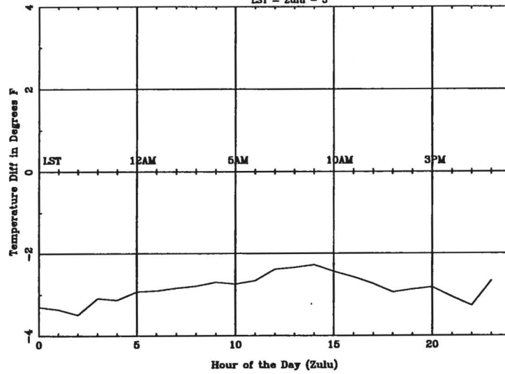
Average Diurnal Cycle for ATL - spring
