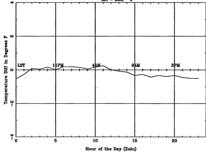
Average Diurnal Cycle for HON - summer LST = Zulu - 6
