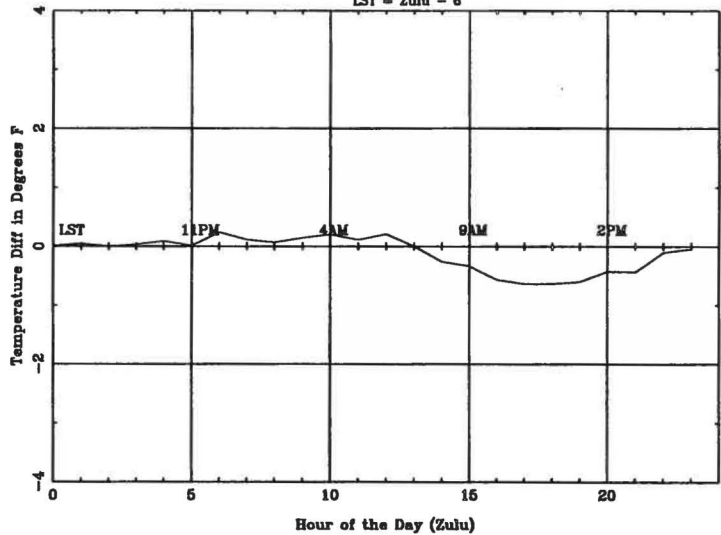
Average Diurnal Cycle for RFD - summer LST = Zulu - 6
