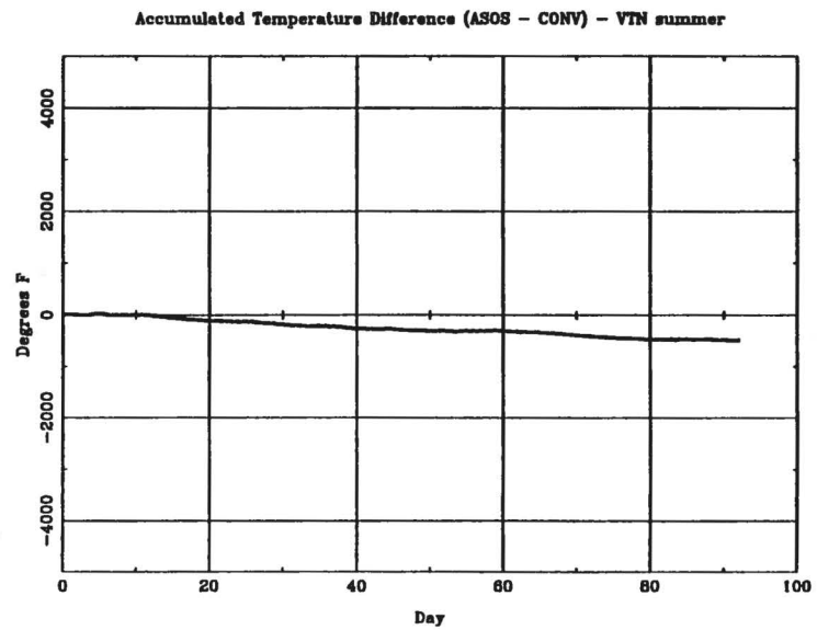
Fig. 3.1 (F) Seasonal accumulated temperature difference plots for Valentine, NE.
