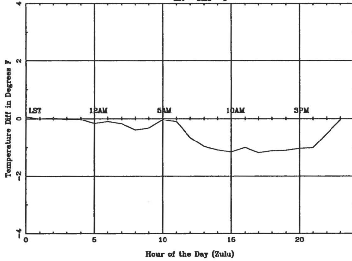
Average Diurnal Cycle for TLH - spring LST = Zulu - 5
