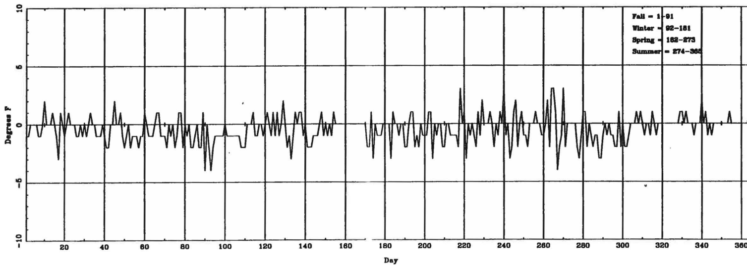
Fig. 3.2 (C) Temperature time series plots for Tucson, AZ.
