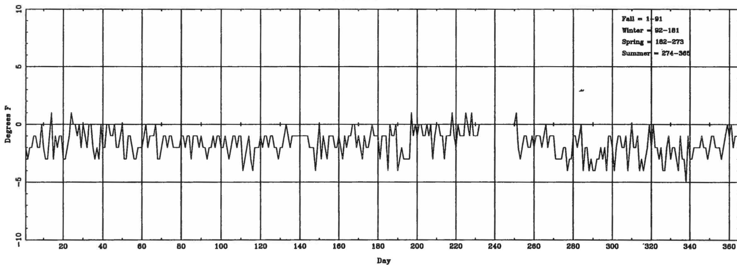
Daily \Delta T_{\text{(lowest hourly)}} (ASOS - CONV) for GRB
