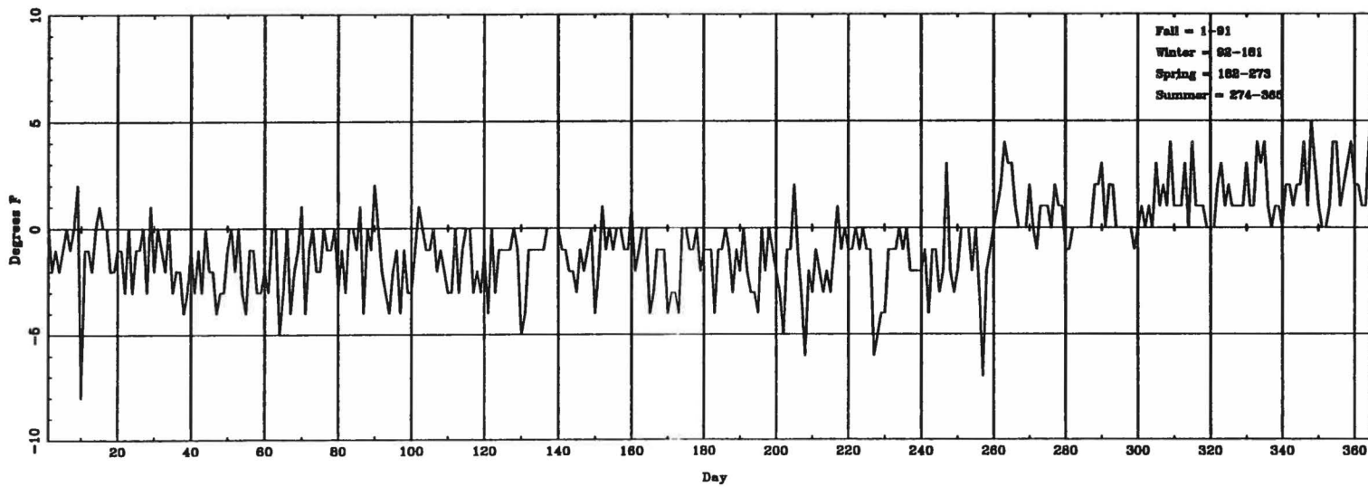
Fig. 3.2 (A) Temperature time series plots for Atlantic City, NJ.
