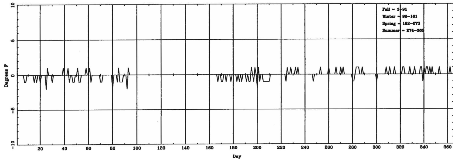
Daily \Delta T_{\text{(lowest hourly)}} (ASOS - CONV) for HON
