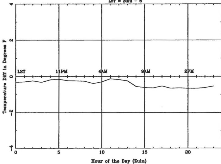
Average Diurnal Cycle for COU - spring
