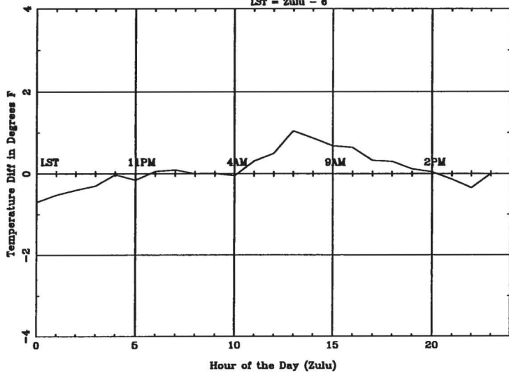
Average Diurnal Cycle for VTN - spring
