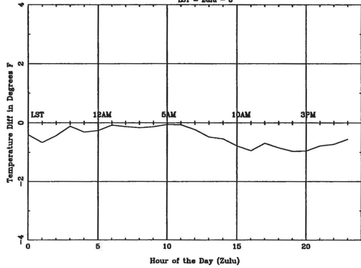
Average Diurnal Cycle for SBN - summer LST = Zulu - 5
