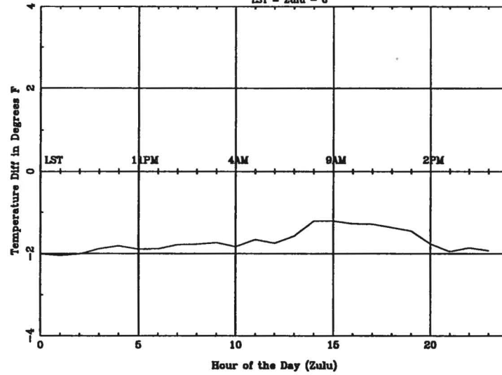
Average Diurnal Cycle for GRB - summer LST = Zulu - 6
