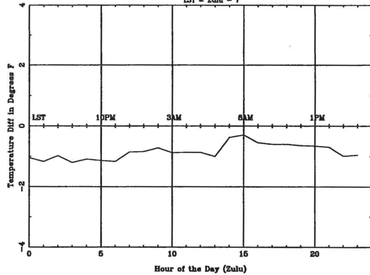
Average Diurnal Cycle for RAP - summer LST = Zulu - 7
