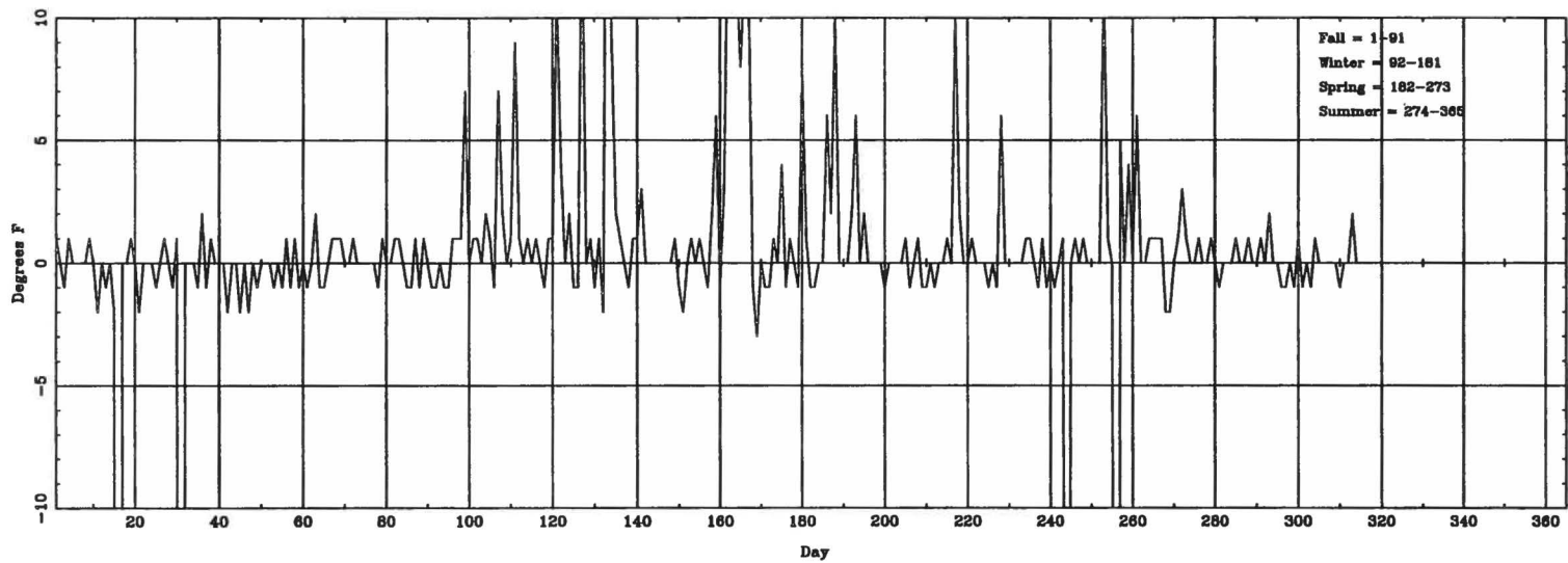
Daily \Delta T (lowest hourly) (ASOS - CONV) for ORH
