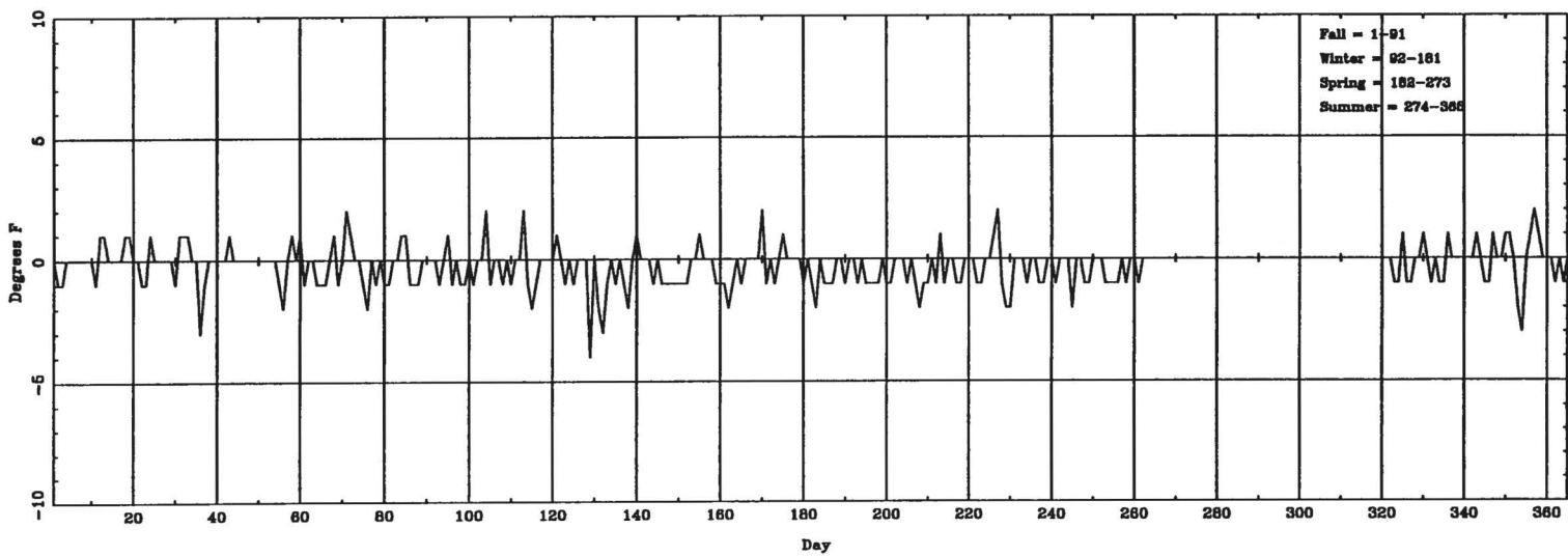
Daily \Delta T_{\text{(lowest hourly)}} (ASOS - CONV) for APN
