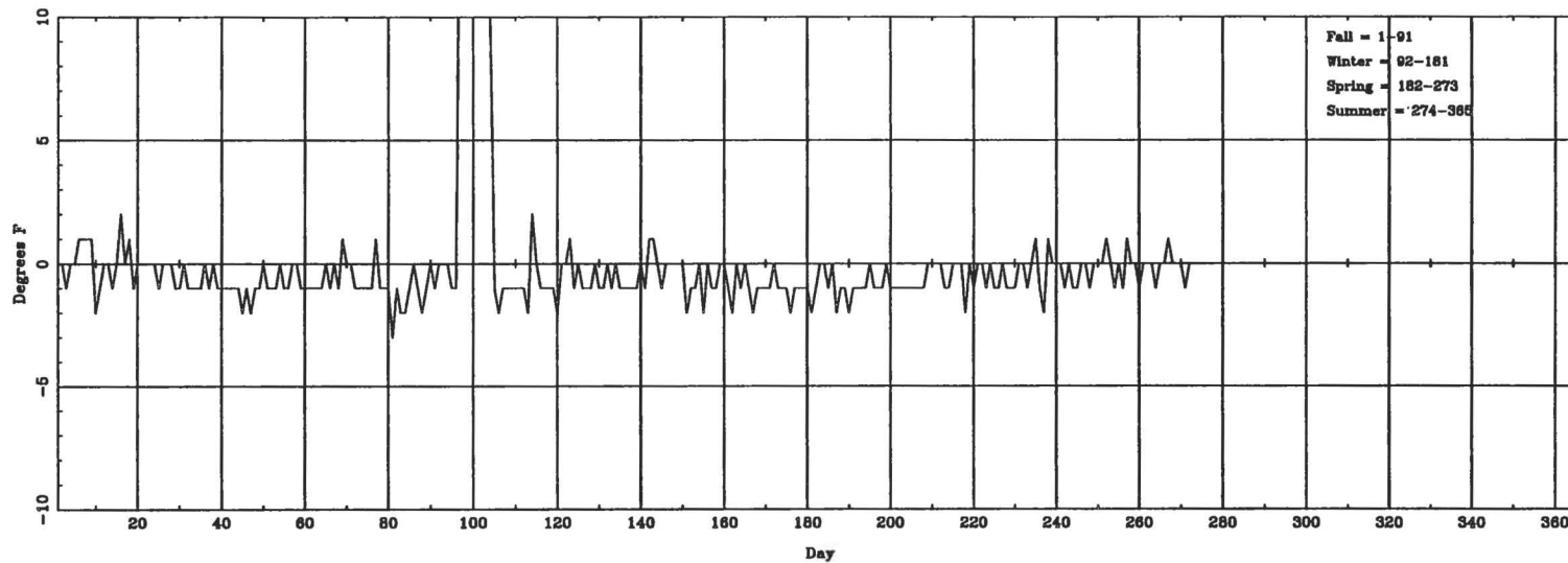
Daily \Delta T_{\text{(lowest hourly)}} (ASOS - CONV) for PDT
