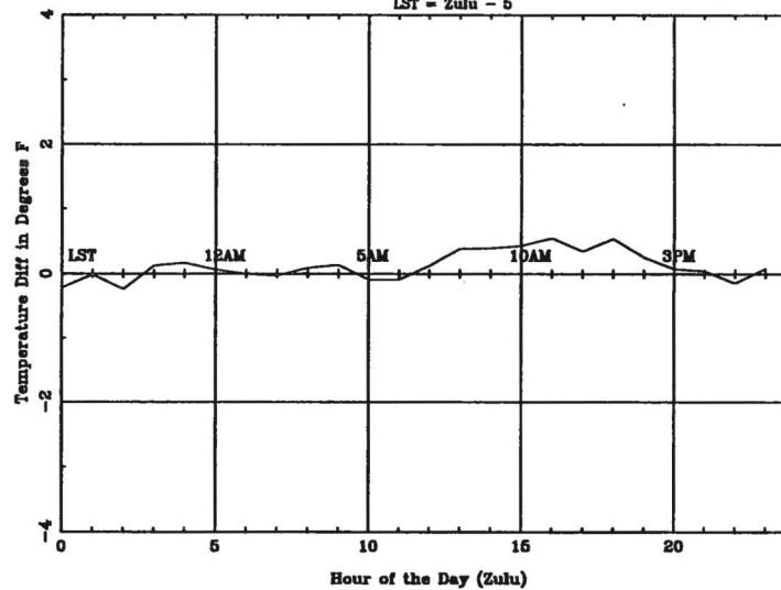
Average Diurnal Cycle for MCO - summer LST = Zulu - 5
