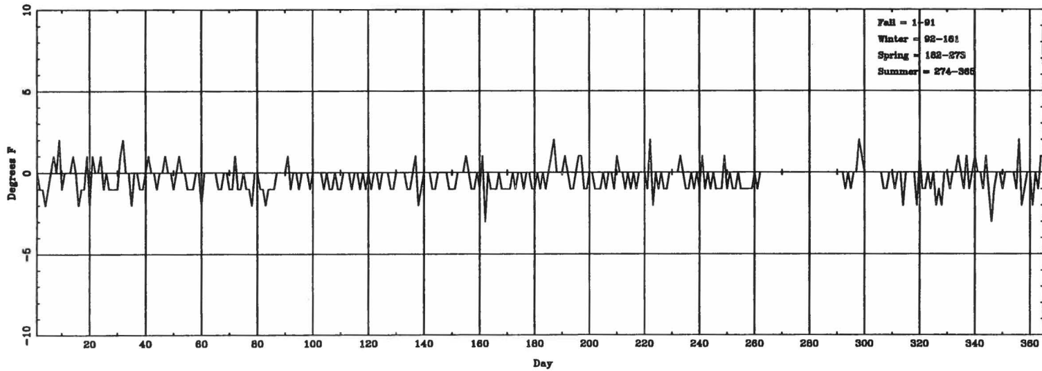
Daily \Delta T_{\text{(lowest hourly)}} (ASOS - CONV) for RDD
