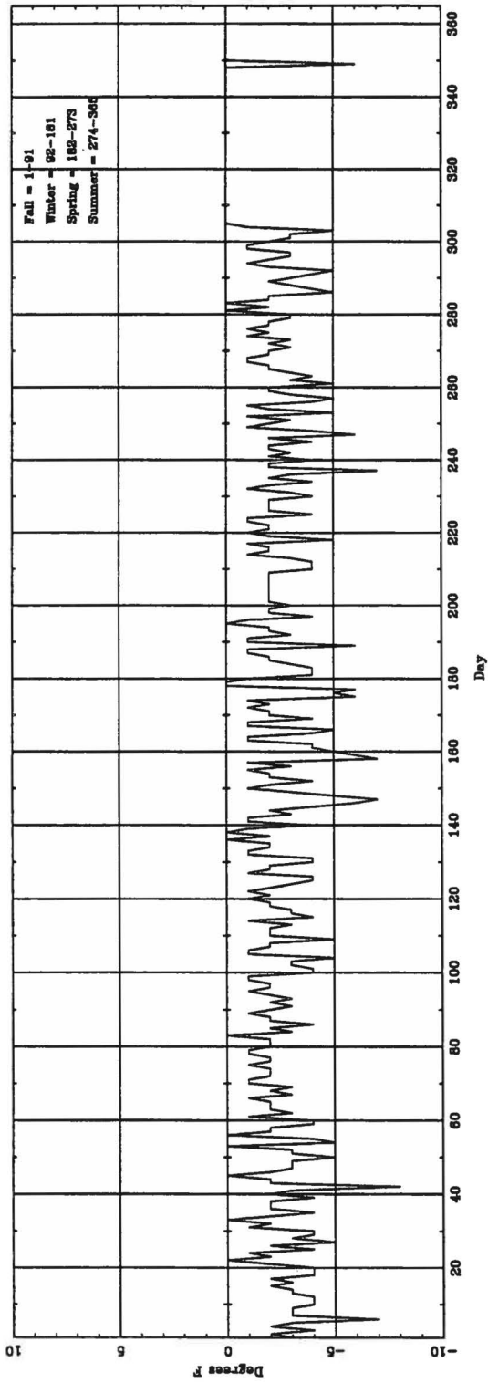
Daily AT (lightest hourly) (ASOS - CONV) for MIKE
