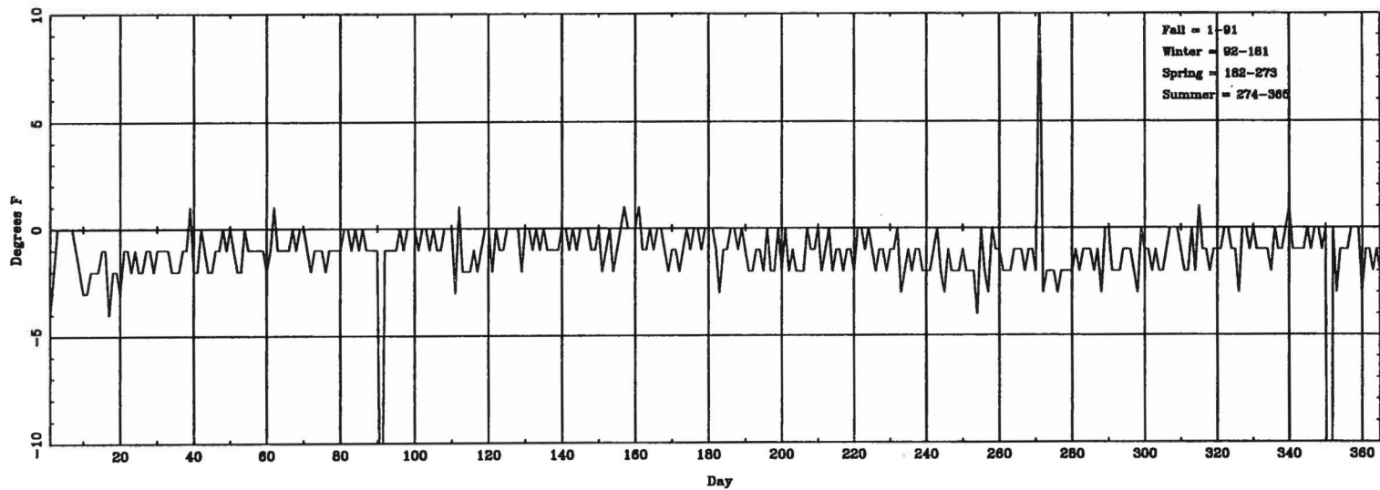
Daily \Delta T_{\text{(lowest hourly)}} (ASOS - CONV) for SBN
