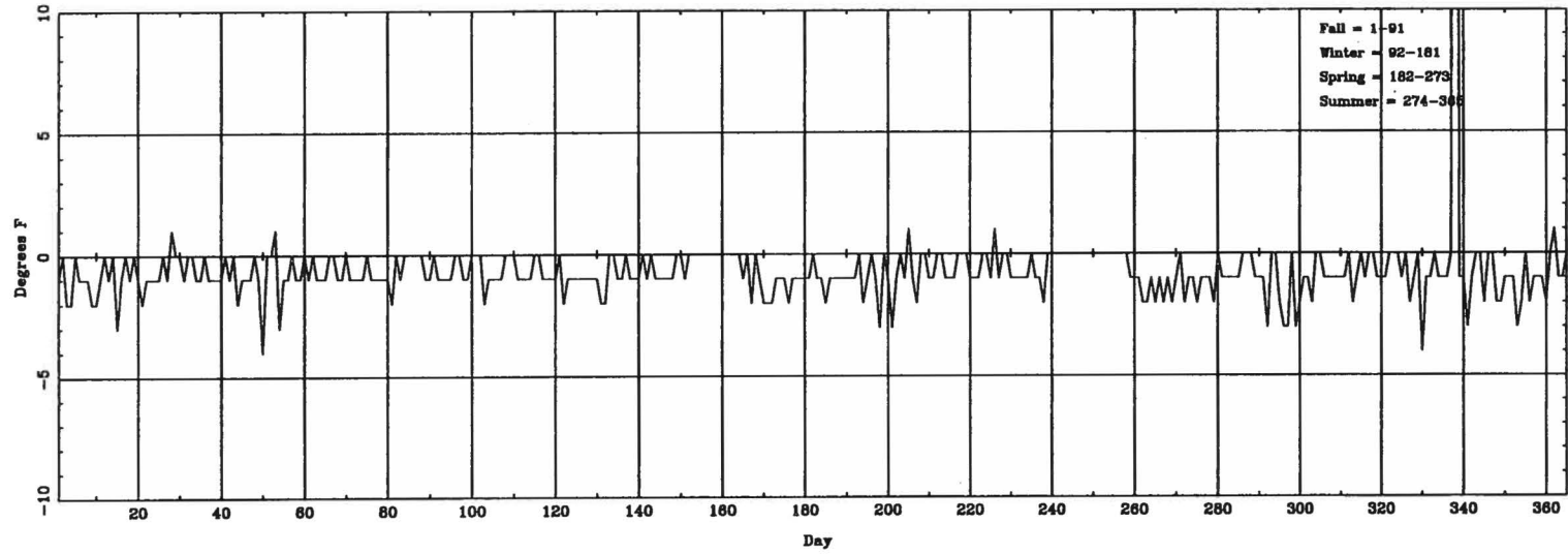
Daily \Delta T_{(lowest\ hourly)} (ASOS - CONV) for BGM
