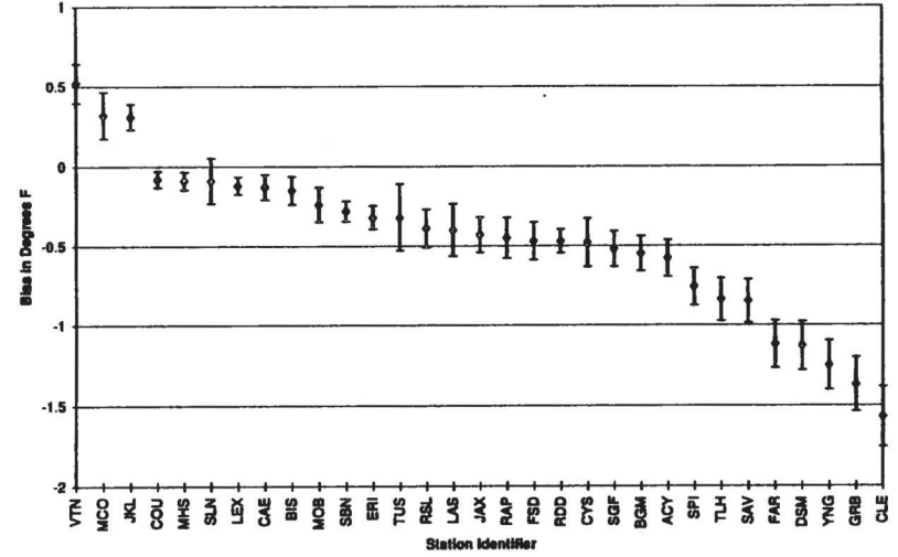
D. Instrument Bias for 4-season stations for Summer
