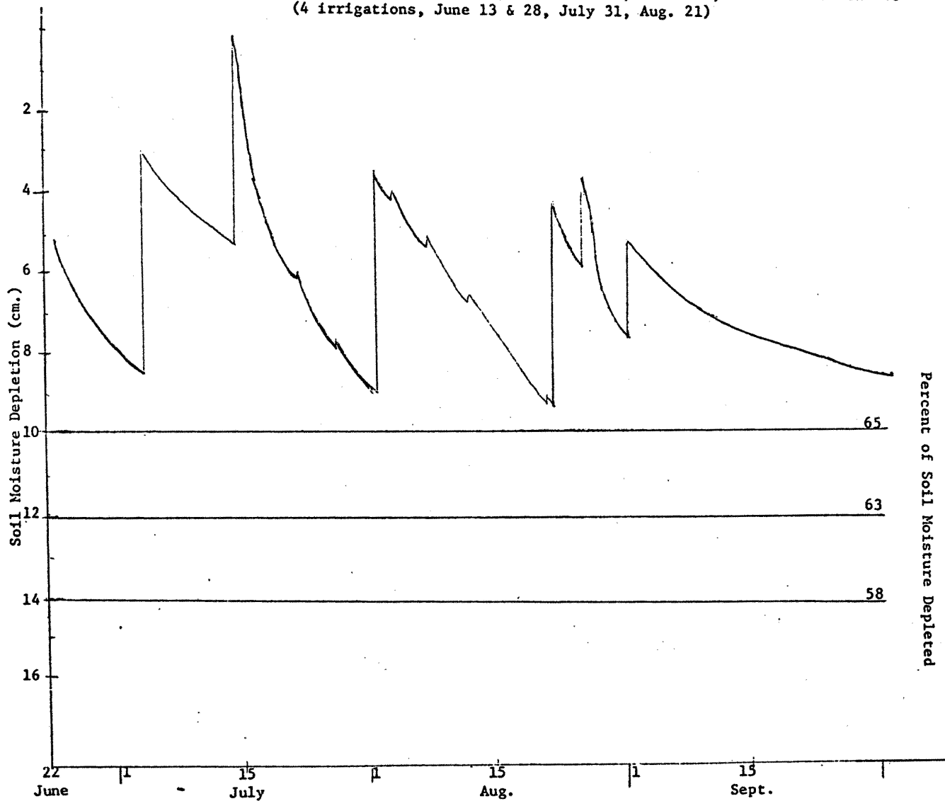
Figure A10--Level of soil moisture in corn experiment, Fort Collins, Colorado, 1972. Treatment 4C (4 irrigations, June 13 & 28, July 31, Aug. 21)
