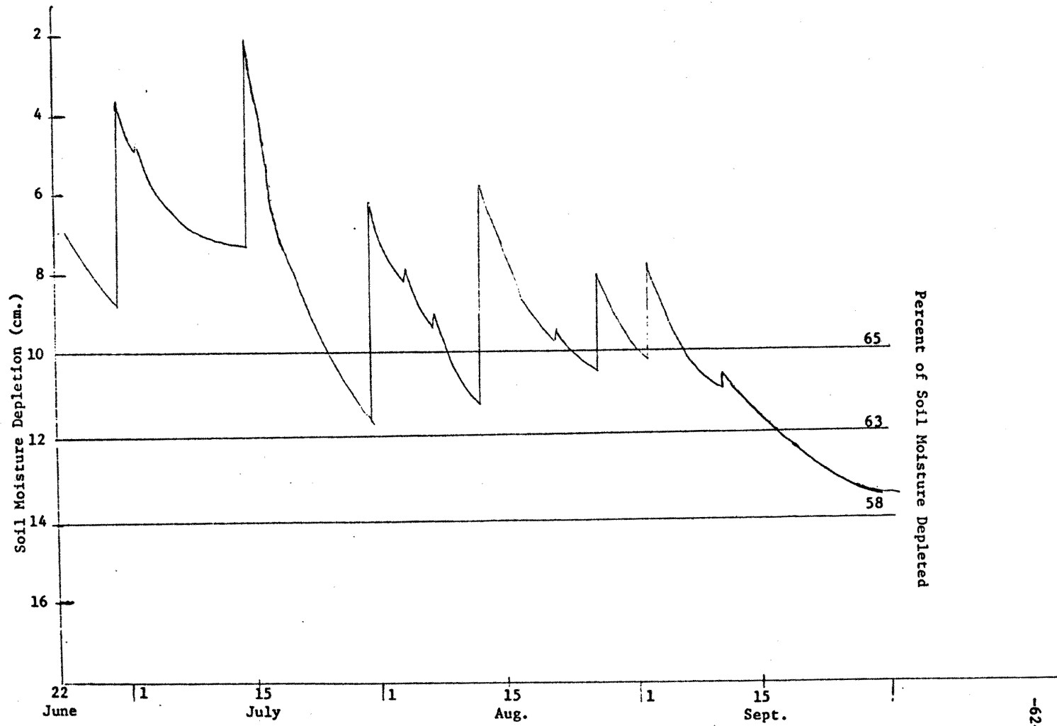
Figure A9—Level of soil moisture in corn experiment, Fort Collins, Colorado, 1972. Treatment 4B (4 irrigations, June 13 & 28, July 28, Aug. 11)
