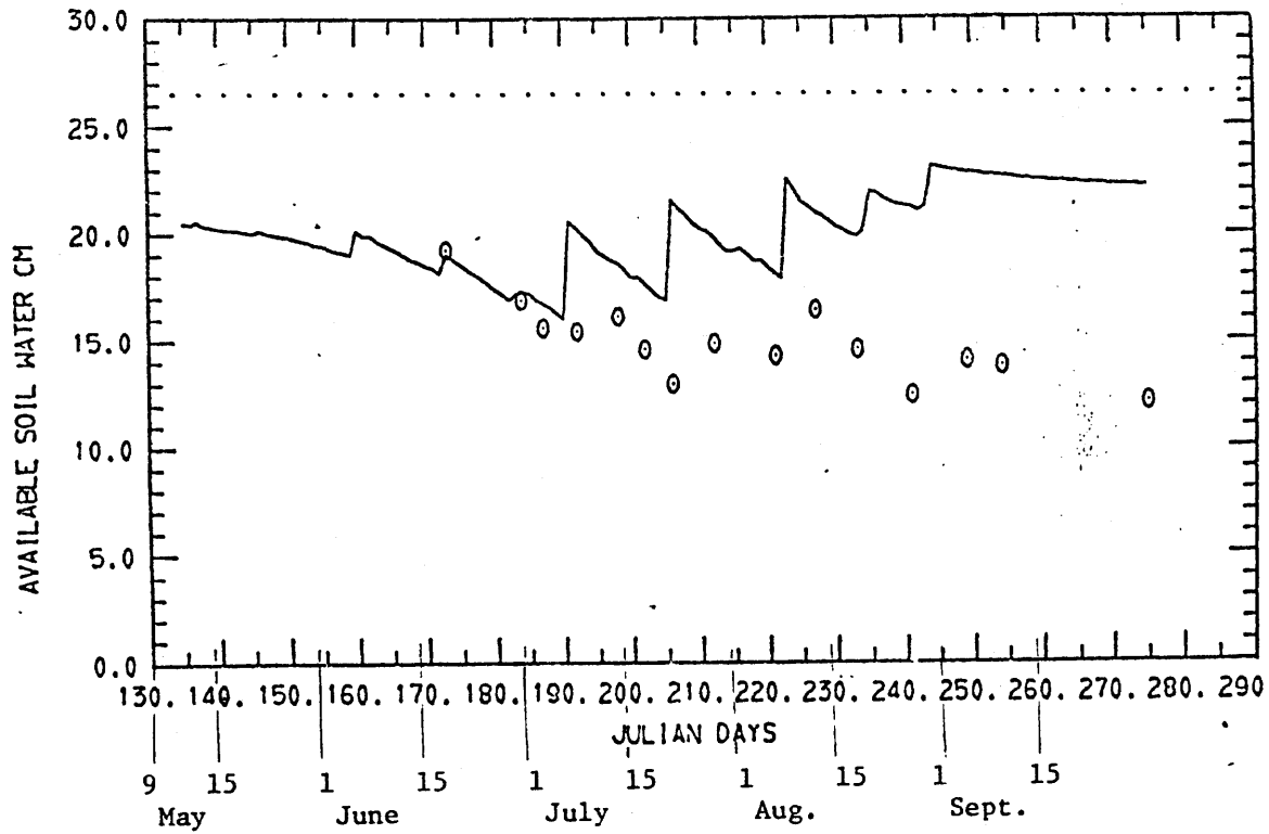
FIG. B5--TREATMENT 3B -- THREE 5 CM IRRIGATION
