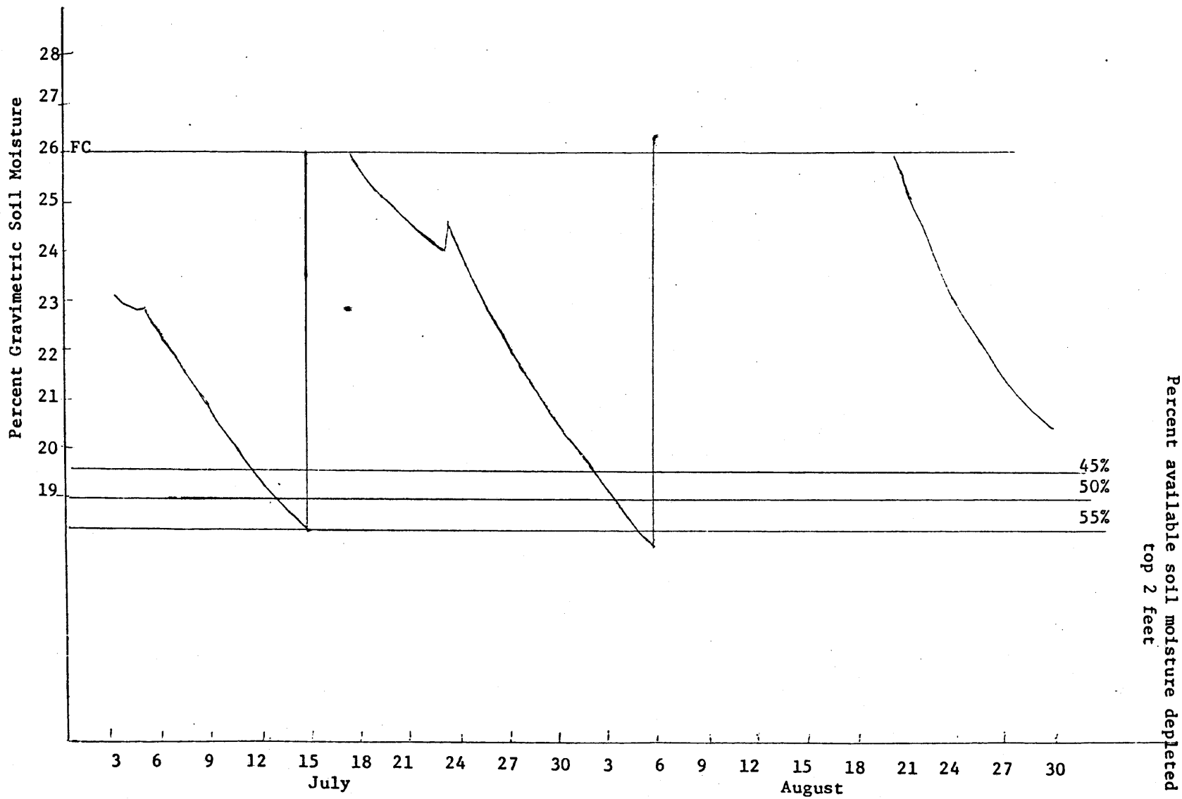
Figure A14--Level of soil moisture in corn experiment, Fort Collins, Colorado, 1968, Treatment III
