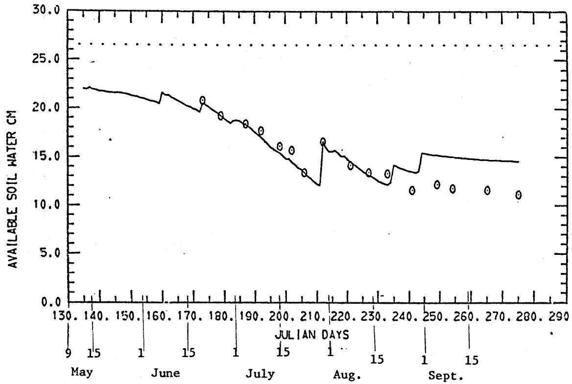
FIG. B2-TREATMENT 1B-- ONE 5 CM IRRIGATION
