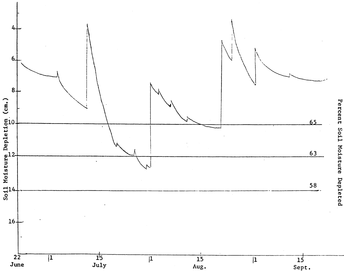
Figure A8—Level of soil moisture in corn experiment, Fort Collins, Colorado, 1972. Treatment 3C (3 irrigations, June 13, Aug. 2, Aug. 21)
