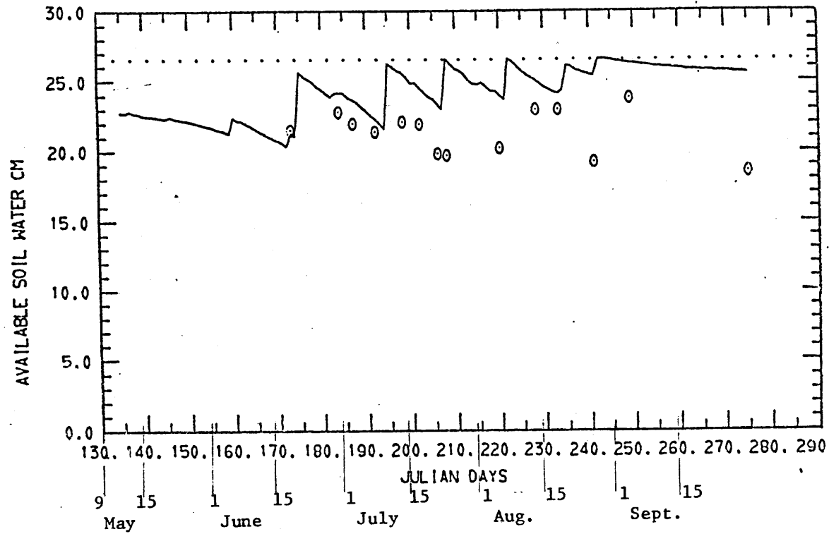
FIG. B10 TREATMENT 5 -- FIVE 5 CM IRRIGATION
