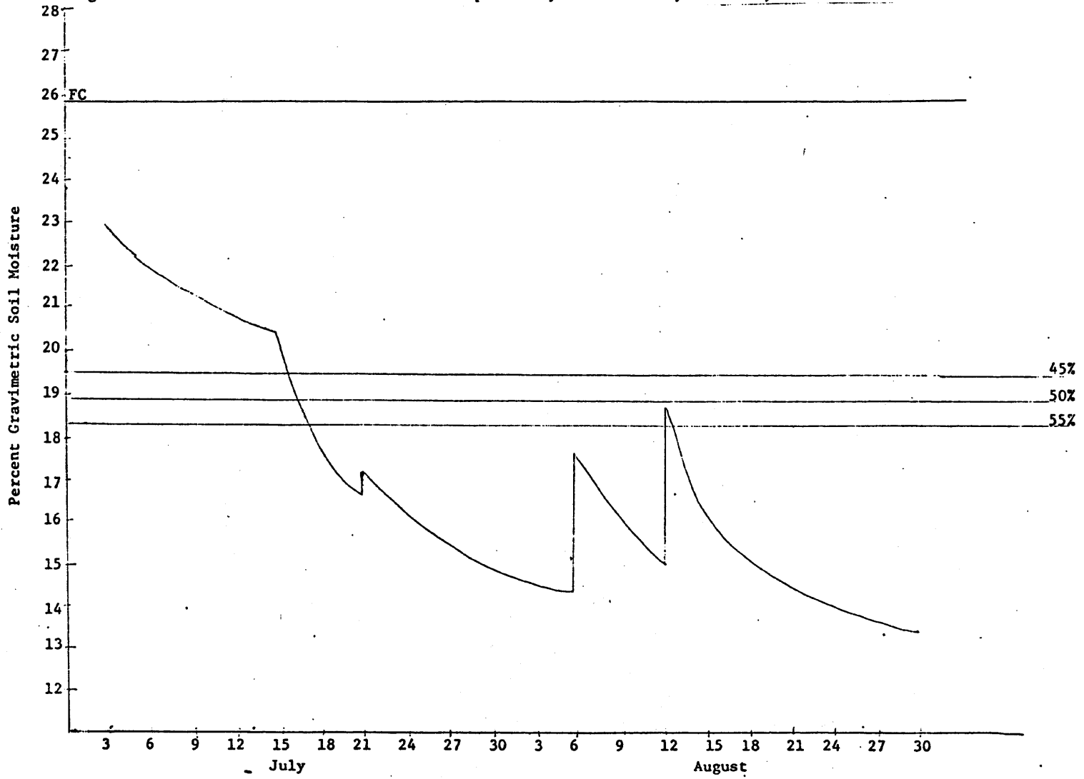
Figure A16--Level of soil moisture in corn experiment, Fort Collins, Colorado, Treatment V
