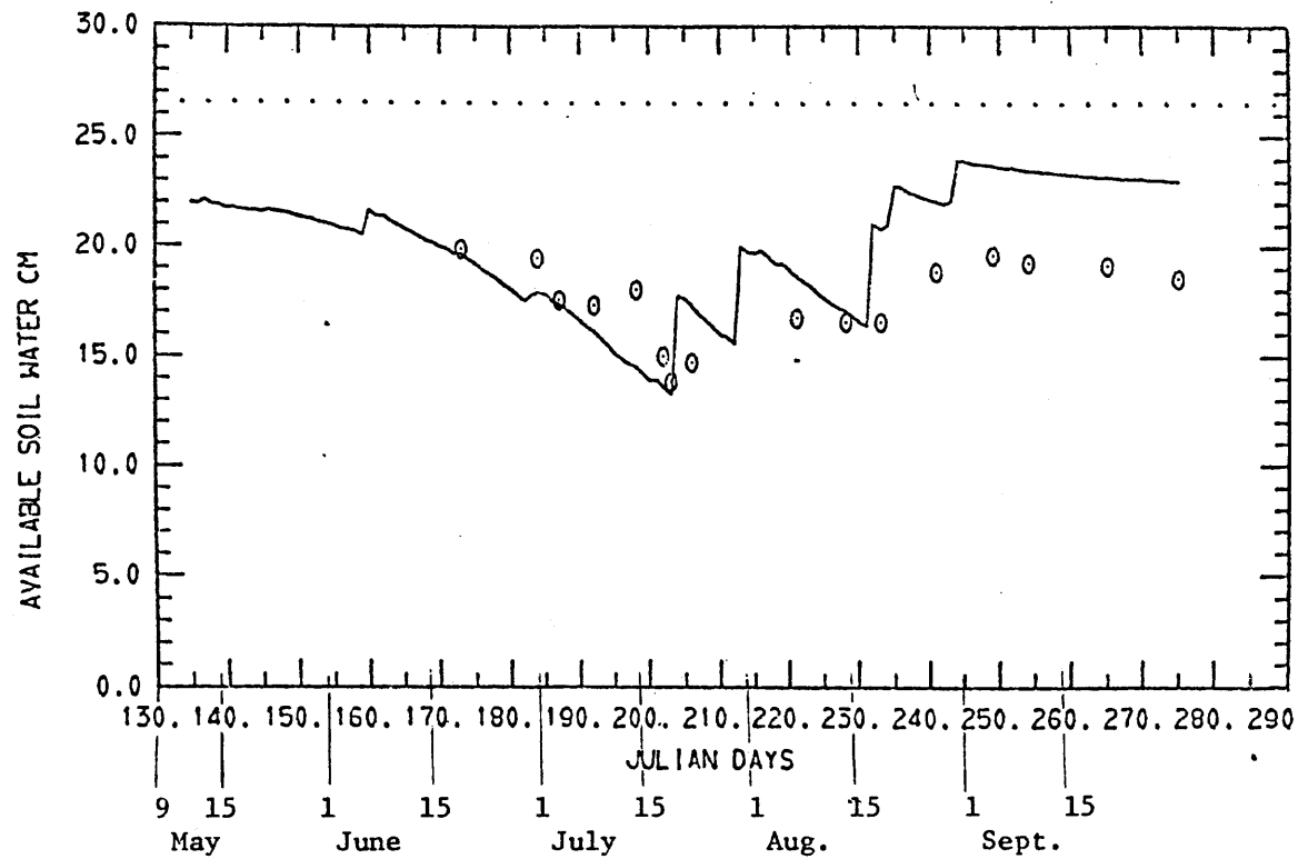
FIG. B6-TREATMENT 3C -- THREE 5 CM IRRIGATION
