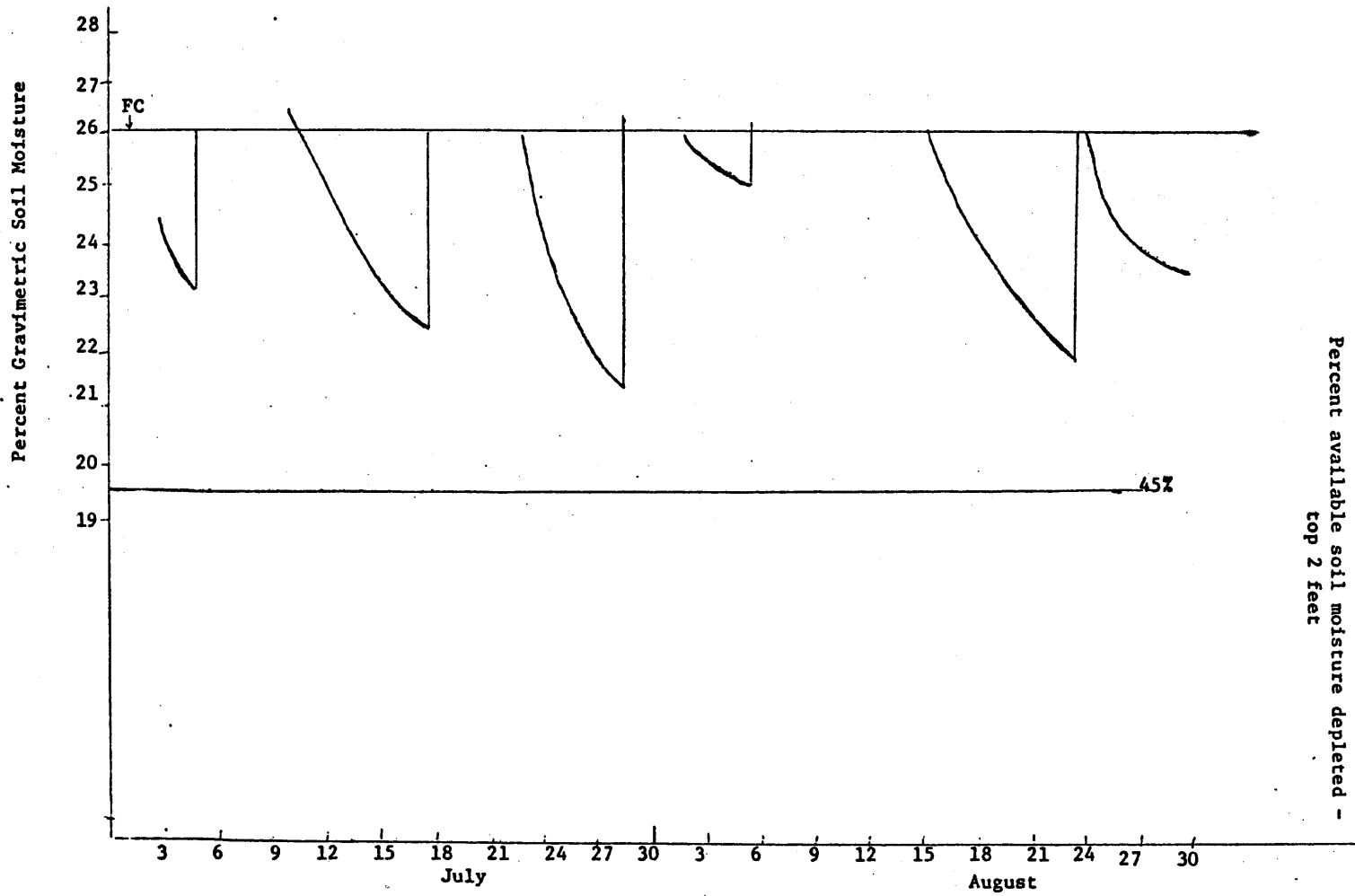
Figure A12--Level of soil moisture in corn experiment, Fort Collins, Colorado, 1968, Treatment I
