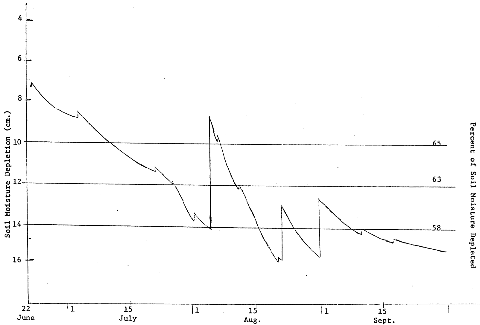
Figure A6.-Level of soil moisture in corn experiment, Fort Collins, Colorado, 1972. Treatment 1C (one irrigation, Aug. 4)
