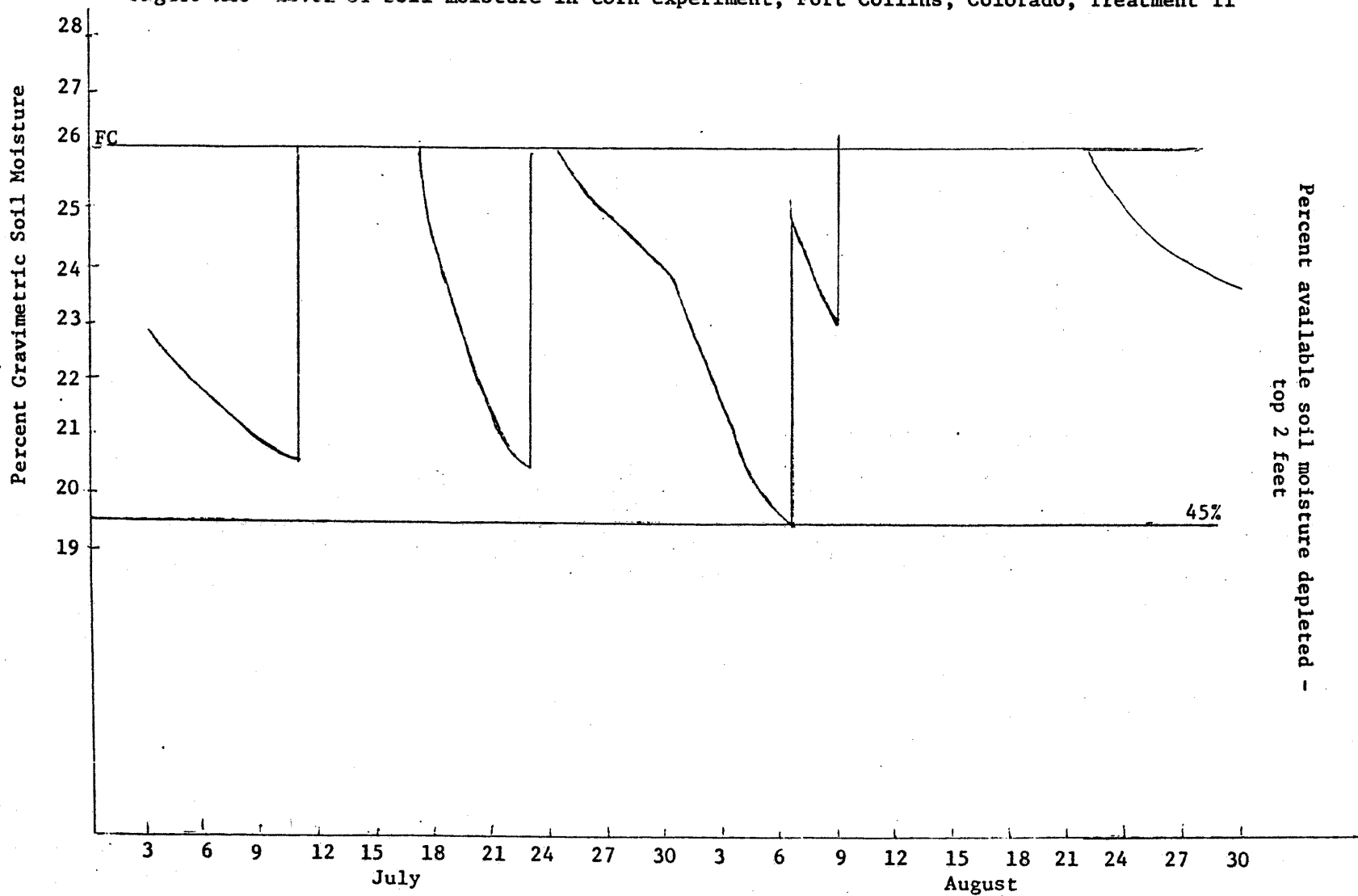
Figure A13--Level of soil moisture in corn experiment, Fort Collins, Colorado, Treatment II
