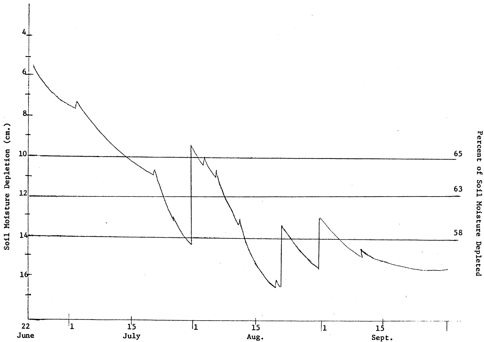
Figure A5-Level of soil moisture in corn experiment, Ft. Collins, Colorado, 1972. Treatment 1B (one irrigation July 31)
