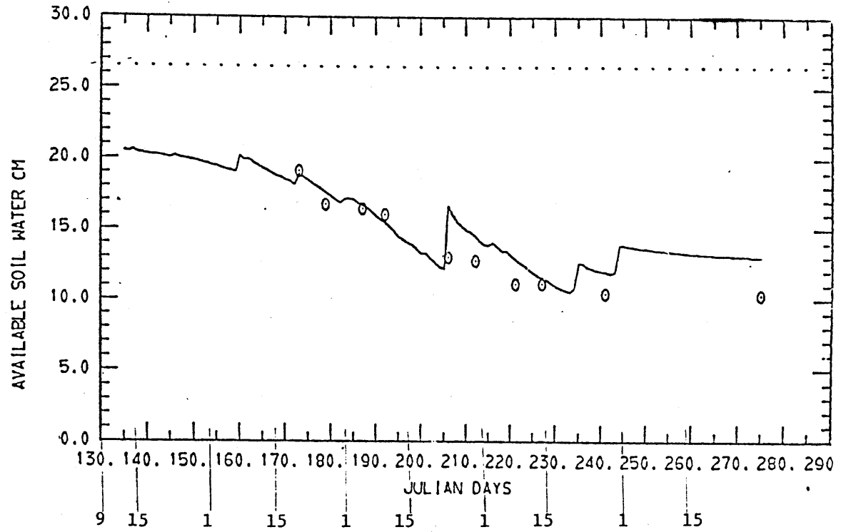
FIG. B1 - TREATMENT 1A-- ONE 5 CM IRRIGATION
