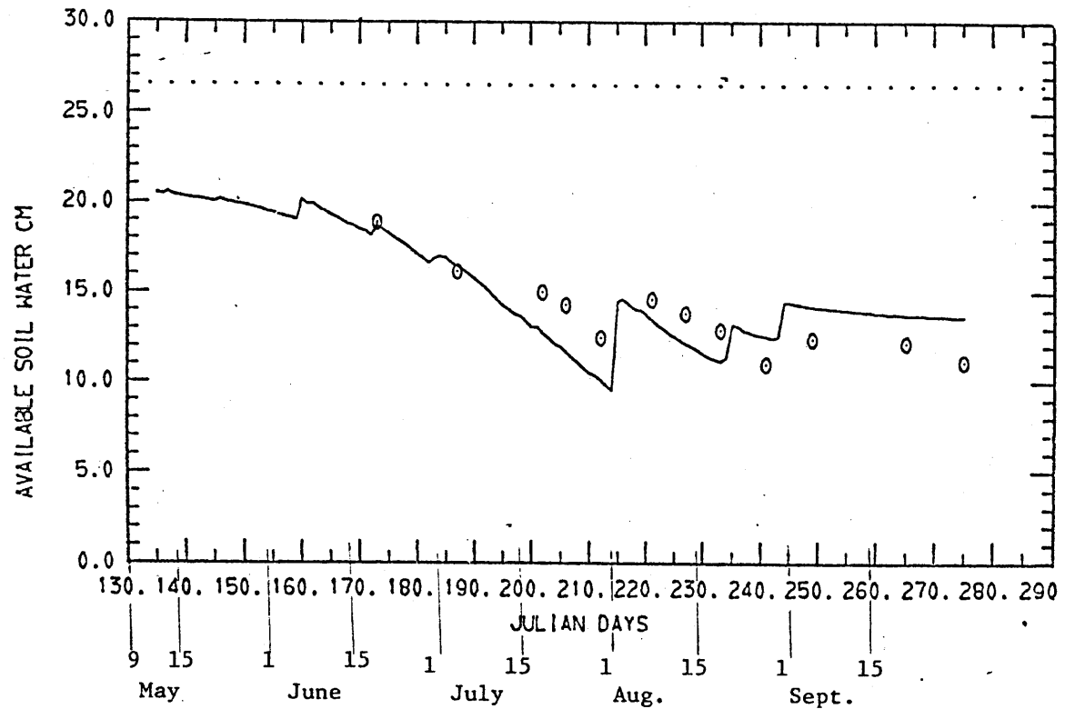
FIG. B3- TREATMENT 1C-- ONE 5 CM IRRIGATION
