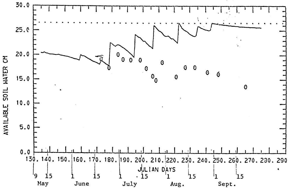
FIG. B8 -TREATMENT 4B -- FOUR 5 CM IRRIGATION
