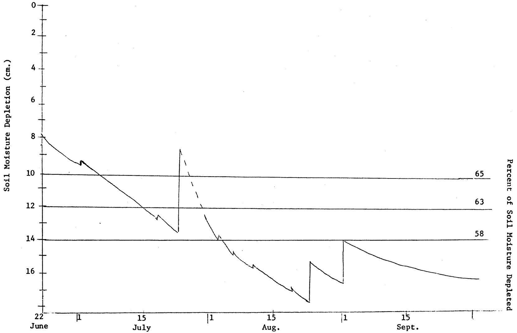
Figure A1-Level of soil moisture in corn irrigation experiment, Fort Collins, Colorado, 1972. Treatment/A (one irrigation, July 25)
