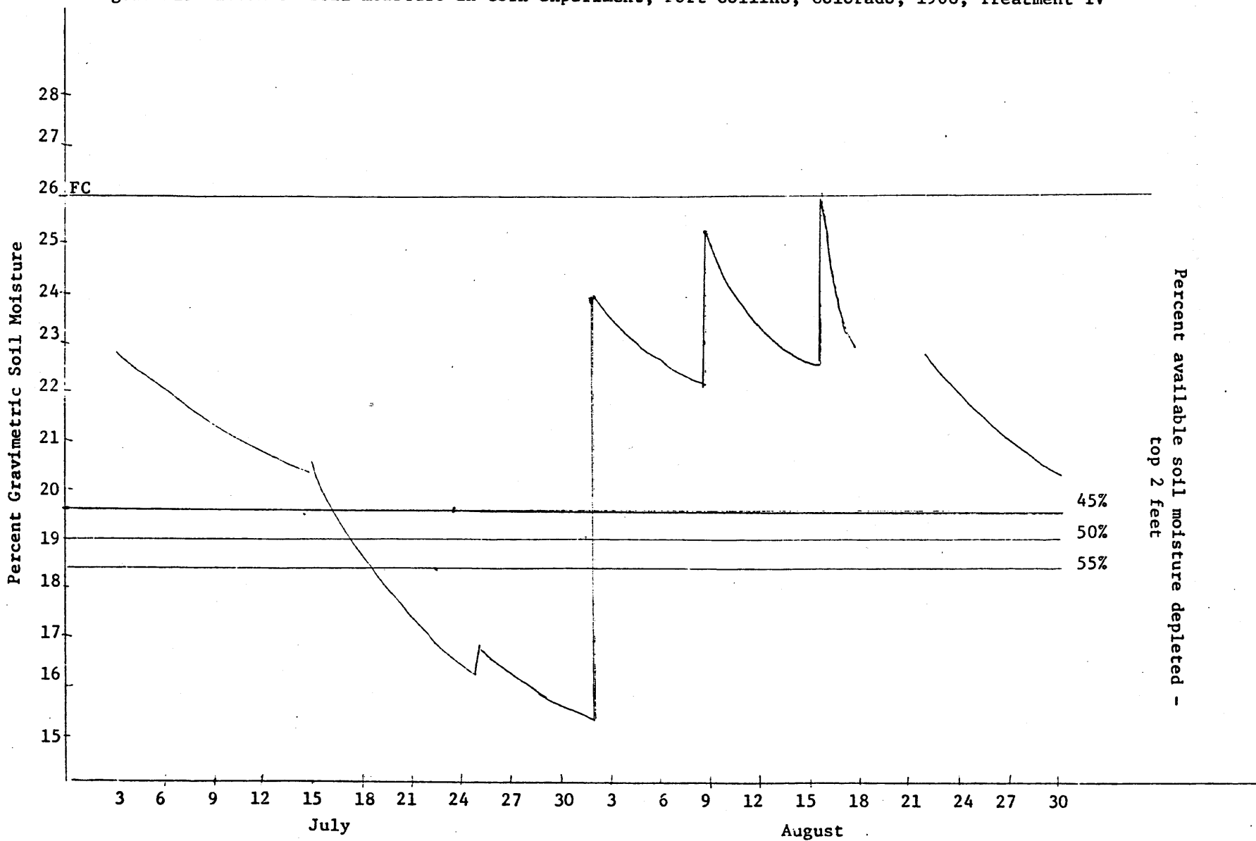
Figure A15--Level of soil moisture in corn experiment, Fort Collins, Colorado, 1968, Treatment IV
