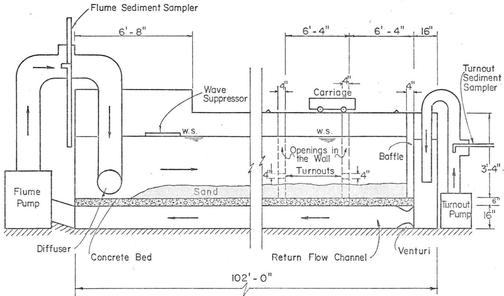
Figure 6. Schematic Arrangement of Laboratory Flume.
