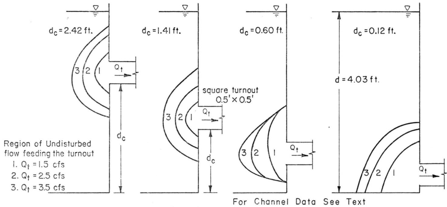
Figure 9. Regions of Undisturbed Channel Flow Feeding the Turnout for Different Turnout Settings and Discharges in Channel (11,11).
