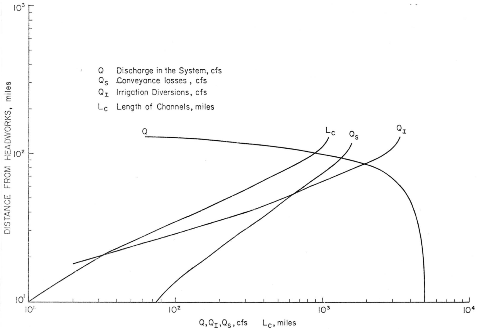
Figure 5. Discharge and Channel Length Variation with Distance from Headworks in the Simulated System.
