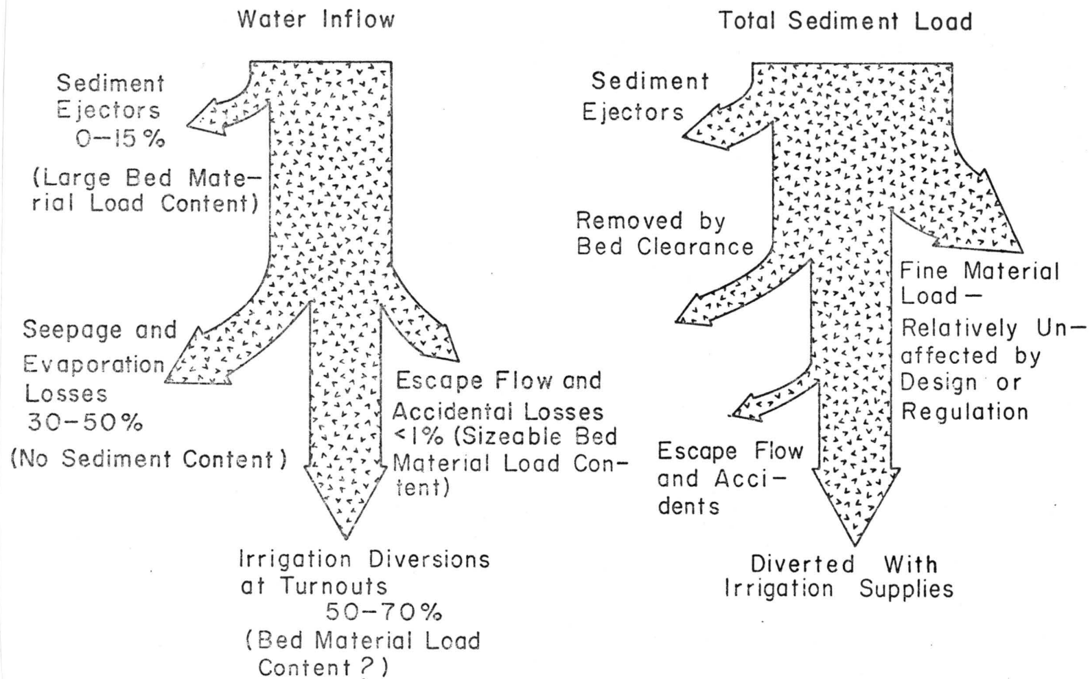
Figure 1. Schematic Distribution of Water and Sediment in Irrigation Canal Systems.
