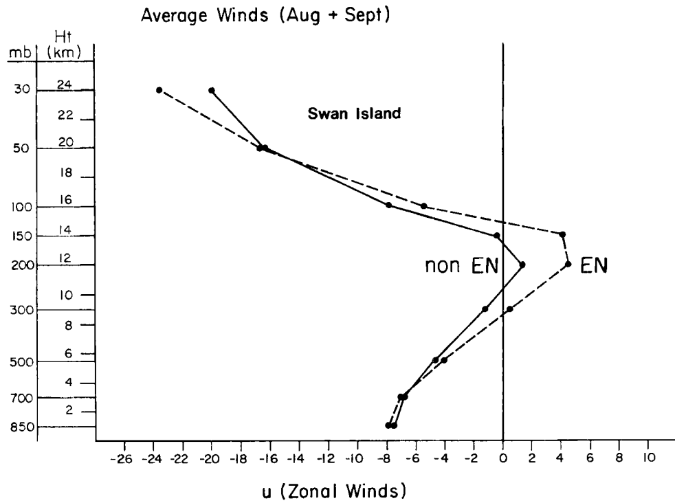
Fig. 24. Vertical profile of zonal wind during August and September at Swan Island (point 1 in Fig. 21) for an average of the last 5 El Niño years (1957, 1965, 1972, 1976 and 1982) - denoted EN- and 18 other non-El Niño years (non EN).
