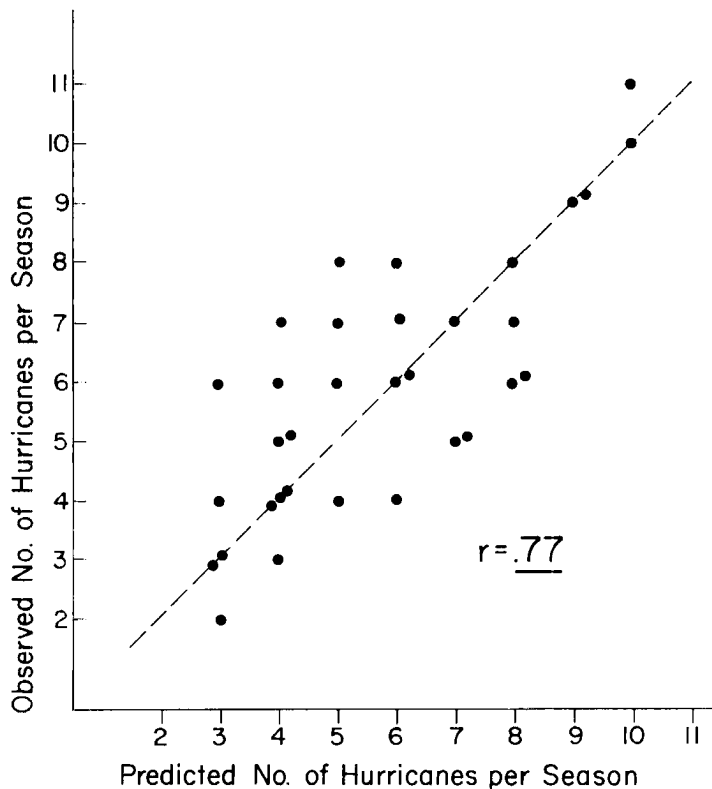
Fig. 11. Regression analysis of predicted vs. observed number of hurricanes per season for the period of 1950-1982 from the use of Eq. (1). The correlation coefficient is .77.
