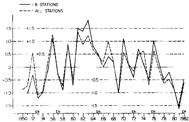
Fig. 1. Six-station average of Caribbean Basin SLPA for May (solid line). All station average is given by the dashed curve.
