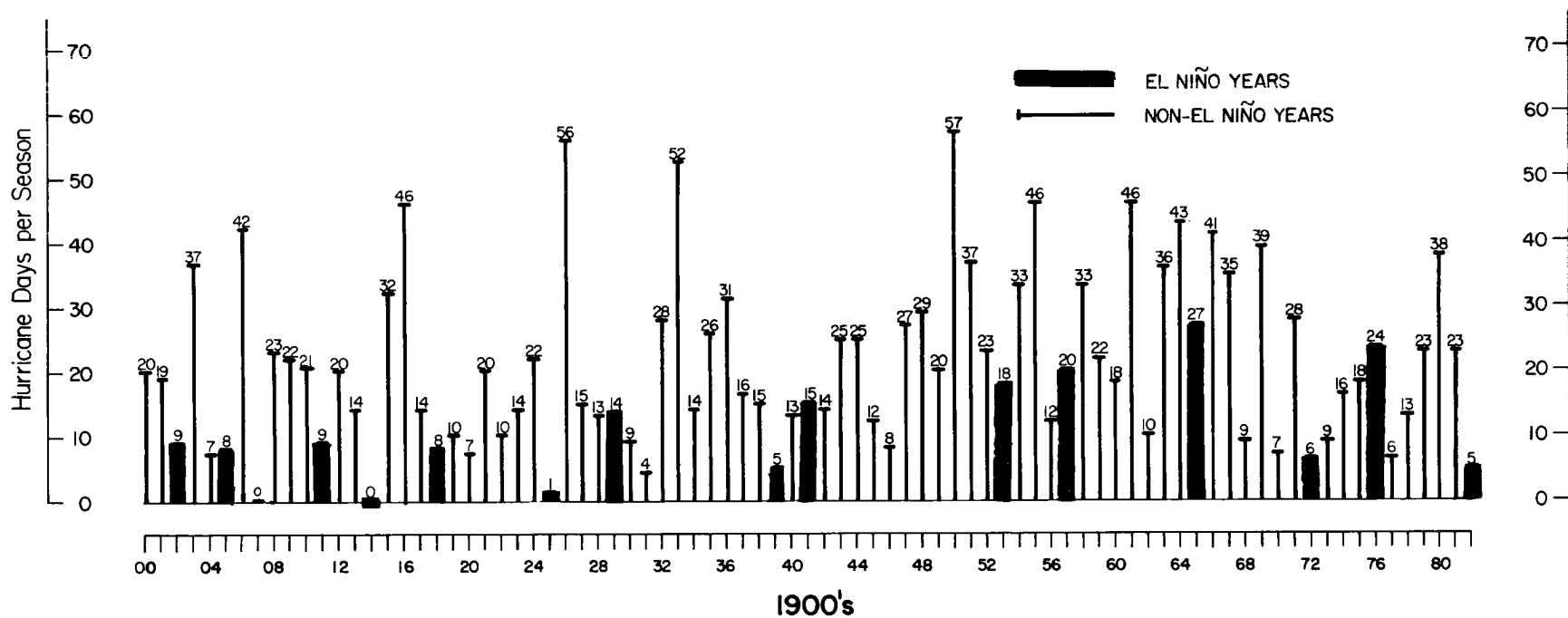
Fig. 2. Number of hurricane days (figure at top of lines) in El Niño and non-El Niño years from 1900-1982.
