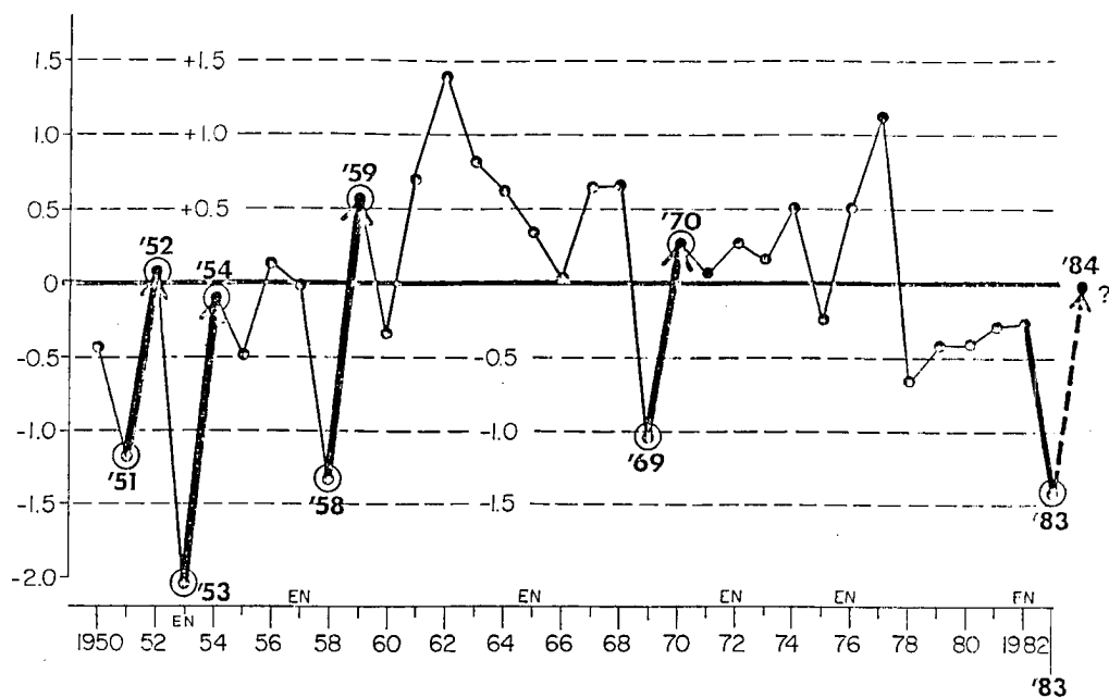
Fig. 2. Yearly variation of April-May mean Caribbean Basin SLPA for 6 standard stations.
