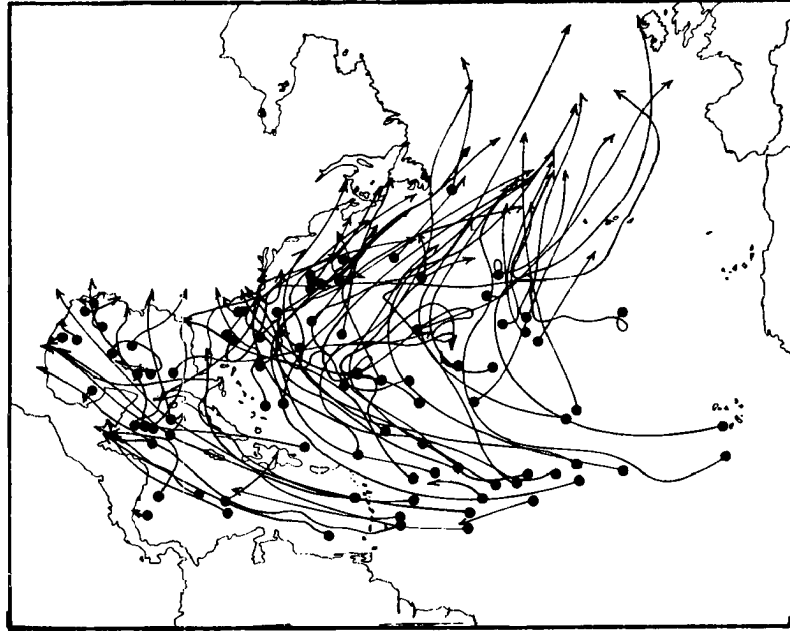
Fig. 32. Tracks of 12 non-El Niño years (1951, 1955, 1959, 1961, 1964, 1966, 1969, 1971, 1973, 1975, 1978, 1980) of hurricane intensity cyclones when seasonal 30 mb equatorial winds were from the west .
