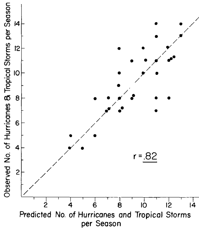
Fig. 12. Regression analysis of the predicted vs. observed number of hurricanes and tropical storms per season for the period of 1950-1982 from Eq. (2).
