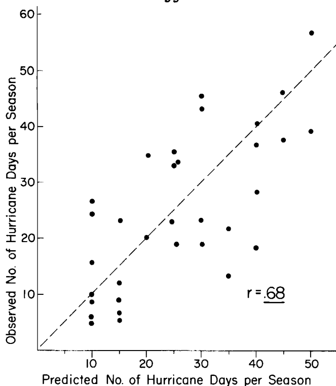
Fig. 13. Regression analysis of the predicted vs. observed number of hurricane days per season for the period of 1950-1982 from the use of Eq. (3).
