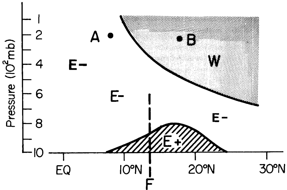
Fig. 23. Schematic north-south vertical cross section of zonal winds in the western Atlantic-Caribbean Basin in August-September relative to the typical latitudinal position of tropical cyclone formation indicated by the dashed line marked F. W and E stand for West and East winds respectively. + and - means strong and weak wind speeds respectively.
