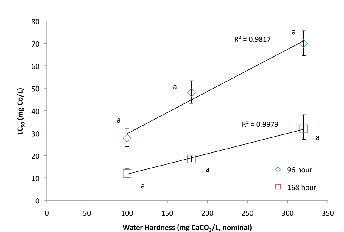
Figure 4.3.b. A comparison of LC 50 values from Study #2 and Study #3
