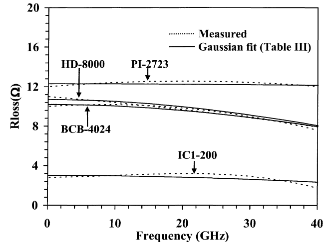
Figure 10. Dielectric loss equivalent resistance vs. frequency.
