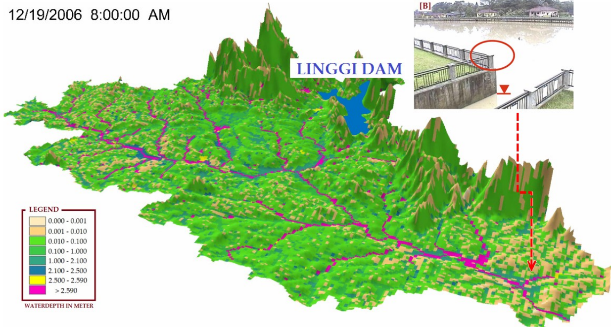
Figure 6.6 3-dimensional representation of the water depths at Kota Tinggi watershed on December 19, 2006 (adapted from Abdullah 2013)
