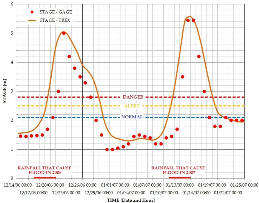
Figure 6.9 Hydrologic validations for large watershed using stage (adapted from Abdullah 2013)
