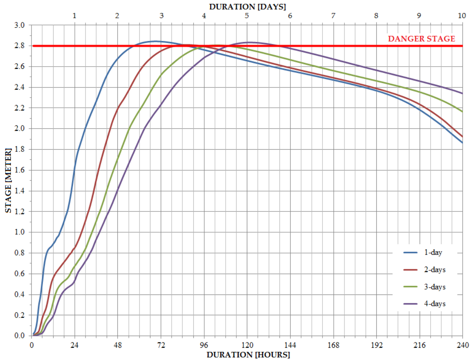
Figure 6.10 Stage hydrograph for 1-day and multi-day rainfall event
