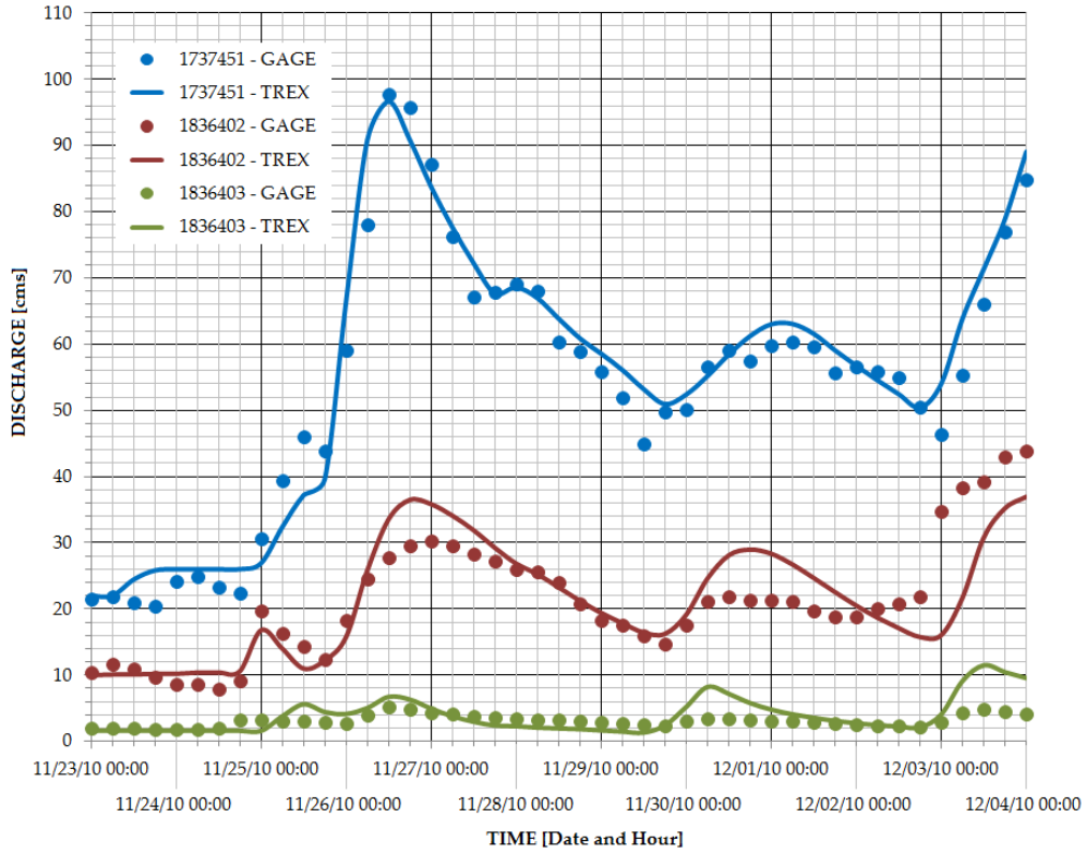
Figure 6.8 Hydrologic calibrations for large watershed (adapted from Abdullah 2013)
