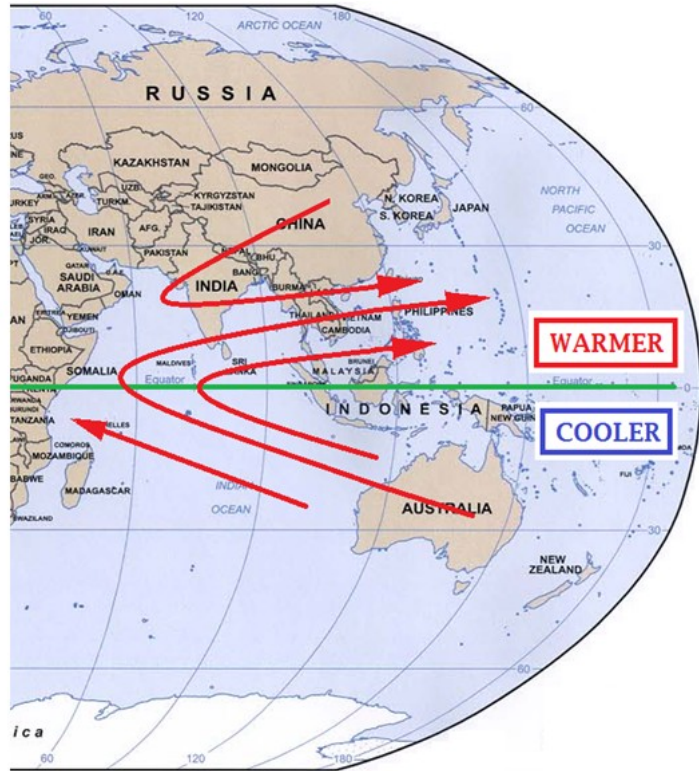
Figure 1.2 Mechanism of SW Monsoon (modified from Wang 2006)
