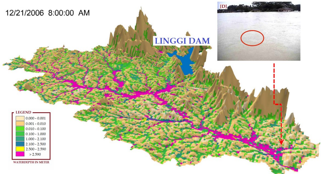
Figure 6.7 3-dimensional representation of the water depths at Kota Tinggi watershed on December 21, 2006 (adapted from Abdullah 2013)
