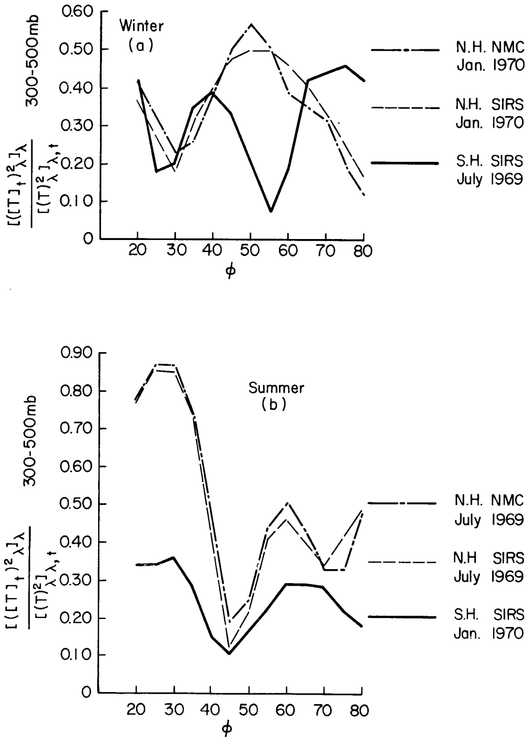
Fig. 4.6 Ratio of temperature variance due to standing eddies to total variance for the layer 300-500 mb; (a) winter, (b) summer.
