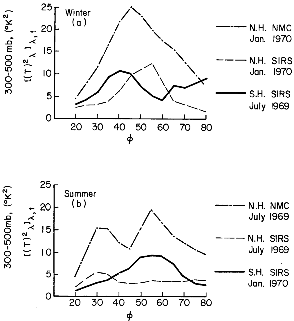
Fig. 4.4 Variance of temperature around latitude circles for the layer 300-500 mb in both hemispheres; (a) winter, (b) summer.
