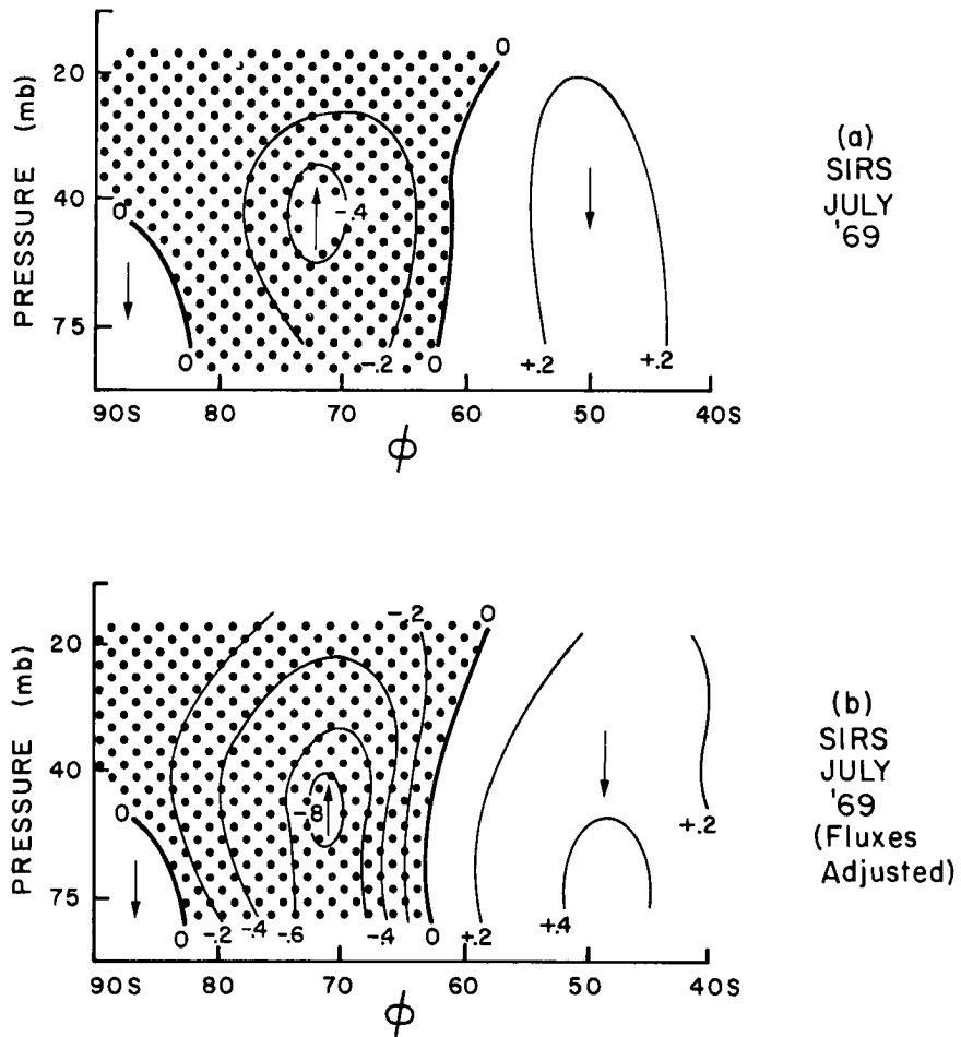
Fig. 5.10 Zonally-averaged vertical motion patterns for the S. H. for July 1969. Units: \text{mb day}^{-1} .
