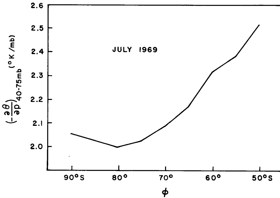
Fig. 5.3 Static stability ( -\frac{\partial\theta}{\partial p} ) in the layer 40-75 mb as a function of latitude in the Southern Hemisphere for July 1969. Values (except at 90°S) determined from SIRS data.
