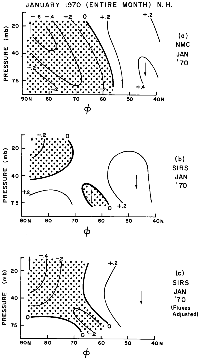
Fig. 5.9 Zonally-averaged vertical motion patterns for the N. H. for January 1970. Units: \text{mb day}^{-1} . Stippled area denotes area of ascent.
