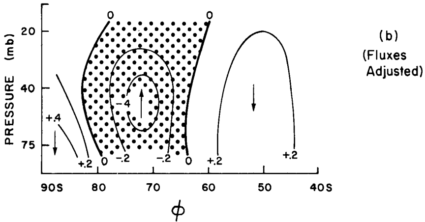
Fig. 5.14 Zonally-averaged vertical motion patterns for the S. H. for the period 18-27 July 1969, a quiet period. Units: \text{mb day}^{-1} .
