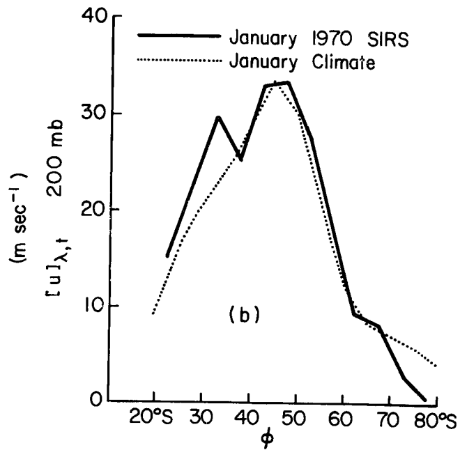
Fig. 4.3 Distribution with latitude of zonal mean geostrophic wind at 200 mb in the Southern Hemisphere for July and January.
