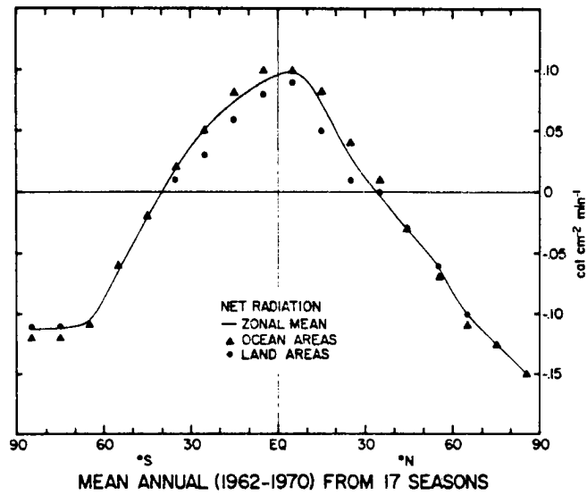
Fig. 2.1 Mean annual, satellite-based net radiation distribution (from Vonder Haar, 1972).
