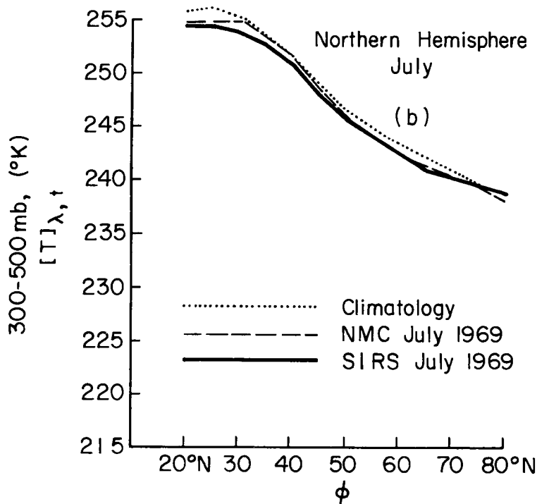
Fig. 4.1 Mean meridional temperature gradients in the upper troposphere (300-500 mb) in the Northern and Southern Hemispheres for January and July.
