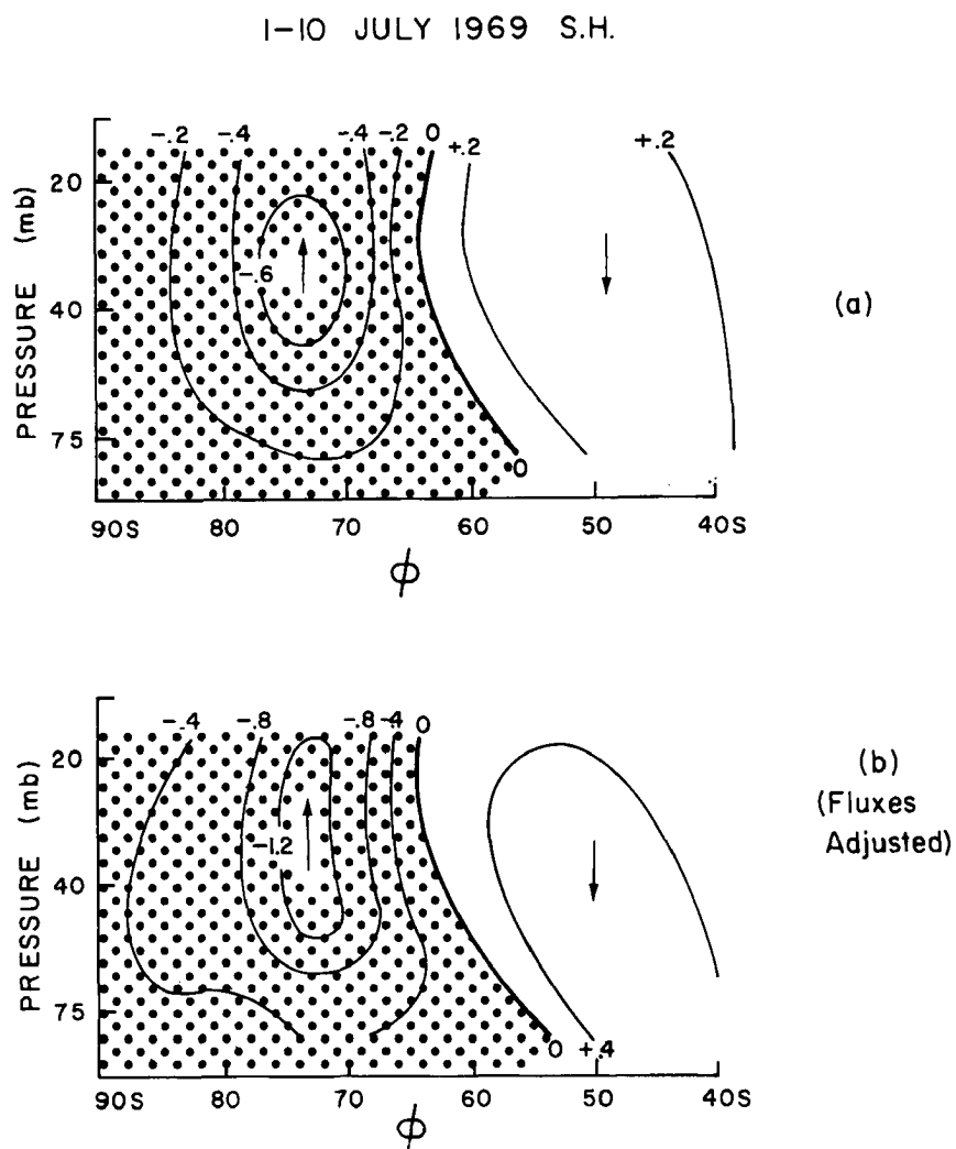
Fig. 5.13 Zonally-averaged vertical motion patterns for the S. H. for the period 1-10 July 1969, during a minor midwinter warming. Units: \text{mb day}^{-1} .
