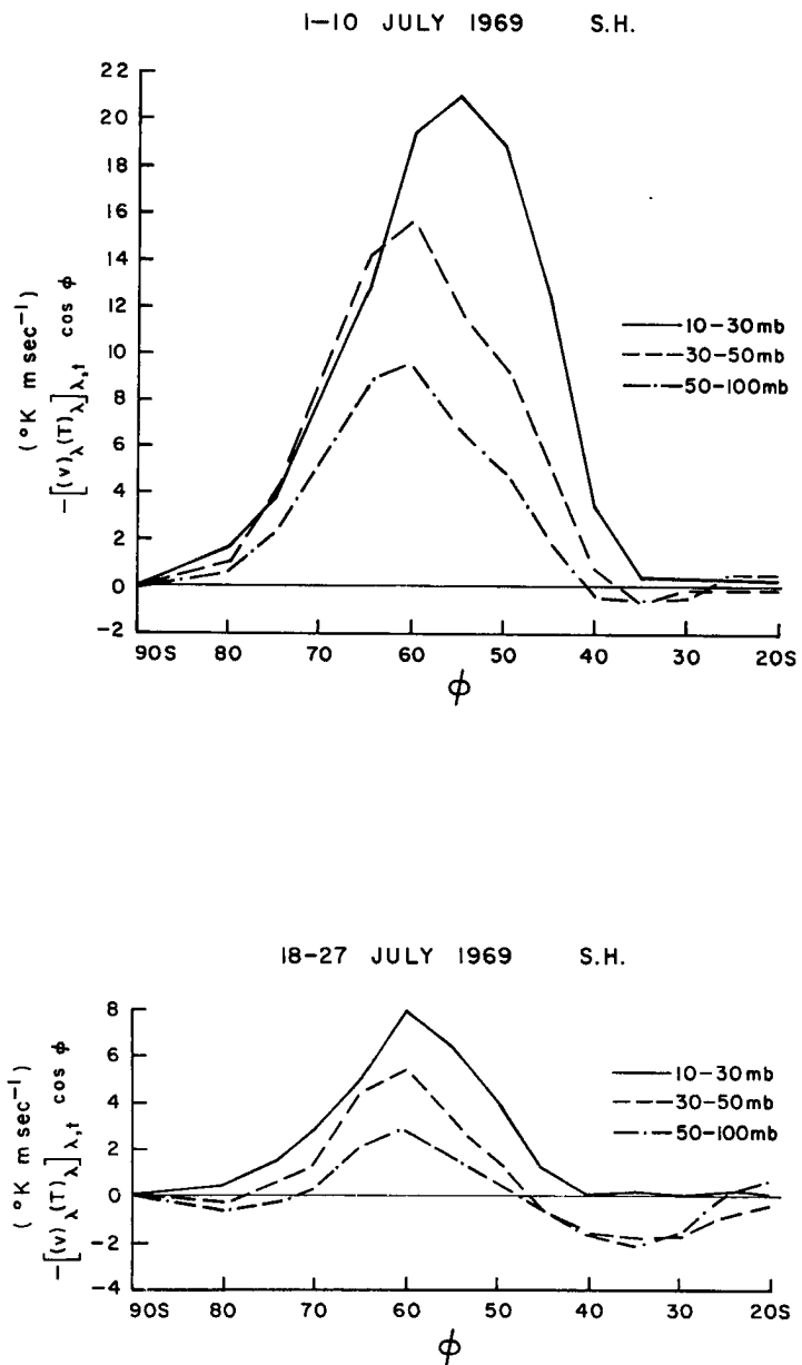
Fig. 5.15 Poleward heat fluxes in the S. H. during the periods (a) 1-10 July and (b) 18-27 July 1969.
