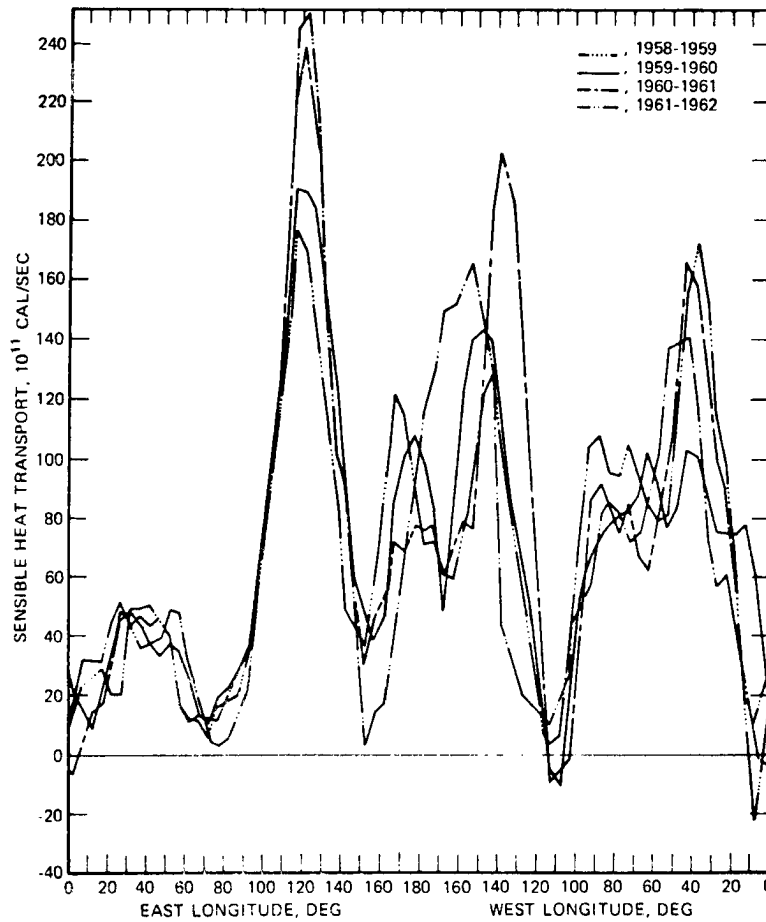
Fig. 4.11 Averages for four consecutive cold seasons (October-March) of contributions in each 5° longitude zone to poleward eddy heat transport across 45°N (from Haines and Winston, 1963).
