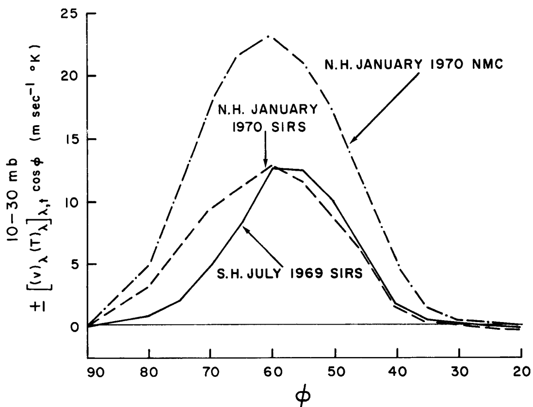
Fig. 5.7 Poleward heat flux in the 10-30 mb layer-January 1970 in the N. H., July 1969 in the S. H.
