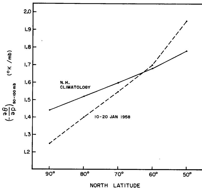
Fig. 5.1 Static stability (-\frac{\partial\theta}{\partial p}) in the layer 50-100 mb as a function of latitude in the Northern Hemisphere for January.
