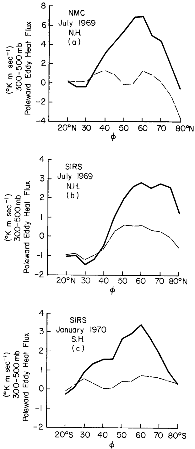
Fig. 4.10 Summertime, total poleward eddy flux of heat, \pm [(v)_\lambda(T)_\lambda]_{\lambda,t} (solid lines), and poleward eddy flux of heat due to standing eddies, \pm [([v]_t)_\lambda([T]_\lambda)]_\lambda (dashed lines) for the layer 300-500 mb in both hemispheres.
