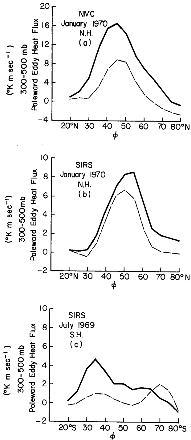
Fig. 4.9 Wintertime, total poleward eddy flux of heat, \pm [(v)_\lambda (T)_\lambda]_{\lambda,t} (solid lines), and poleward eddy flux of heat due to standing eddies, \pm [([v]_t)_\lambda ([T]_t)_\lambda]_{\lambda} (dashed lines) for the layer 300-500 mb in both hemispheres.
