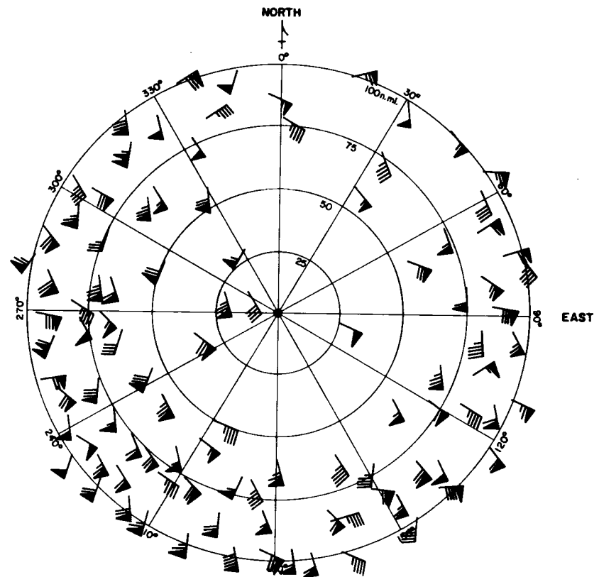
Fig. 16. Composite of all U. S. and Japanese proximity 850 mb wind soundings centered on the tornado.
