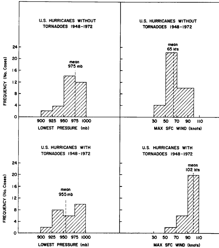
Fig. 12. A comparison of maximum surface winds and lowest sea level pressures for hurricanes with and without tornadoes at landfall. Mean values are indicated on each histogram.
