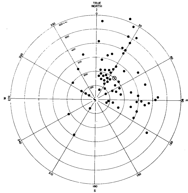
Fig. 6. Plan view display of 68 Japanese typhoon tornadoes (1950-1971) (Fujita et al., 1972) with respect to the typhoon center (S) and true north. \otimes refers to the centroid of all cases at 40^{\circ} azimuth, 200 n. mi. from the center of the typhoon.
