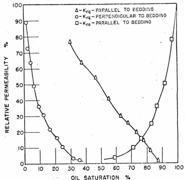
FIG. 3—RELATIVE PERMEABILITY OF ANISOTROPIC SANDSTONE.
