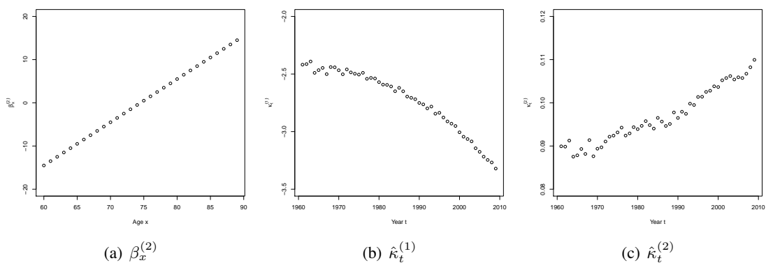
Figure 3: Parameters estimates for the Cairns-Blake-Dowd model for England and Wales (males) using yearly data from 1961-2009.
