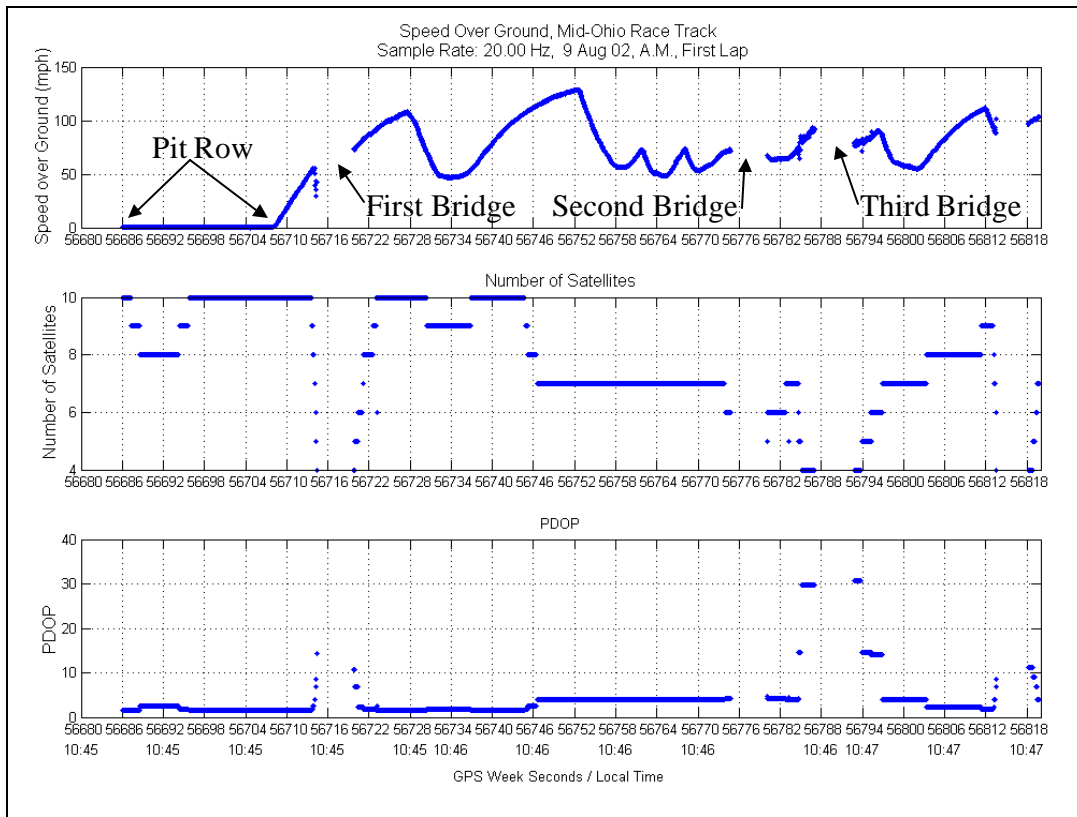
Figure 24. Effects of Ground Speed, Number of Satellites Tracked, and PDOP
