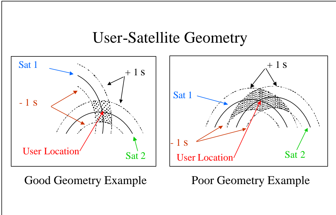
Figure 8. User-Satellite Geometry [22]
