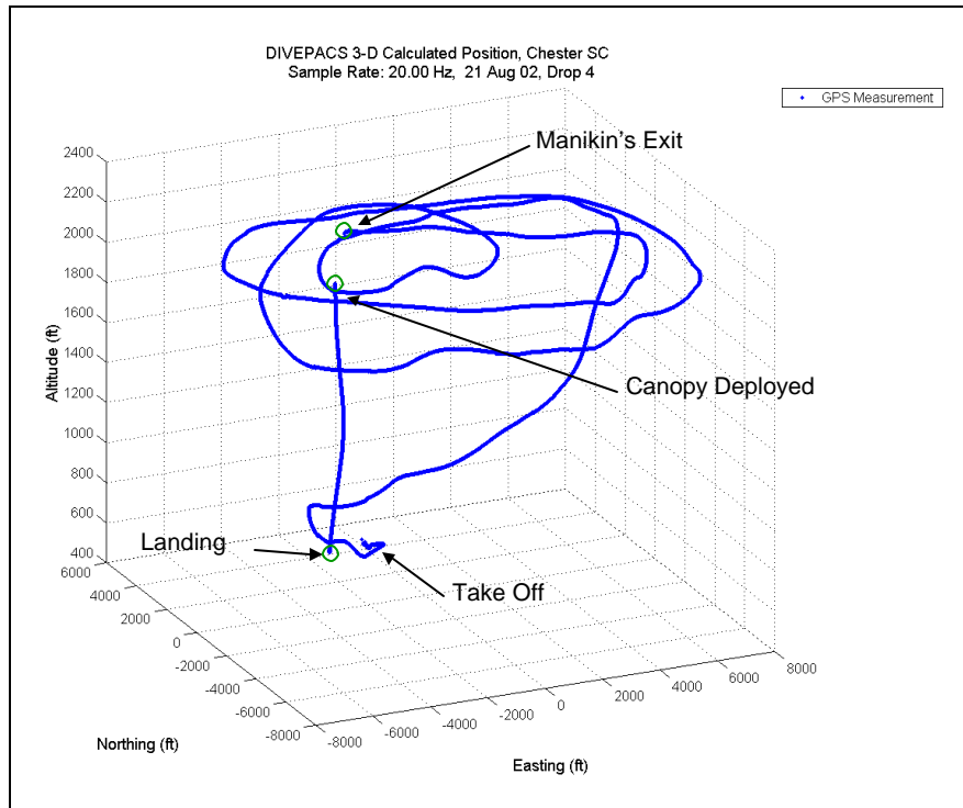
Figure 31. Manikin Drop 4 Three-dimensional View
