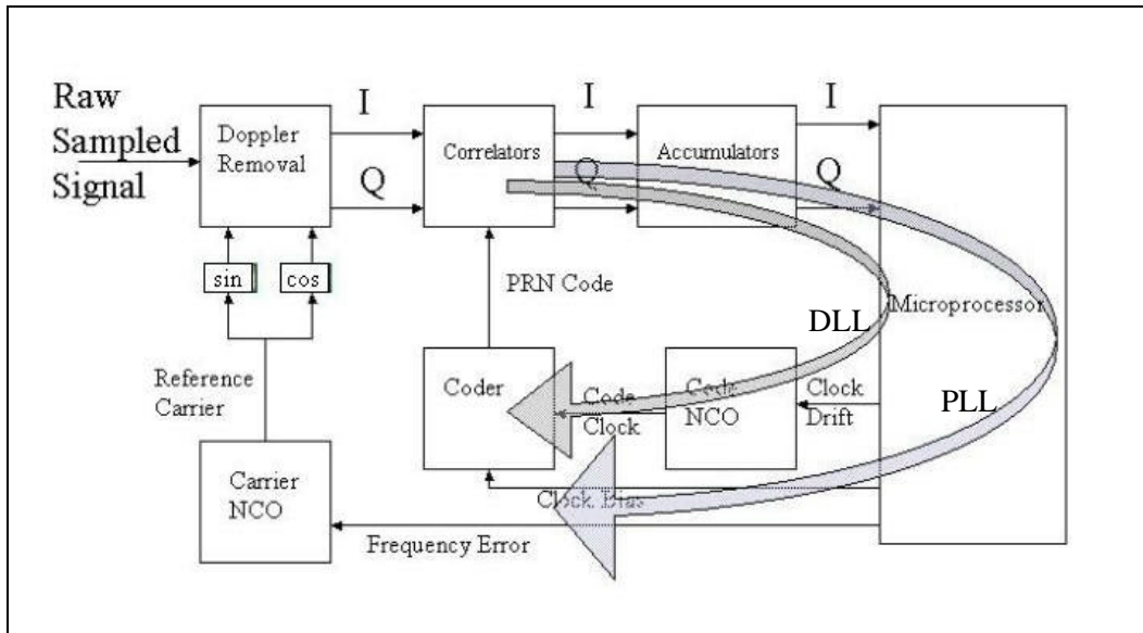
Figure 9. Tracking Loops [29]
