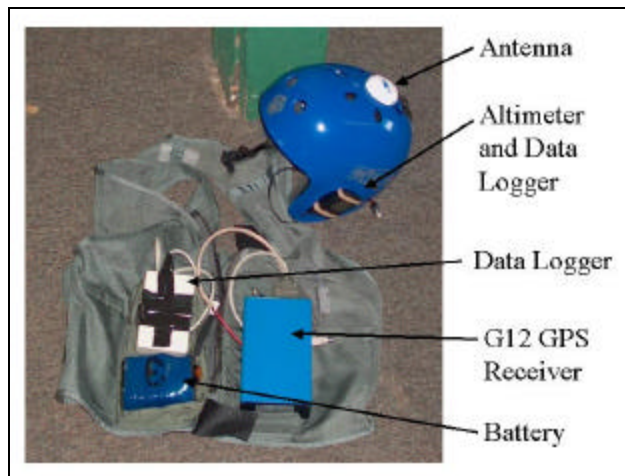
Figure 4: DIVEPACS configured for freefall testing
