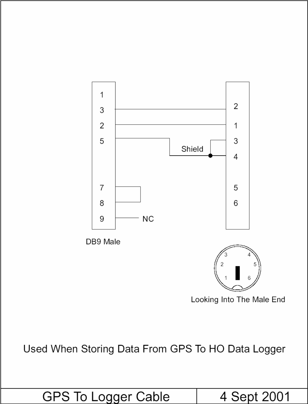
Figure 46. GPS to Logger Cable
