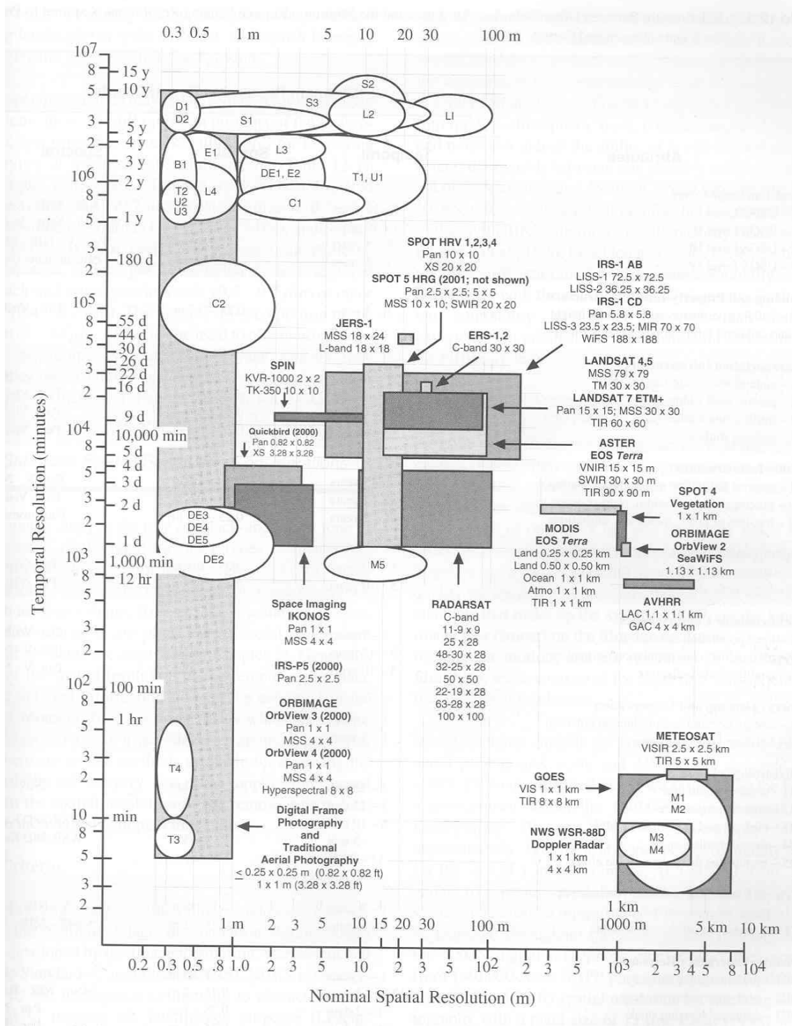
Figure 4-1: Diagram of Resolutions (Jensen and Cowen, 1999:613).
