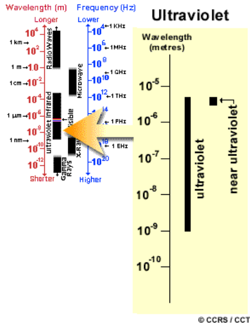
Figure 2-8: Ultraviolet (Fundamentals of Remote Sensing, 2002)
