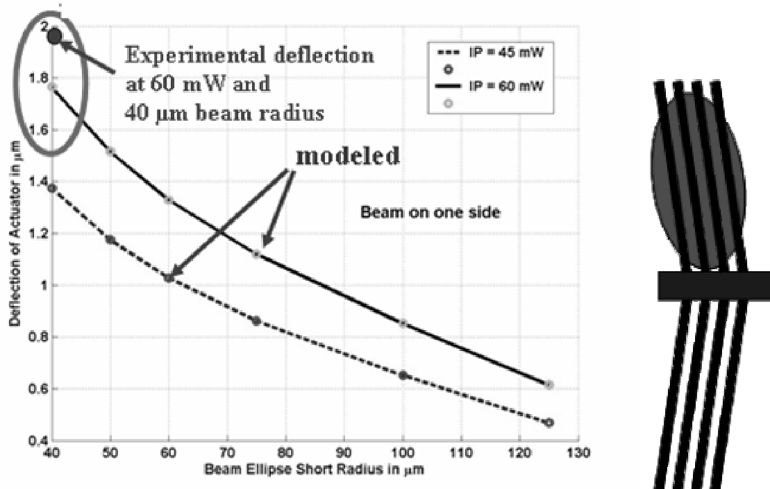
Figure 7.20: Plot showing the model predicted deflection versus laser beam dot size with the beam asymmetrical heating one side of actuator and giving almost 2 \mu\text{m} of deflection at 60 mW of incident power and a 40 \mu\text{m} beam dot radius.
