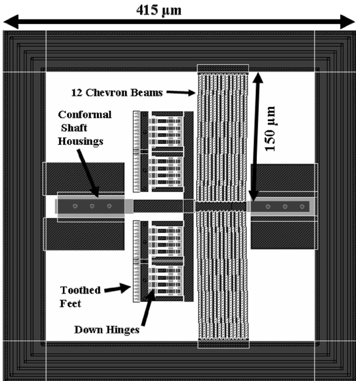
Figure 8.1: L-Edit design layout of the 415 by 415\ \mu\text{m} LR-150-12 microrobot, incorporating several design optimizations; including twelve 150\ \mu\text{m} long chevron actuator beams, placed only 2\ \mu\text{m} apart.
