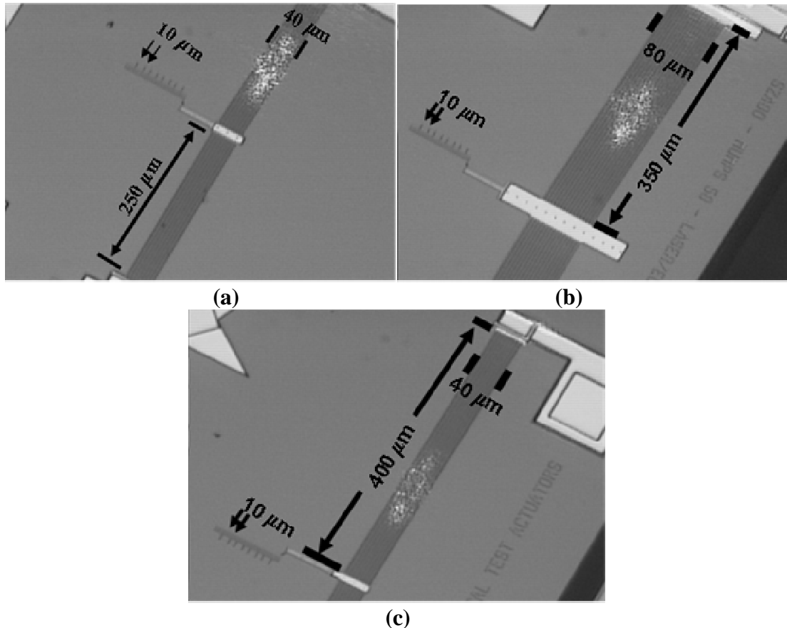
Figure 4.9: Digital photographs, showing PolyMUMPs 58 test actuators under laser testing, with (a) 250\ \mu\text{m} by 8-beam chevron, (b) showing a 350\ \mu\text{m} by 16-beam chevron and (c) showing a 400\ \mu\text{m} by 8-beam chevron.
