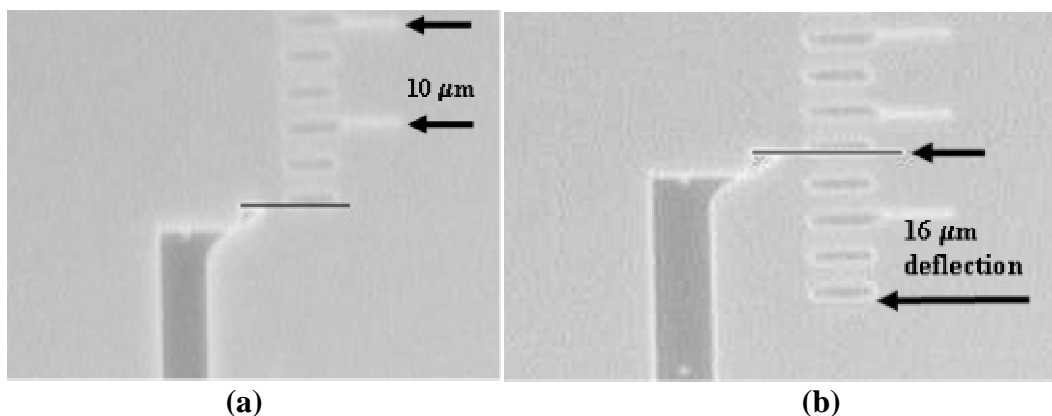
Figure 7.2: Digital images of the PolyMUMPs 58 Chevron 350 \mu\text{m} by 16-beam chevron test actuator under electrical test, with (a) being the pointer position showing a barely discernible deflection of .25 \mu\text{m} at 1 volt and (b) showing a maximum deflection of at 16 \mu\text{m} at 16 volts.
