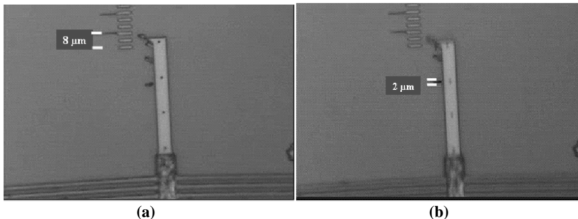
Figure 7.17: Captured still digital video images from digital video of the effects of frequency on the magnitude of deflection, with (a) showing 8\ \mu\text{m} of deflection at 61 Hz and (b) showing 2\ \mu\text{m} of deflection at 2 kHz.
