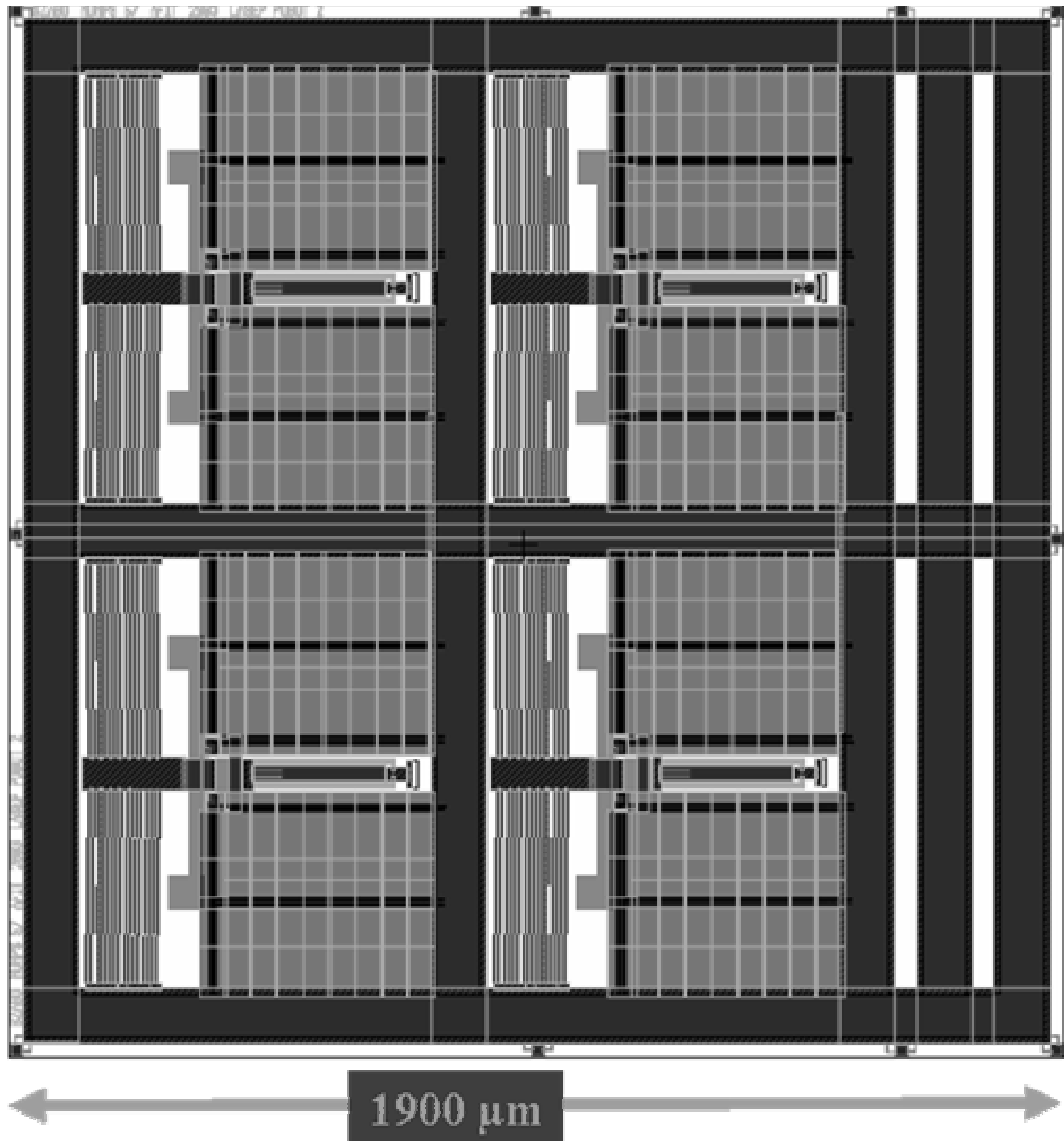
Figure A1.9: L-Edit layout showing the PolyMUMPs 57 microrobot design; an optothermal chevron microrobot design with a 1900 by 1900 \mu\text{m} size, four, 350 \mu\text{m} long chevron actuators with 16 chevron beams, and with four, 250 \mu\text{m} long down thermal actuators.
