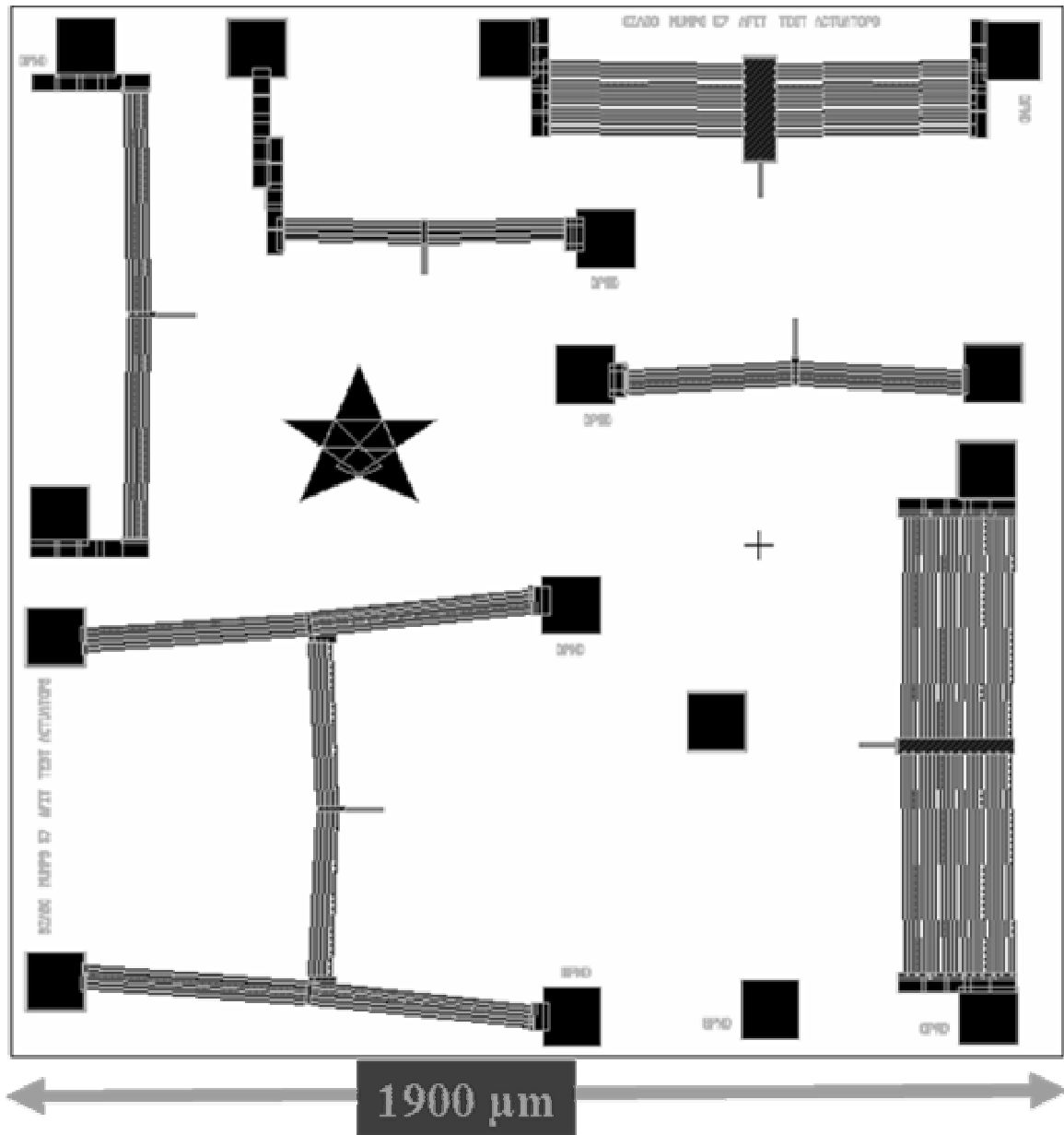
Figure A1.14: L-Edit layout showing the PolyMUMPs 57 test actuator design chip; with 250 μm, 350 μm, and 400 μm long chevron actuators with 4, 16 and 24 chevron beams. They can be tested both electrothermally and optothermally.
