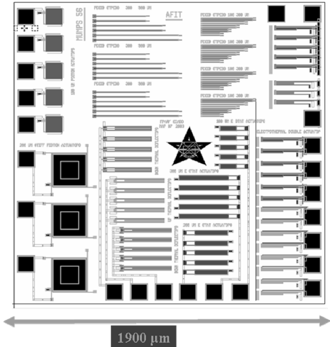
Figure A1.15: L-Edit layout showing the PolyMUMPs 56 test actuator design chip; with 250 \mu\text{m} long double hot arm actuators, up and down thermal actuators, gold dot tests double hot arm actuators, electrostatic actuators and residual stress structures. These residual stress structures were used in this research as calibration marks for aligning the laser beam dot size.
