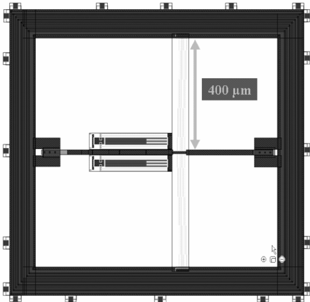
Figure A1.2: L-Edit layout showing the PolyMUMPs 58 microrobot design; the LR400-8 microrobot with a 990 by 1120 \mu\text{m} size, 400 \mu\text{m} long chevron actuators with 8 chevron beams, and with two, 250 \mu\text{m} long down thermal actuators.
