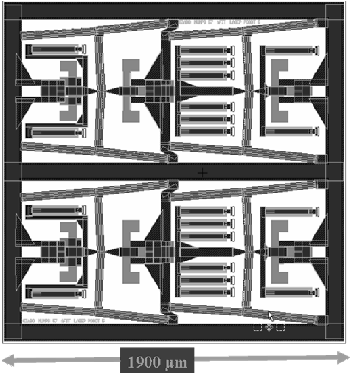
Figure A1.7: L-Edit layout showing the PolyMUMPs 57 microrobot design; a cascade-microrobot design with a 1900 by 1900 μm size, 400 and 300 μm long chevron actuators with 4 chevron beams, and with twenty, 250 μm long down thermal actuators. It also has detachable tabs for under-over drive shaft housings.
