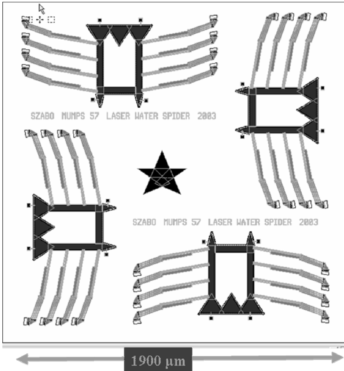
Figure A1.11: L-Edit layout showing the PolyMUMPs 57 microrobot design; the Laser Water Spider with a 1250 by 560 μm size, and eight, 250 μm long, double hot arm actuators, and 200 μm long bimorph down thermal actuators mounted at the end of the double hot arm actuators.
