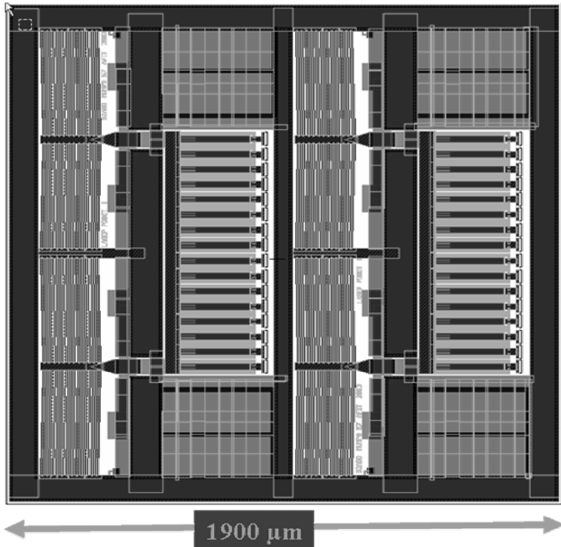
Figure A1.10: L-Edit layout showing the PolyMUMPs 57 microrobot design; an optothermal chevron microrobot design with a 1900 by 1900 \mu\text{m} size, 4, 400 \mu\text{m} long chevron actuators with 20 chevron beams, and with thirty-two, 250 \mu\text{m} long down thermal actuators.
