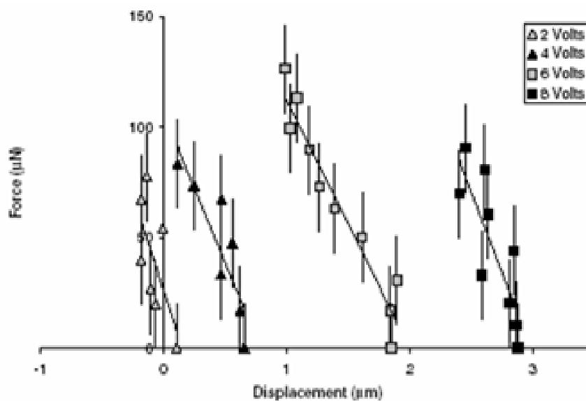
Figure 7.16: Plot of the force versus deflection Lai, et al. obtained for their 8 \times 150 \mu\text{m} chevron actuator designs. [2].
