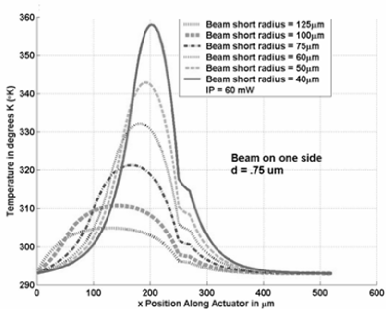
Figure 5.17: Plot showing the temperature distribution in chevron actuator arms with the actuator closer to surface, as would happen with a released microrobot.
