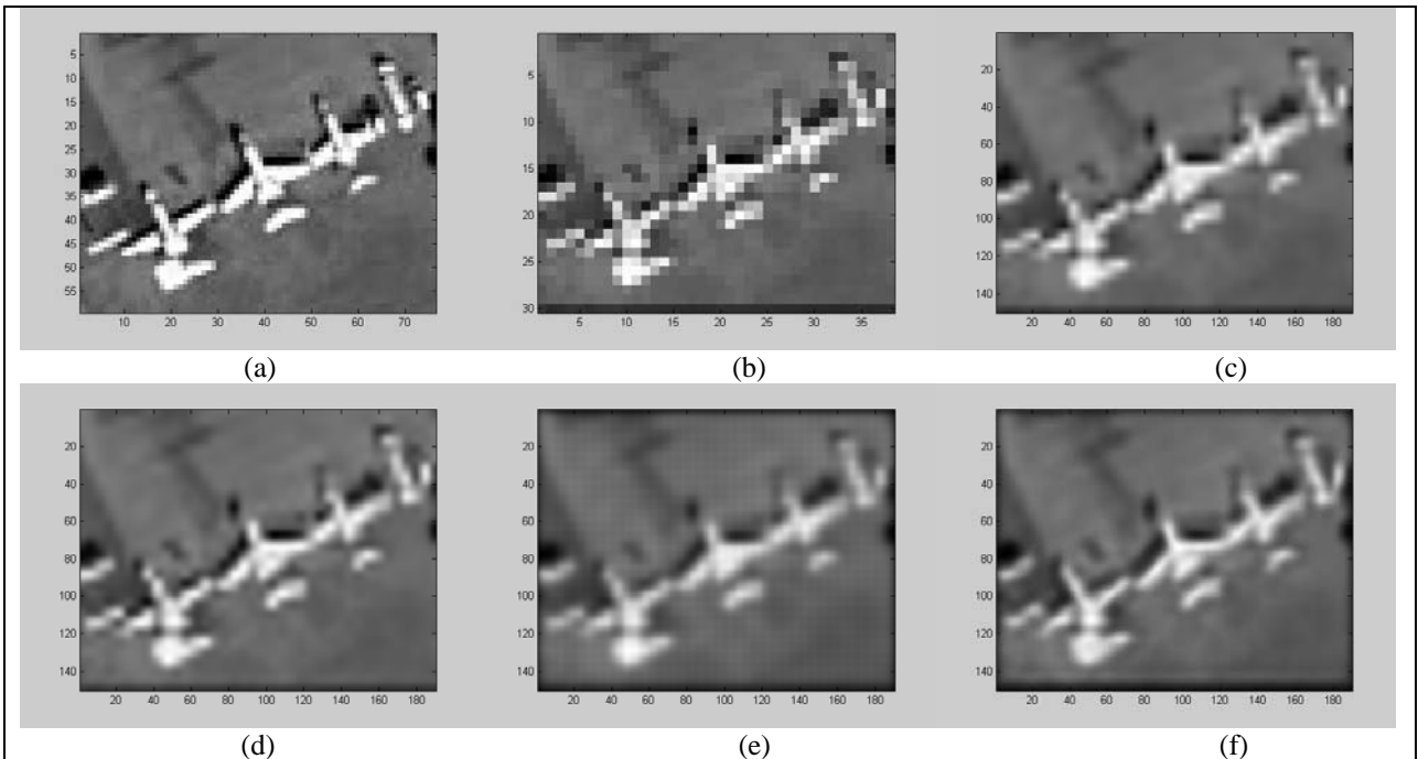
Figure 40. Interpolation results using the Airplane image. (a) Original image, (b) Image degraded using a low pass filter, (c) Bilinear interpolation, (d) Bicubic interpolation, (e) Gaussian radial basis function interpolation, (f) Adaptive Gaussian Interpolation.
