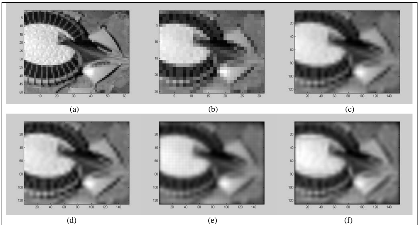
Figure 39. Interpolation results using the Stadium image. (a) Original image, (b) Image degraded using a low pass filter, (c) Bilinear interpolation, (d) Bicubic interpolation, (e) Gaussian radial basis function interpolation, (f) Adaptive Gaussian Interpolation.
