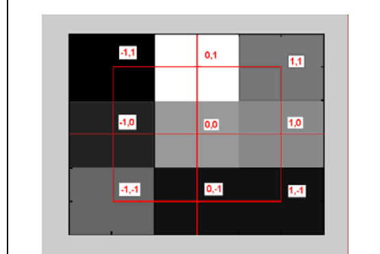
Figure 13 Window coordinate system, in which dark colors represent low numbers and lighter colors represent higher numbers; thus the data is centered slightly to the top right of the center of the window.
