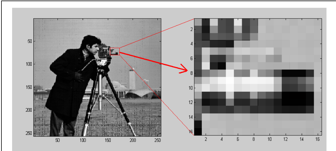
Figure 9 An example of a use of AGI, where a small portion of an image in which interesting or critical information exists is heavily magnified. The algorithm is executed on this small portion. The program takes approximately 30 seconds to interpolate the small portion of the image using a 2.8Ghz Pentium 4 processor with 1GB RAM and MATLAB software [6].
