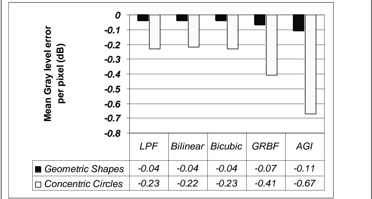
Figure 44 As in Figure 43 but for geometric images.
