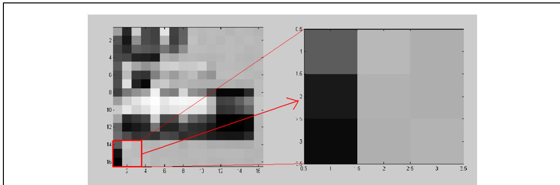
Figure 10 This figure demonstrates the method by which the image is analyzed one window at a time. A 3x3 (9 pixel) window creates a 2-D gaussian using a least squares fit. The pixel in the center of the 3x3 window is the pixel to be interpolated and replaced by a Gaussian.
