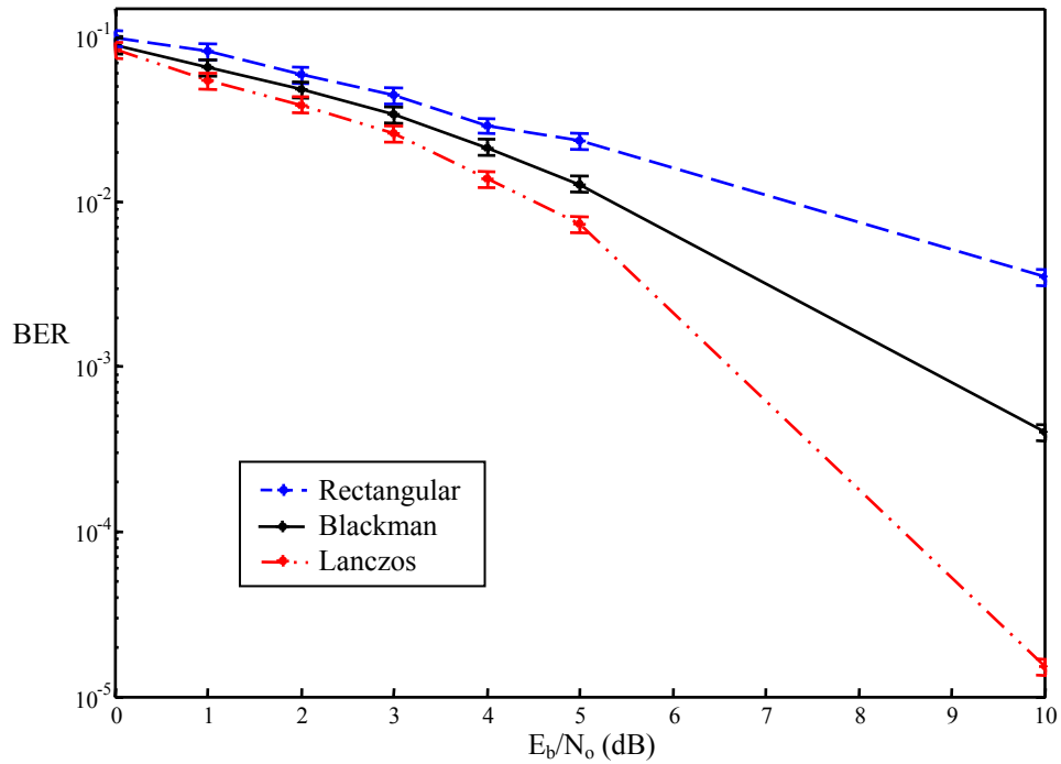
Figure 4.17. BER for Asynchronous Best-Case Gold Coded DS/SSMA System with K = 9 Users, N = 31 Length Codes and Chip Waveform Shaping.
