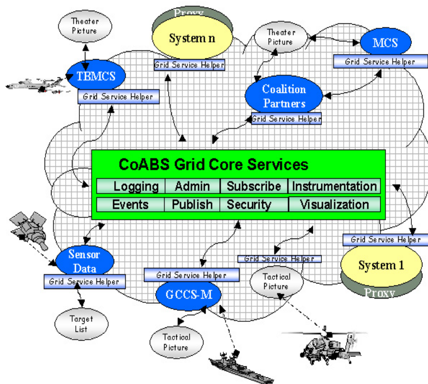
Figure 2-4. CoABS Grid [11].
