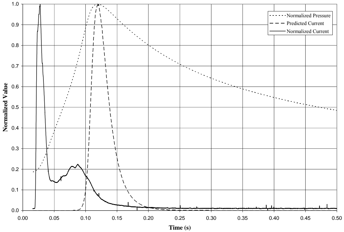
Figure 21. Saitzkoff et al. model applied to this experiment at baseline condition of 3 atm initial pressure and \varphi = 1.0
