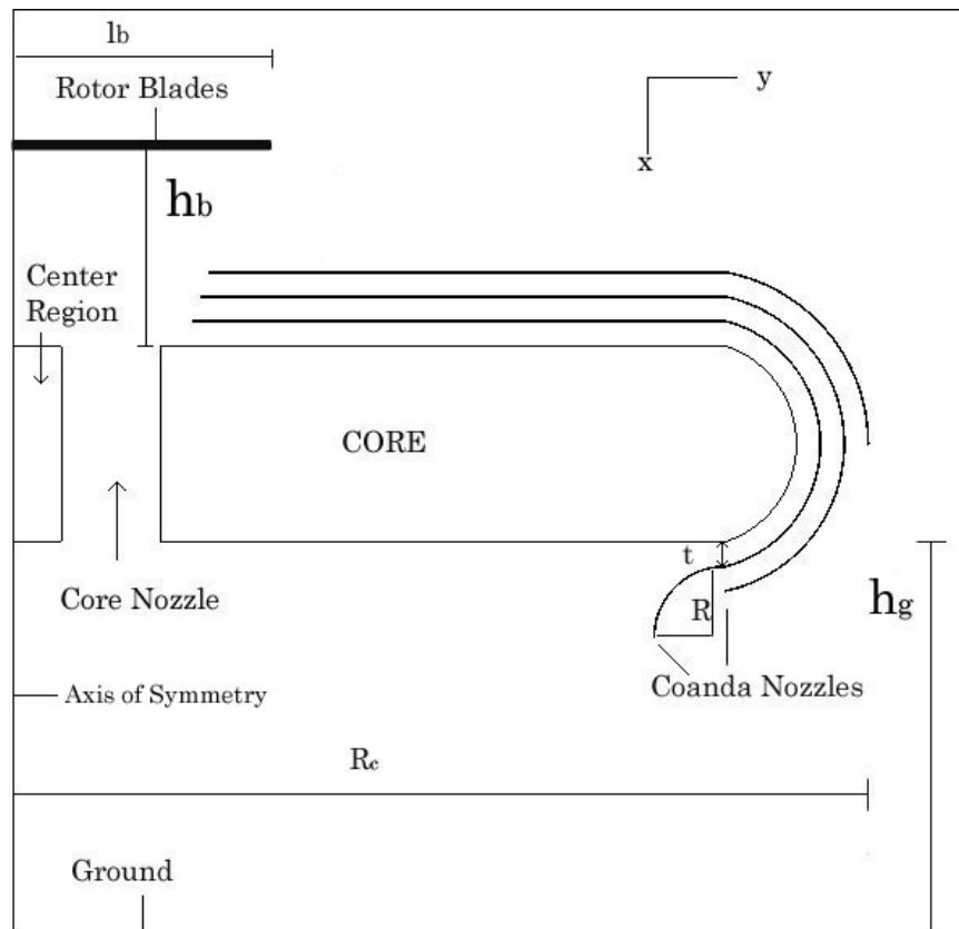
Figure 3: Schematic of the First Design
