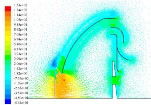
Velocity Vectors Colored By Axial Velocity (m/s) (Time=1.5000e-01) Dec 19, 2003 FLUENT 6.1 (axi, dp, segregated, lam, unsteady)
