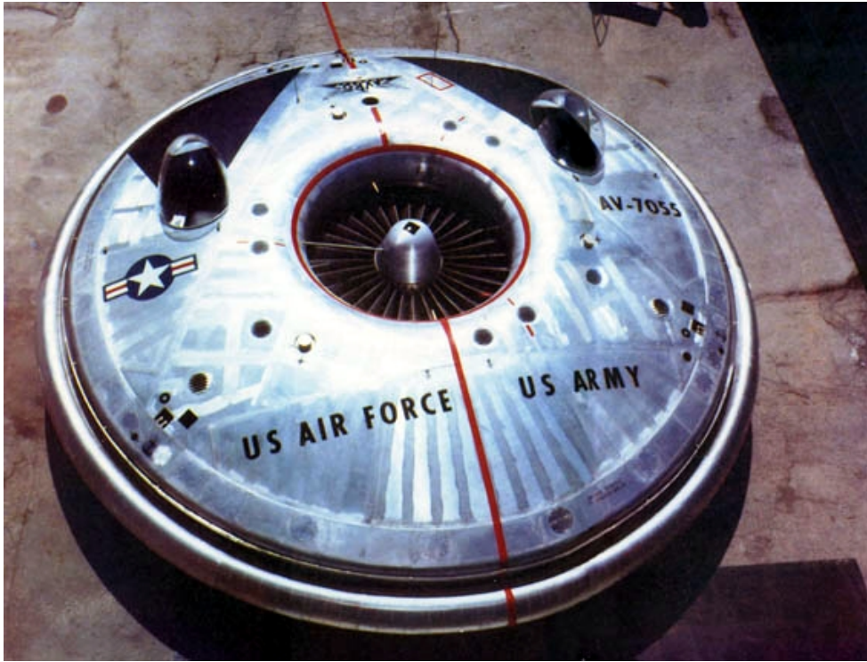
Figure 1: Full Scale AVRO Car
