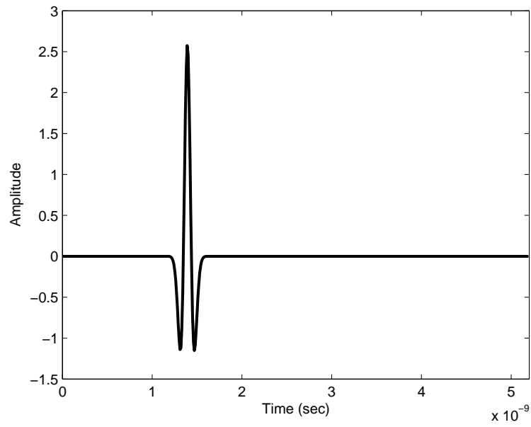
Figure B.1 UWB ChRx Input Signal
