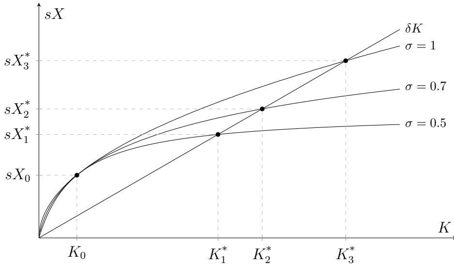
Figure 3: Development of sX and the steady-state capital stock K^* for different values of \sigma
