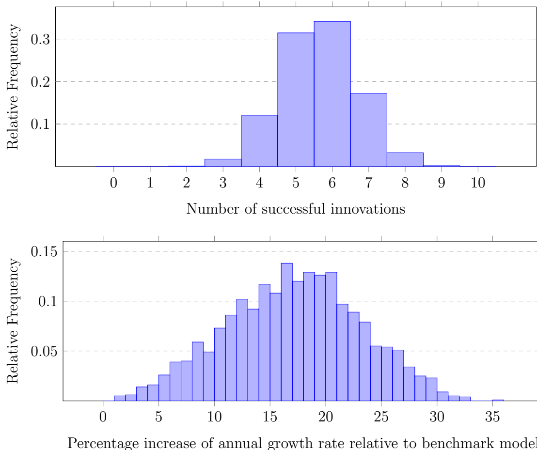
Figure 5: Number of successful innovations and percentage increase in average annual growth rate relative to benchmark model over 2,000 simulation runs
