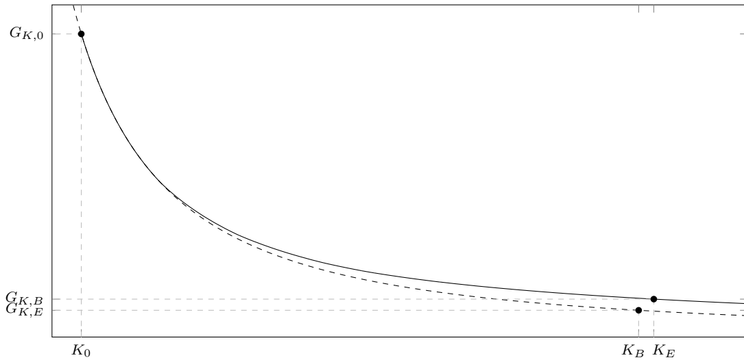
(b) Development of marginal product G_K
