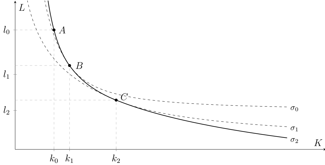
(a) Development of the unit isoquant curve
