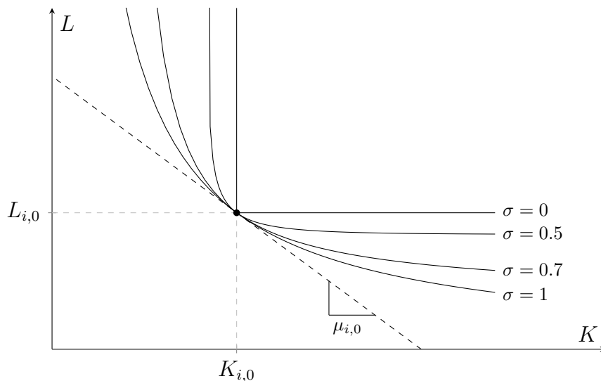
Figure 1: Family of isoquant curves for the normalized intermediate CES production function (2)
