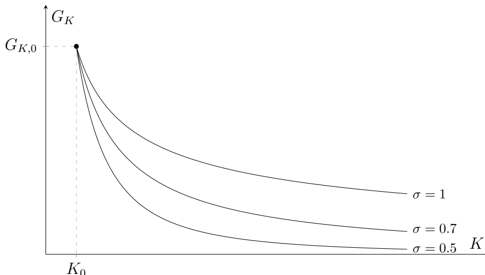
Figure 2: Development of G_K for different values of \sigma
