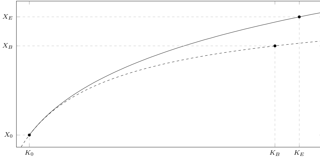
(a) Development of final output X
