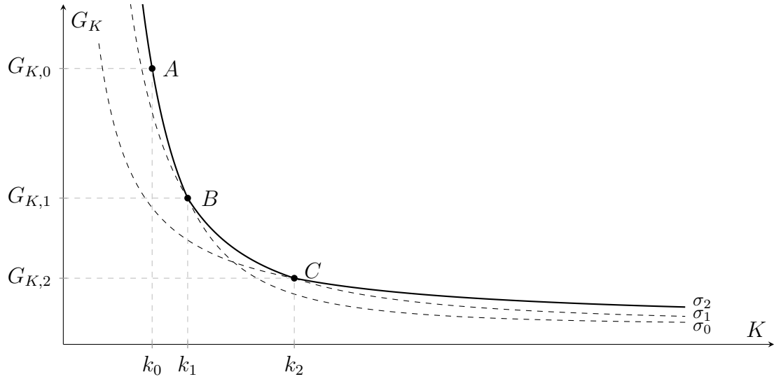
(b) Development of G_K
