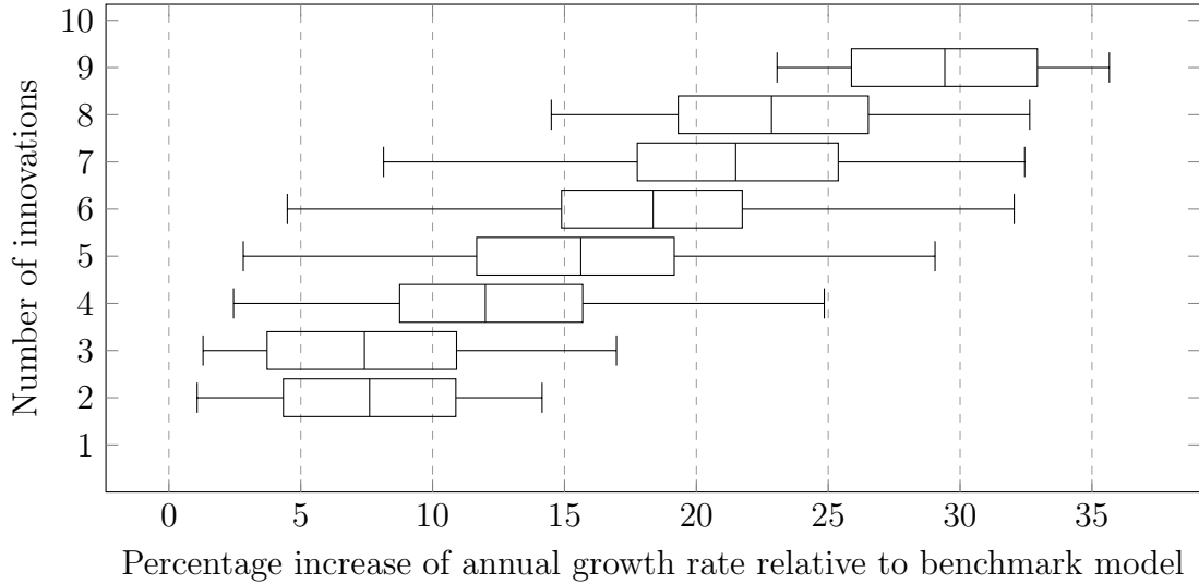
Figure 6: Boxplot for each number of successful innovations
