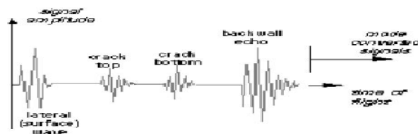
Gambar 1. Sinyal pantul ultrasonik (A-scan) [3]
