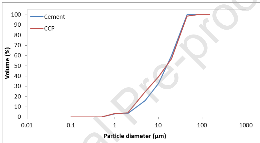
Figure 1: The particle size distribution of cement and CCP.
