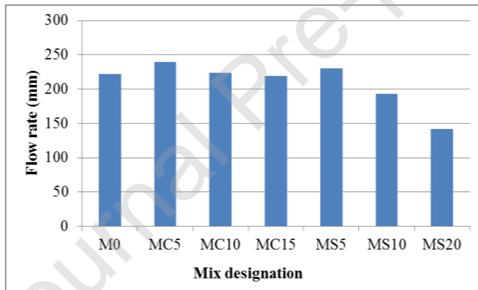
Figure 5: Flow rate results of mortar mixtures at 28-day.
