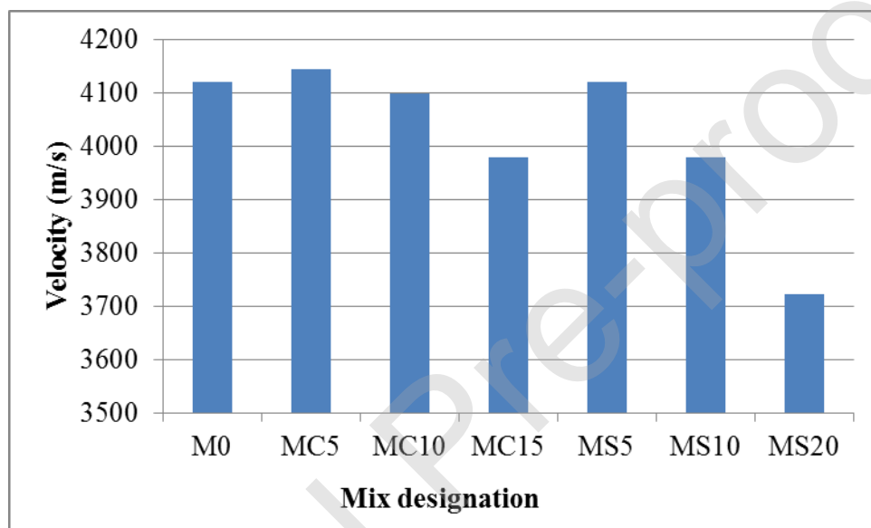
Figure 9: UPV results of mortar mixtures at 28-day.
