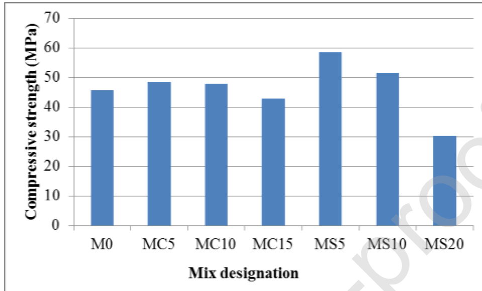
Figure 6: Compressive strength results of mortars at 28 days.
