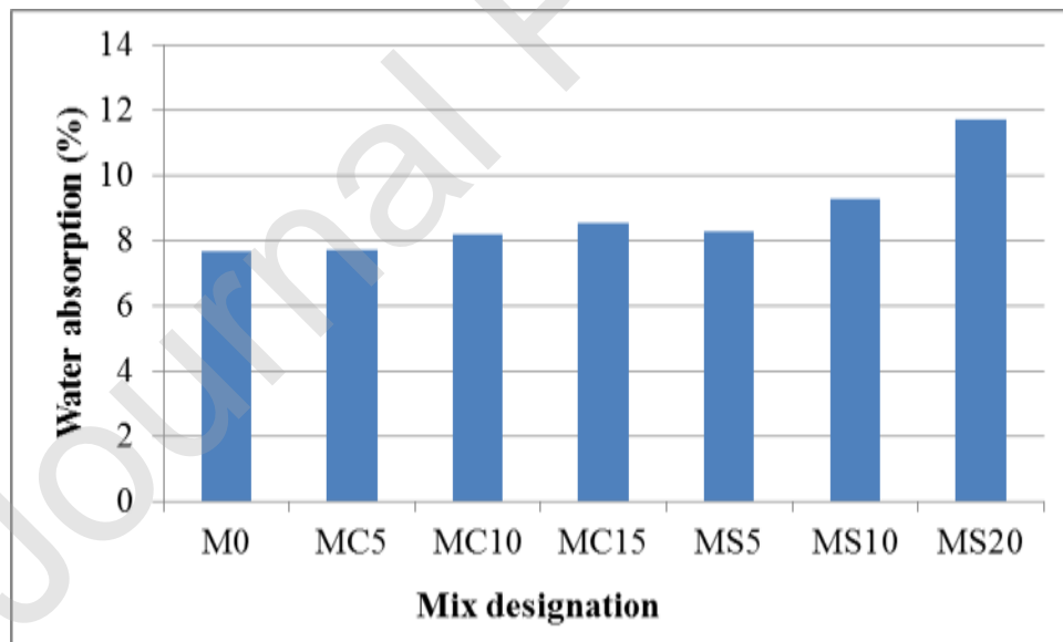
Figure 7: Water absorption results of mortars at 28 days.
