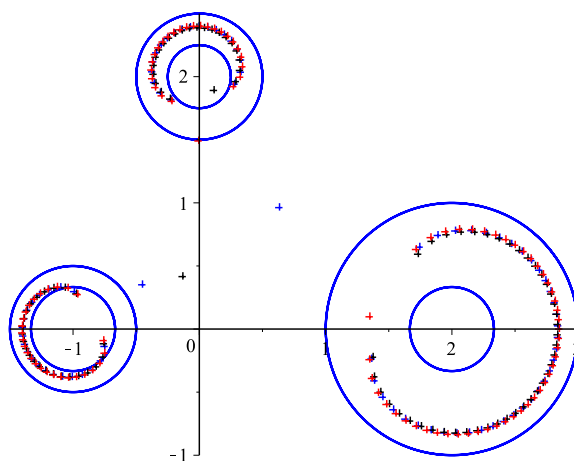
FIGURE 7. Zeros of the polynomials p_n(G^*, z) of Example 5.2, for n = 80, 90 and 100 .
