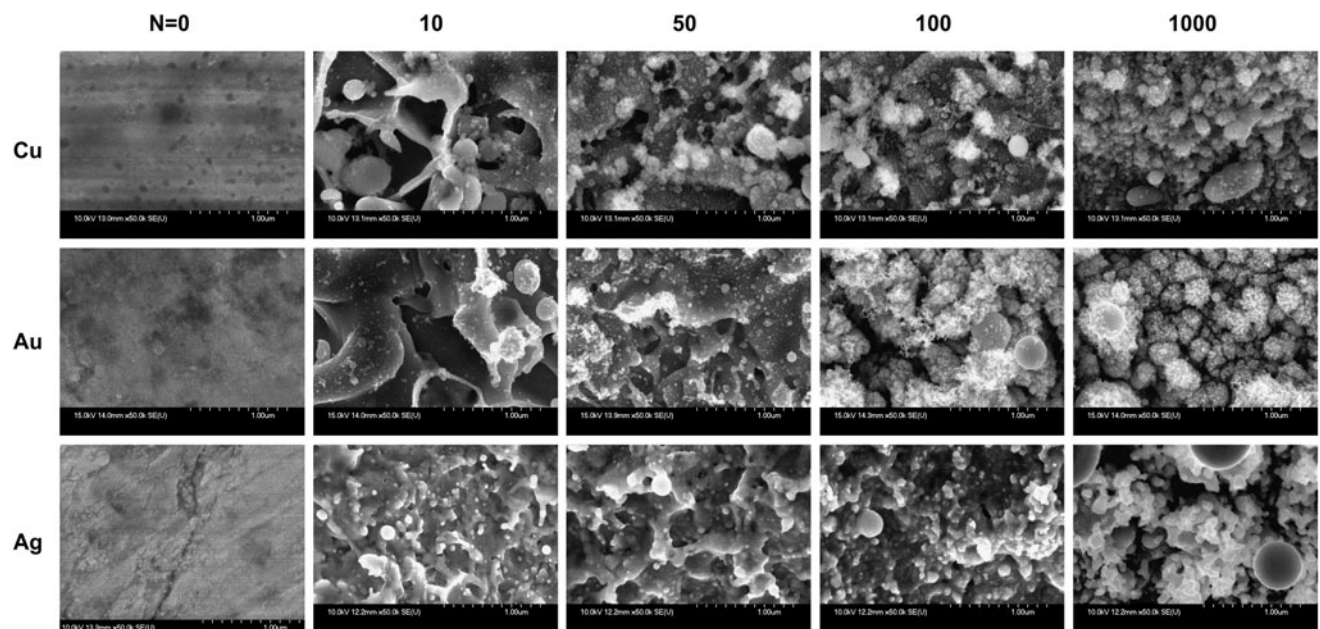
Fig. 5 Electron microscopic images of the metal surfaces irradiated with different numbers of laser pulses of 190 \text{ mJ/cm}^2 fluence
