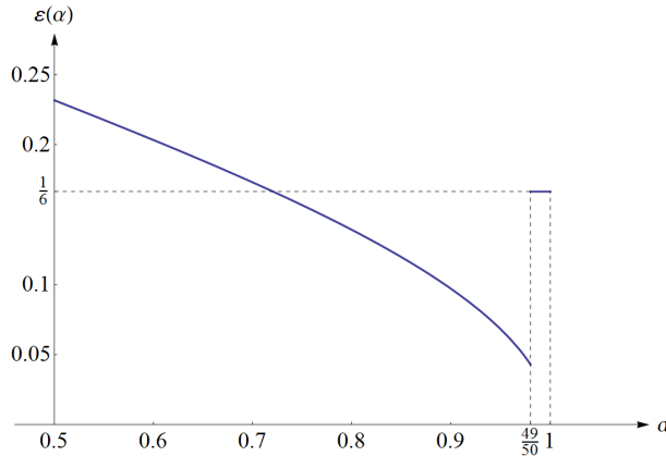
FIGURE 6. U(\alpha) is the square with sides 2\varepsilon(\alpha) , centered at (0, 0) . \varepsilon(\alpha) is obtained from Theorem 4.3 for \alpha \in [\frac{1}{2}, \frac{49}{50}] and from Theorem 4.4 for \alpha \in [\frac{49}{50}, 1] .
