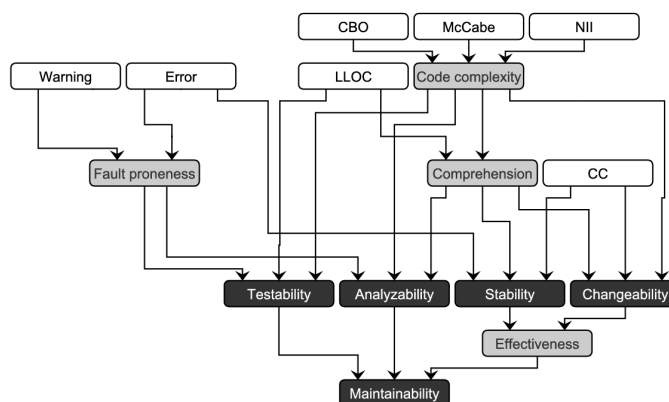
Figure 1: Java attribute dependency graph
