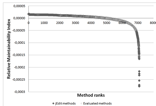
Figure 4: The relative maintainability indices and corresponding ranks
