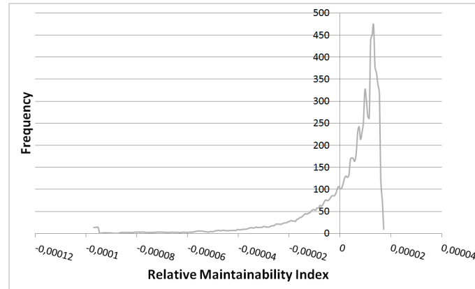
Figure 5: The density function of the relative maintainability indices
