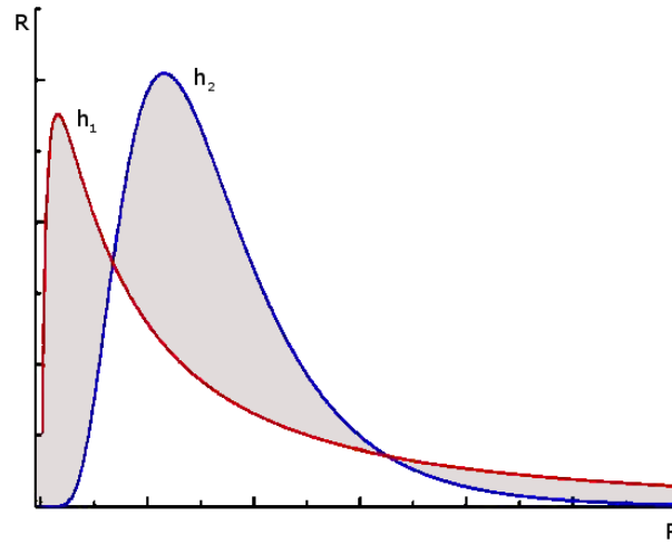
Figure 2: Comparison of probability density functions
