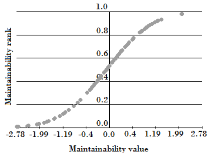
Figure 3: Benchmark characteristic for Maintainability
